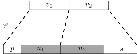
Figure 3.3: A graphical explanation of the definition of the synchronizing point.
