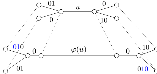
Figure 3.10: A graphiccal explanation of Example 3.3.26.
