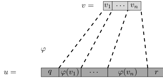
Figure 3.4: A graphical explanation of Definition 3.2.1.
