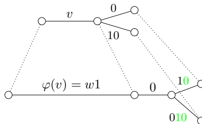
Figure 3.5: A graphiccal explanation of Example 3.2.3.
