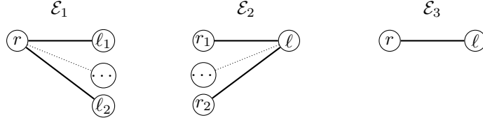
Figure 4.3: Extension graphs of non bispecial words.
