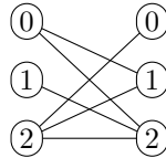
Figure 2.1: The extension graph of \mathcal{E}(\varepsilon) .
