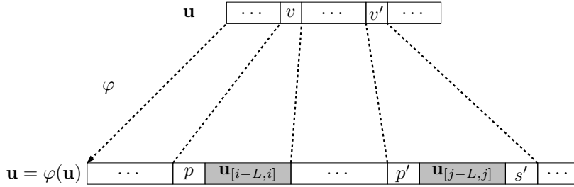
Figure 3.8: Occurrences i - L and j - L of u \in \mathcal{L}(\mathbf{u}) from the proof of Proposition 3.3.13.
