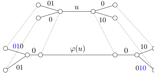
Figure 3.10: A graphical explanation of Example 3.3.26.
