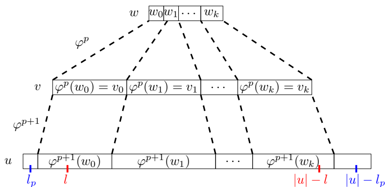
Figure 3.13: A graphical explanation of the proof of Theorem 3.4.1.
