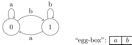
Figure 5.7: Automaton that generates the monoid M = \{\varepsilon, a, b\} .
