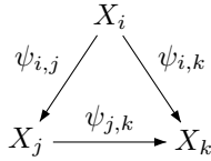
Figure 5.1: Projective system.
