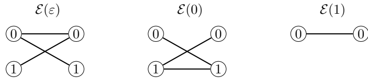
Figure 4.1: The graphs \mathcal{E}(\varepsilon) , \mathcal{E}(0) and \mathcal{E}(1) for the language \mathcal{L}(\mathbf{u}) .
