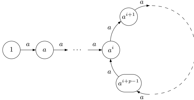
Figure 5.2: The monoid \in M_{i,p} .
