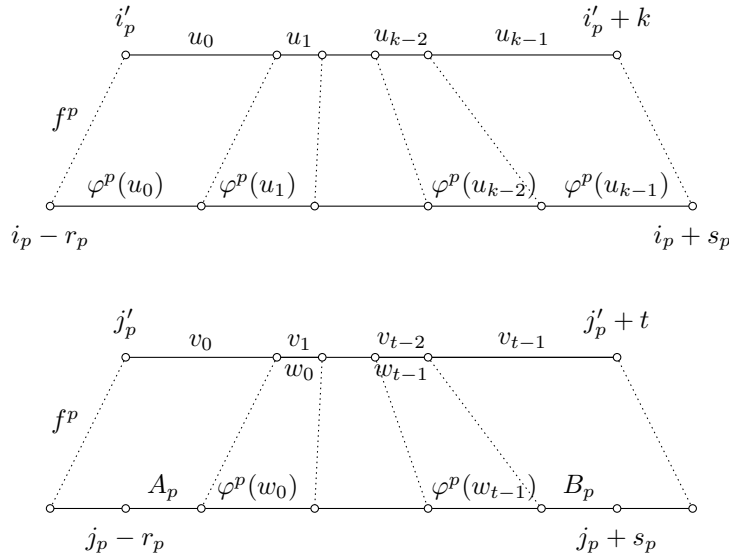
Figure 3.11: Decomposition of \varphi^p(\mathbf{u}) .
