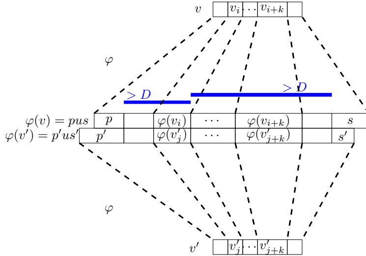
Figure 3.18: A graphical illustration of Definition 3.6.12.
