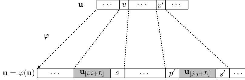
Figure 3.7: Occurrences i and j of u \in \mathcal{L}(\mathbf{u}) from the proof of Proposition 3.3.4.
