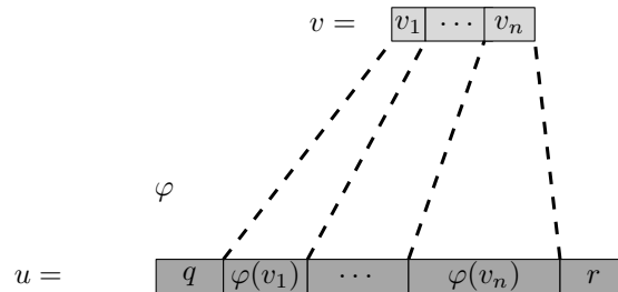
Figure 3.4: A graphical explanation of Definition 3.2.1.
