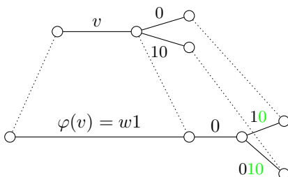
Figure 3.5: A graphical explanation of Example 3.2.3.
