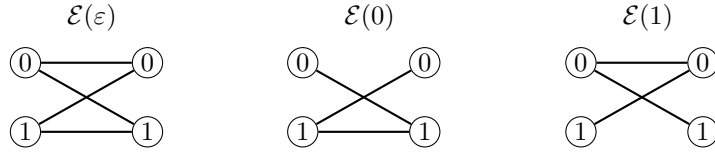
Figure 4.2: The graphs \mathcal{E}(\varepsilon) , \mathcal{E}(0) and \mathcal{E}(1) for the language \mathcal{L}(\mathbf{u}) .
