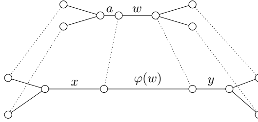
Figure 4.7: A graphical explanation of Lemma 4.3.6.
