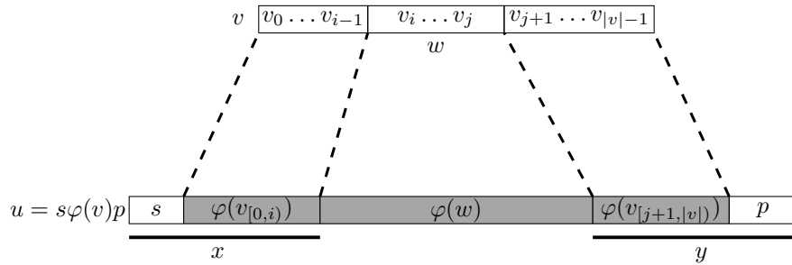
Figure 4.5: A graphical explanation of the definition of the antecedent.
