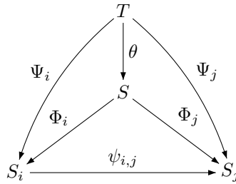
Figure 5.3: The projective limit.
