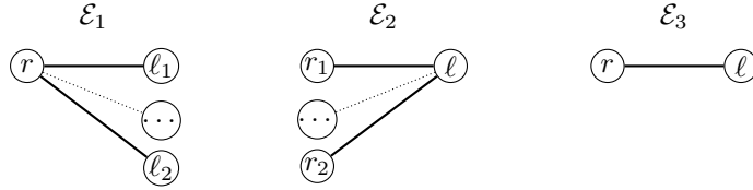
Figure 4.3: Extension graphs of non bispecial words.
