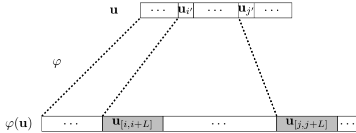
Figure 3.6: A graphical illustration of Definition 3.3.2.
