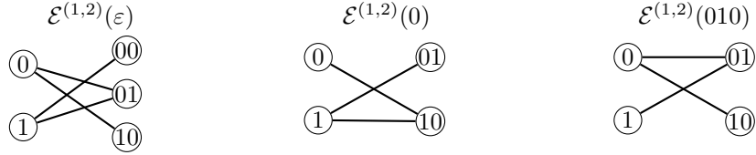
Figure 4.8: The graphs \mathcal{E}^{(1,2)}(\varepsilon) , \mathcal{E}^{(1,2)}(0) and \mathcal{E}^{(1,2)}(010) .
