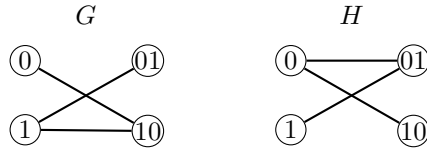
Figure 4.9: The graphs of the classes G = [\mathcal{E}^{(1,2)}(u)] (on the left) and H = [\mathcal{E}^{(1,2)}(v)] (on the right).
