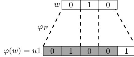
Figure 3.2: In the Fibonacci language the word w = 010 covers u = 0100 .
