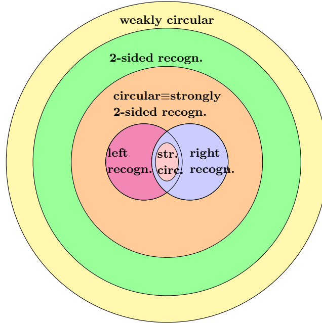
Figure 3.20: Relations between the definitions of recognizability and circularity.
