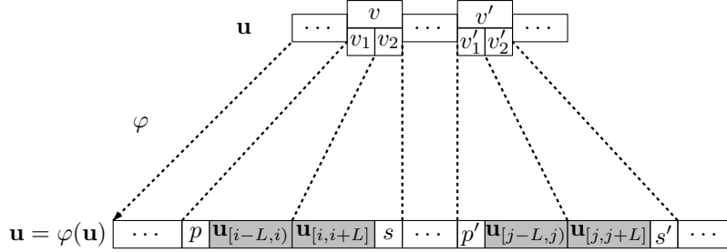
Figure 3.9: Occurrences i - L and j - L of u \in \mathcal{L}(\mathbf{u}) from the proof of Proposition 3.3.20.
