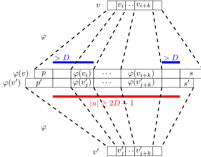
Figure 3.19: A graphical explanation of the proof of Theorem 3.6.25.
