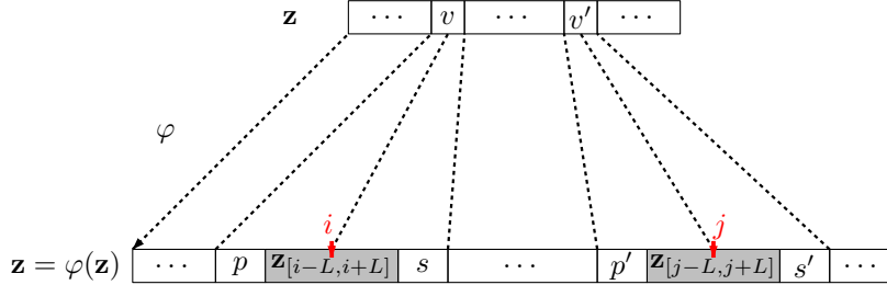
Figure 3.14: Occurrences i and j of u \in \mathcal{L}(\mathbf{u}) from the proof of Proposition 3.3.4.
