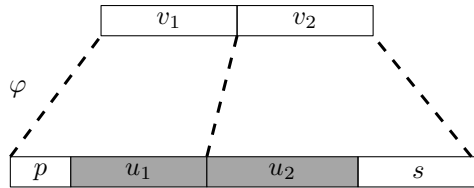
Figure 3.3: A graphical explanation of the definition of the synchronizing point.
