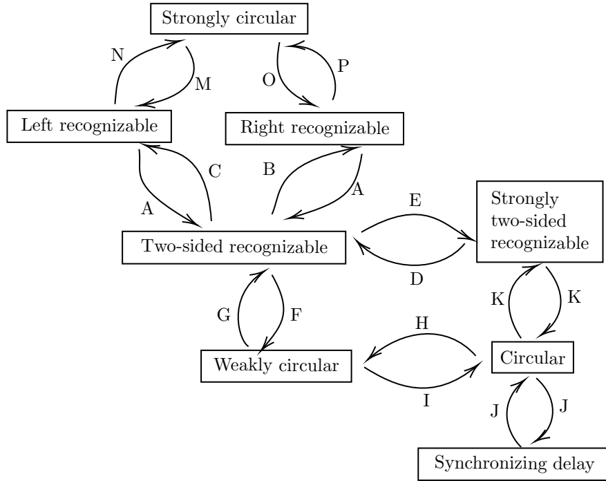
Figure 3.23: Relations between the definitions for an aperiodic morphism.
