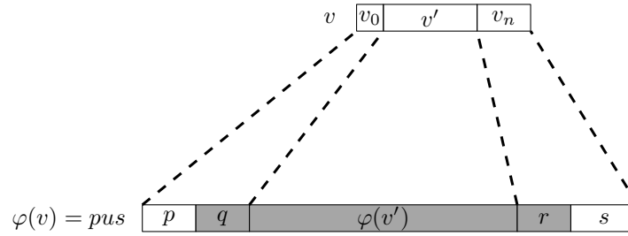
Figure 3.1: A graphical explanation of the definitions of external and internal interpretation.
