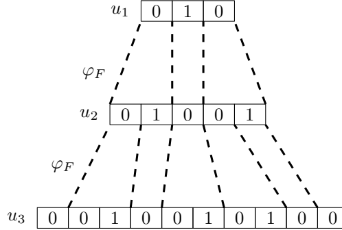
Figure 4.6: The sequence of antecedents of the word u_3 = 0010010100 in the Fibonacci language.
