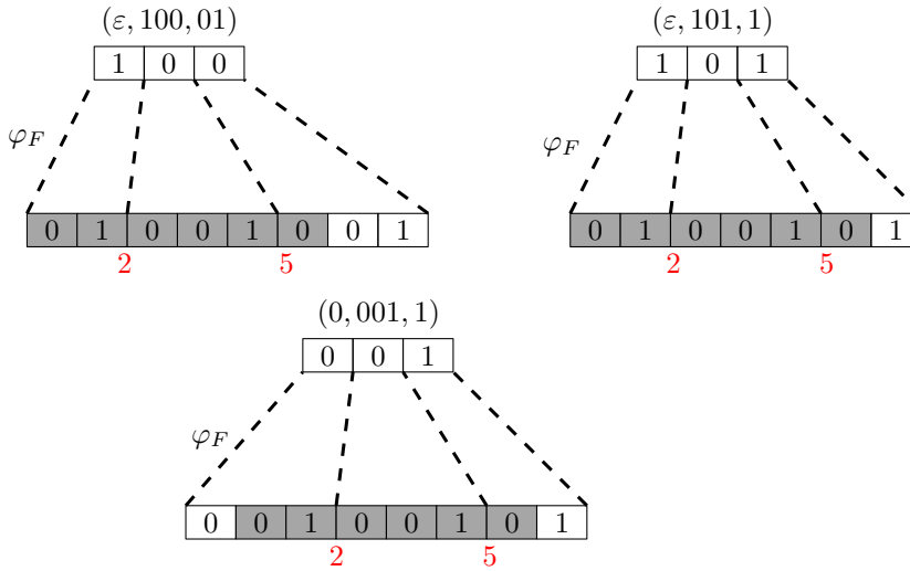
Figure 3.17: External interpretations of u = 010010 synchronized at positions 2 and 5 of u .
