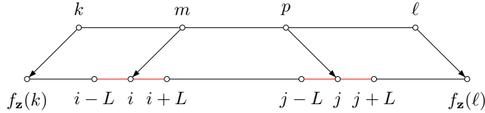
Figure 3.15: Locating k, m, p, \ell .
