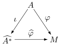
Figure 5.4: The universal property of \widehat{A^*} .
