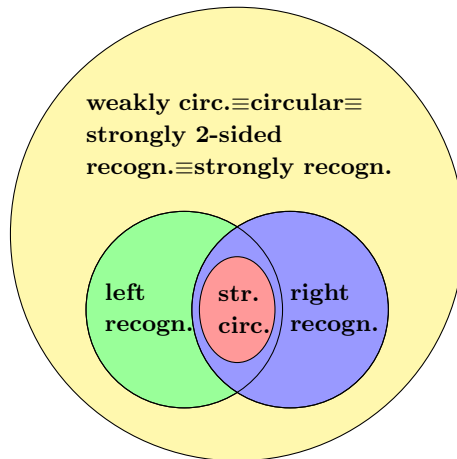
Figure 3.22: Relations between the definitions of recognizability and circularity for the primitive case.
