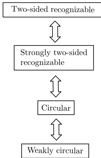
Figure 3.21: Relations between the definitions of recognizability and circularity for the case of primitive and aperiodic morphisms.
