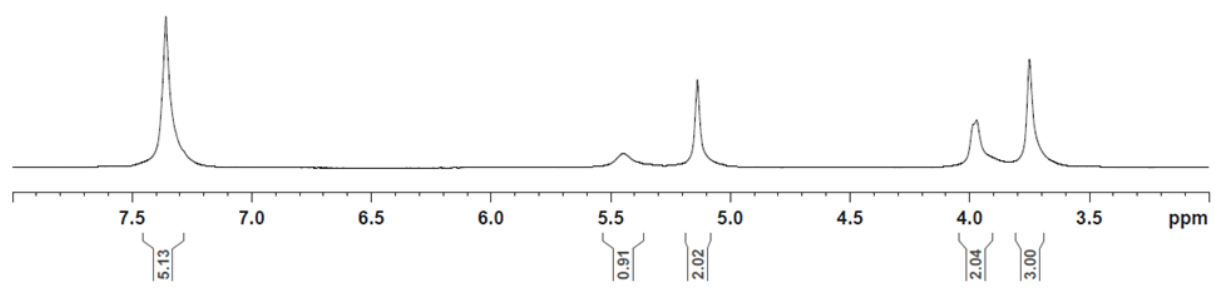
1 H-NMR HIE reaction 18b
