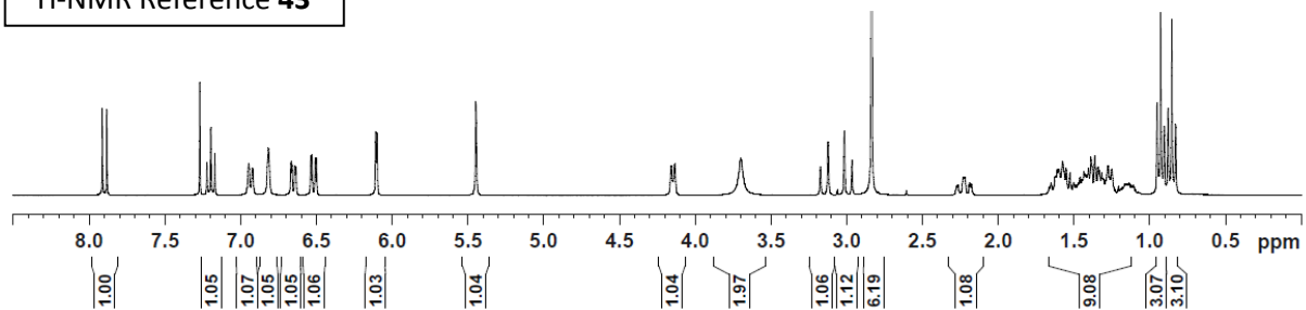
1 H-NMR Reference 43
