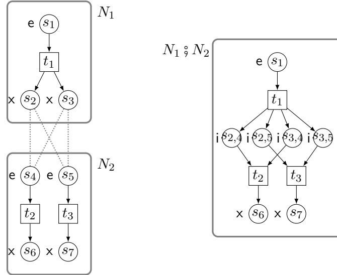
Figure 1.8. On the left: two Petri nets with control flow N_1, N_2 . On the right: the result of the gluing phase of the sequential composition N_1 \circ N_2 . Place names are indicated inside places. Dotted lines indicate how control flow places are paired by the Cartesian product during the gluing phase. Notice that, because no named place is present, the right net is exactly N_1 \circ N_2 .
