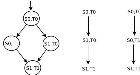
Figure 1.14. Interleavings and execution sequences of the two processes in 1.13 (see Figure [130])
