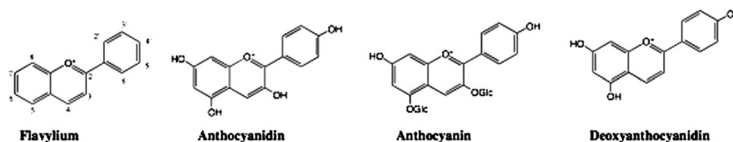
Scheme 1 Network of reversible chemical reactions of 4'-hydroxyflavylium.
