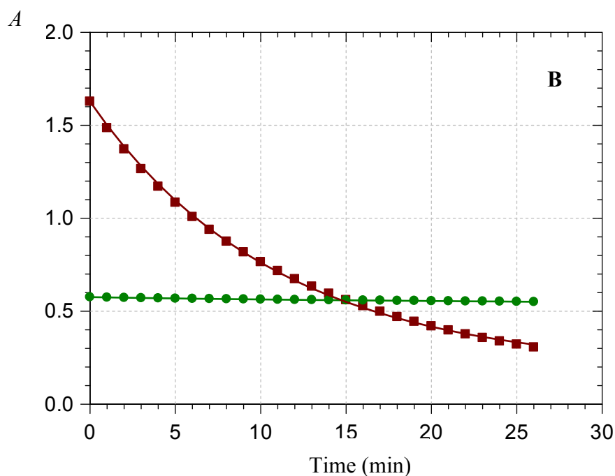
Fig. 1. A: UV-visible spectra (pigment concentration = 50 \mu\text{M} ). a) Quinonoid bases (pH 7.4 phosphate buffer, 25°C): P3 (—) and P5 (—) immediately after dilution in the buffer, P3 (---) and P5 (---) after 30 min. b) Flavylium ions (0.1 M HCl, 25°C): P3 (—), P5 (---). B: decay of the visible absorbance of the bases at \lambda_{\text{max}} . P3 (■, detection at 505 nm), P5 (●, detection at 485 nm). Solid lines result from curve-fitting assuming apparent first-order kinetics: k_{\text{obs}}(\text{P3}) = 15.4 (\pm 0.2) \times 10^{-4} \text{ s}^{-1} , k_{\text{obs}}(\text{P5}) = 19.4 (\pm 0.2) \times 10^{-6} \text{ s}^{-1} , r = 0.9998 .
