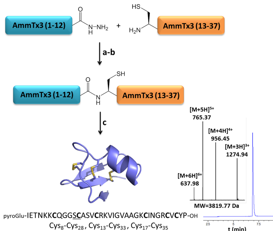
Scheme 1. Synthesis of AmmTx3 using NCL of two peptide segments. a) AmmTx3(1–12) activation: Gn-HCl (6 M), sodium phosphate (0.2 M, pH 3.0), NaNO 2 (10 equiv.), –15 °C; b) Ligation: AmmTx3(13–37), MPAA (100 equiv.), pH 6.5, room temperature; c) Folding and disulfide formation: Tris (0.2 M, pH 8.2). Analytical RP-HPLC ( \lambda = 214 nm) and ES-MS for the final purified AmmTx3 toxin were performed. Observed mass 3819.77 Da vs calculated mass 3819.87 Da. MPAA = 4-Mercaptophenylacetic acid; Tris = Tris(hydroxymethyl)aminomethane.
