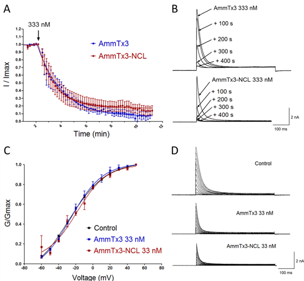
Fig. 4. AmmTx3-NCL and AmmTx3 (produced by SPPS) equally block K_v4.2 channels. A) Average time course of K_v4.2 channel outward current block recorded at 70 mV following addition of either 333 nM AmmTx3 (blue trace, n = 6 ) or AmmTx3-NCL (red trace, n = 9 ). Error bars are SEM. B) Current traces from representative cells for K_v4.2 channel block recorded at different time points (100 s, 200 s, 300 s and 400 s) following addition of AmmTx3 (top) or AmmTx3-NCL (bottom). C) K_v4.2 activation curve (conductance-voltage relation G/G_{max} ) fitted with Boltzmann functions for control currents (black trace, n = 81 ), and following addition of 33 nM AmmTx3 (blue trace, n = 7 ) or AmmTx3-NCL (red trace, n = 2 ). Error bars are SEM. D) Representative traces in response to voltage clamp activation protocol recorded for control currents (top) and in the presence of 33 nM AmmTx3 (middle) or AmmTx3-NCL (bottom).
