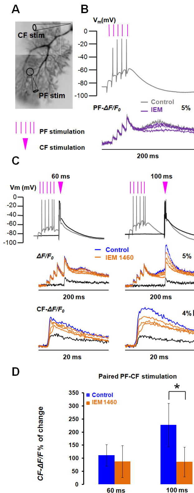
Figure 4.4.1: The effect of blocking TRPC3 channels on the physiological mGluR1-dependent supralinear \text{Ca}^{2+} signals
