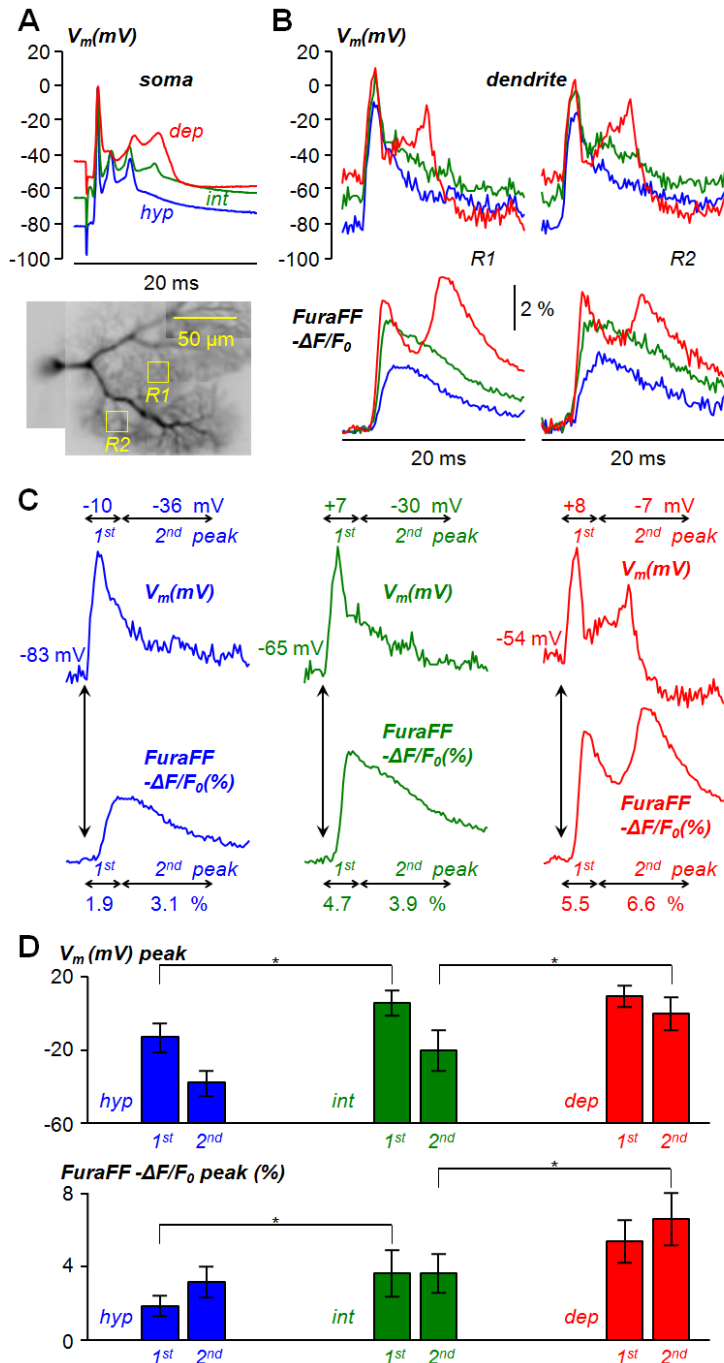
Figure 3.1.2: Combined V_m and Ca^{2+} transients associated with the CF-EPSP at different initial V_m .
