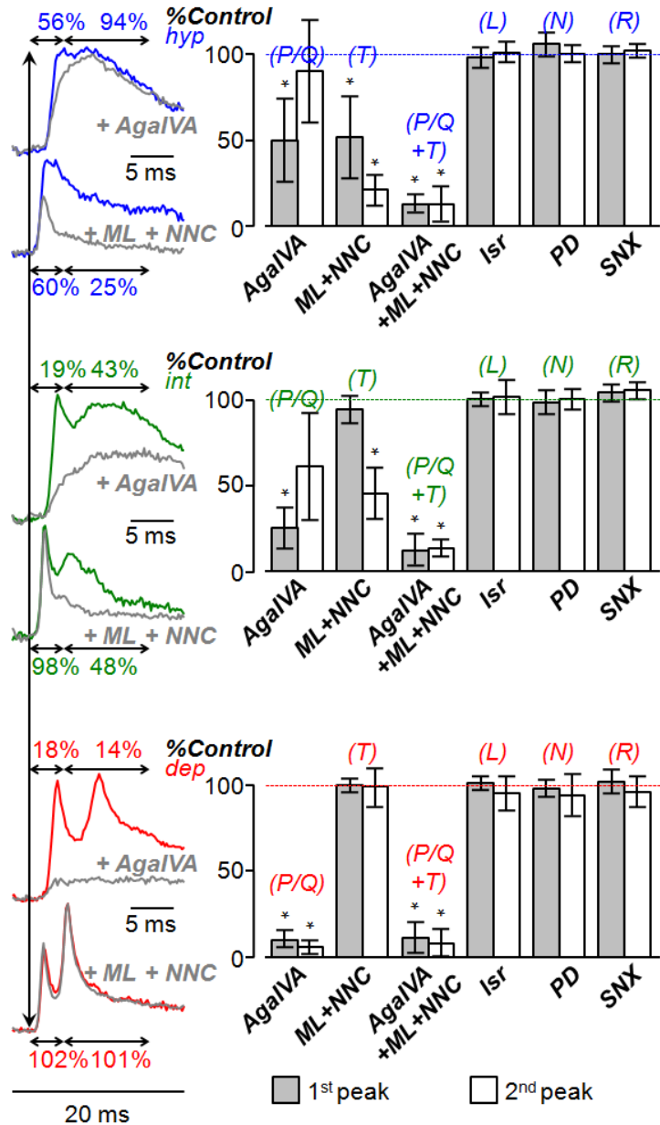
Figure 3.2.2: \text{Ca}^{2+} channels activated by the CF-EPSP at different initial V_m state.
