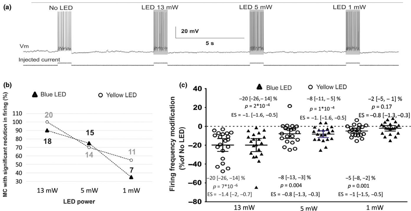
FIGURE 1 The reduction in the evoked mitral cells (MC) firing by LED stimulation depends on light power but not wavelength. (a) Representative example of LED effect on evoked MC firing. (b) Cell-by-cell analysis depicting the number and the percentage of neurons for which the LED stimulation (blue or yellow light) produce a significant ( p < 0.05 ) reduction in MC firing, compared with no-LED condition. (c) Population analysis of the effect of blue and yellow LED stimulation on MC firing. Horizontal lines represent average. Error bars represent 95% CI. Gray bars in A depict the time of LED stimulation. n = 20 MC. ES: Effect Size
