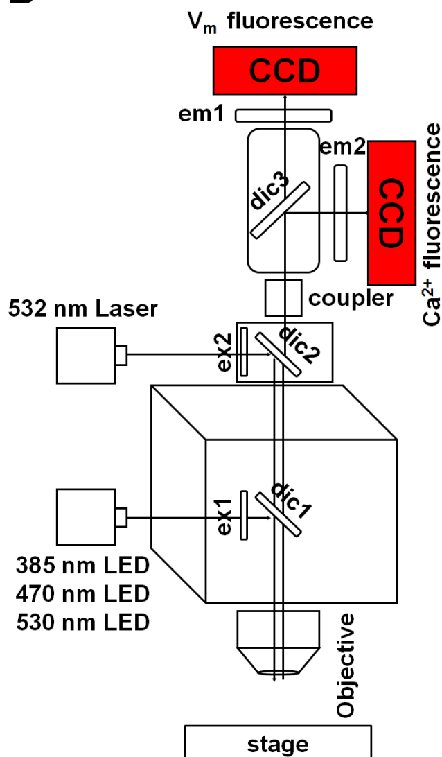
Figure 2.A. The dual NeuroCCD camera manufactured by RedshirtImaging for this type of measurement. B. Schematic drawing of the apparatus for sequential voltage and \text{Ca}^{2+} imaging using the VSD JPW1114 and the \text{Ca}^{2+} indicator FuraFF or for \text{Ca}^{2+} imaging only using OG5N; Light from a 385 nm or a 470 nm LED via the epifluorescence port of a commercial microscope is reflected by a 495 nm long-pass dichroic mirror (dic1); 532 nm laser light via the top of the microscope is reflected by a 560 nm dichroic mirror. (dic2); fluorescence images are demagnified and separated by a 565 nm long-pass dichroic mirror (dic3); The V_m image and the \text{Ca}^{2+} images are filtered by a 610 nm long-pass (em1) and by a 510\pm 42 nm band-pass filter (em2) respectively, then acquired by two CCD cameras.
