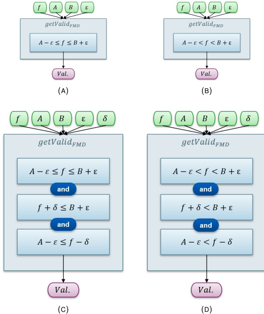
FIGURE 4.8 – Pixel validation (A) (resp. C) and its alternate version (B) (resp. D) in the classic case (resp. in the cyclic case without any rotation).
