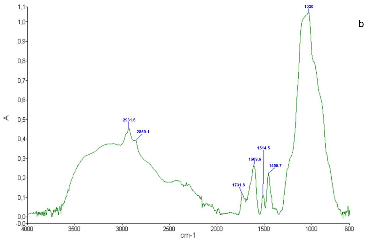
Figure 6 FTIR analysis spectra of tannins extracted from K. ivorensis sapwood (a) and heartwood (b).
