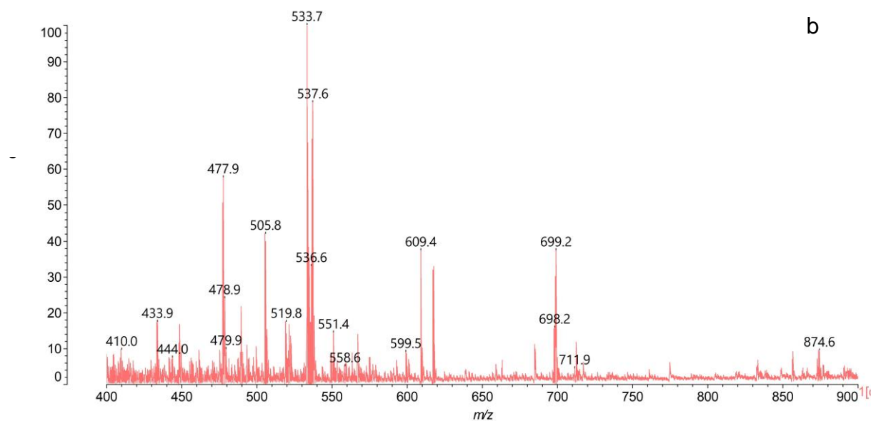
Figure 4 MALDI-TOF spectrum of tannin extracts from K. ivorensis sapwood (a) and heartwood (b) in the range 400-900 Da.
