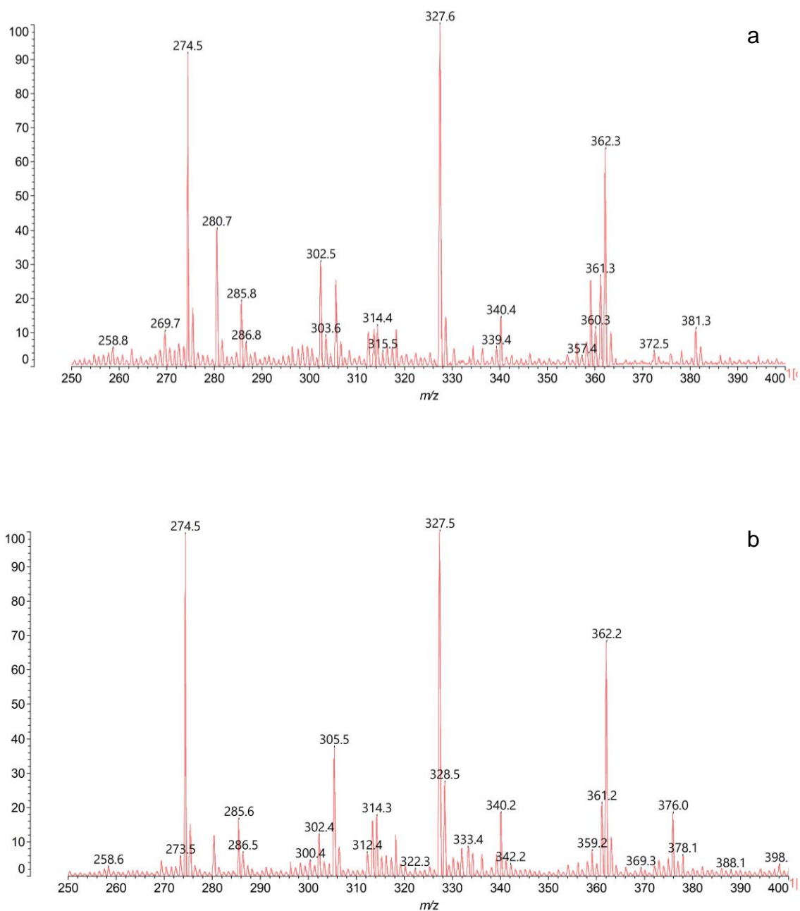
Figure 2 MALDI-TOF spectrum of tannin extracts from K. ivorensis sapwood (a) and heartwood (b) in the range 250-400 Da
