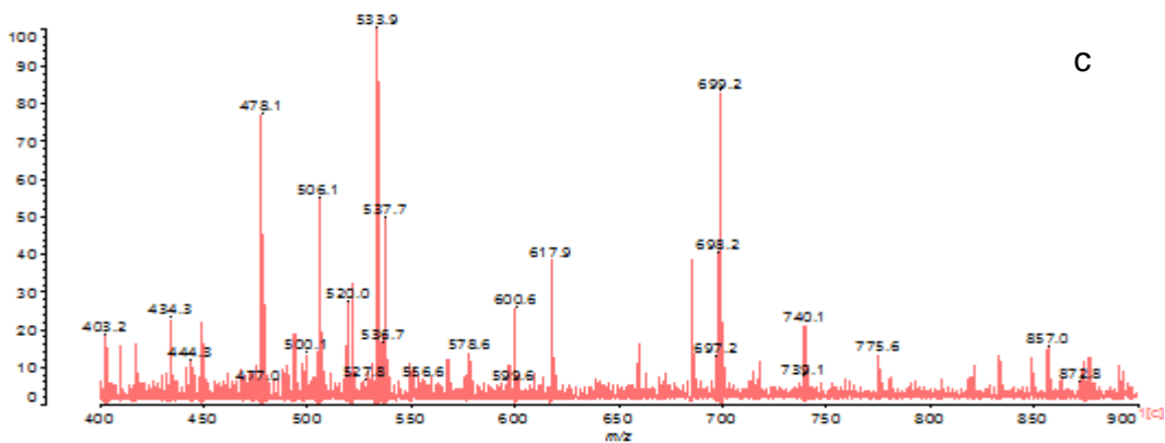
Fig. 3: MALDI-TOF spectrum of tannin extracts from K. ivorensis bark in the range 250-400 Da (a); 300-600 Da (b) and 400-900 Da (c).
