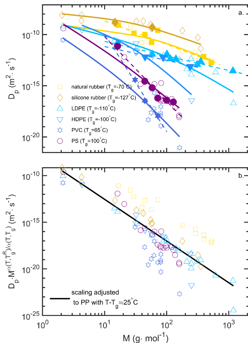
Figure II-19. Diffusivities of various substances at 25°C in glassy and rubber polymers: (a) raw values, (b) normalized data to remove polymer effects (standardized to T_g value of 0°C corresponding to atactic polypropylene PP). Filled symbols correspond to n -alkanes (scaling laws D_p \propto M^{-\alpha} as dashed lines) and empty symbols to various solutes including gases and plastic additives (scaling laws D_p \propto M^{-\alpha} as continuous lines). Data from Schwöpe et al. (1990).
