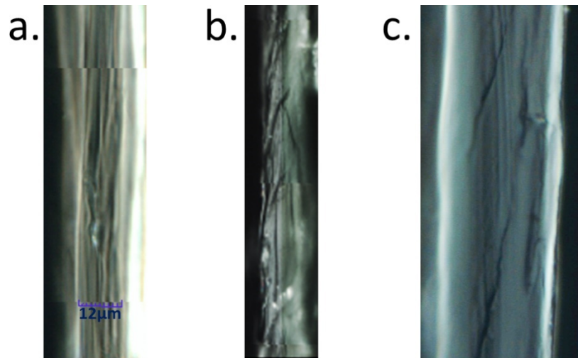
Figure V-34. Microscopic observations in phase contrast of the cross sections of 12µm-thick PET film F1. (a) neat film; (b) film immersed in water at 50°C for 10 hours; (c) film immersed in ethanol at 50°C for 10 hours.
