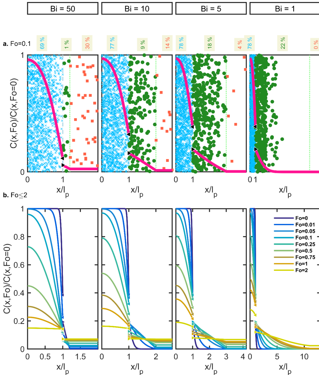
Figure II-8. One-dimensional description of solute diffusion (e.g., additive, monomer) from the packaging wall (position: 0 \leq x/l_p \leq 1 , individual solutes identified as ×) to the contacting phase (individual solutes identified as ■) via the food boundary layer (individual solutes identified as ●): (a) random distribution of solutes and corresponding concentration profile at Fo = 0.1 and (b) after contact times up to Fo = 2 . The percentages in the top part represent the residual amount in each compartment.
