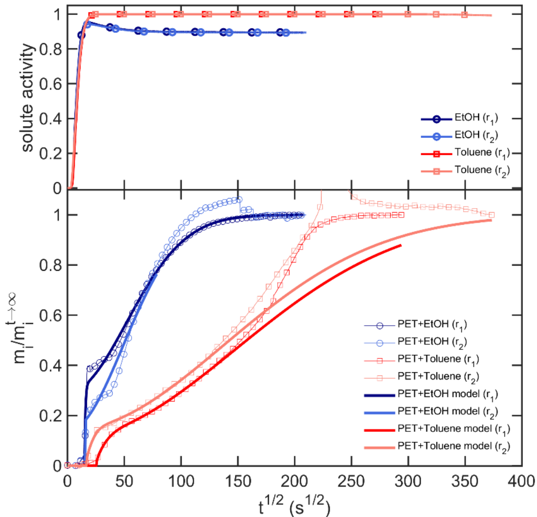
Figure V-36. Sorption kinetics of ethanol and toluene in 12 \mu\text{m} thick PET films ( F_i ) at 50°C at high activities. The fitted model is a delayed version of Eq. (V.4).
