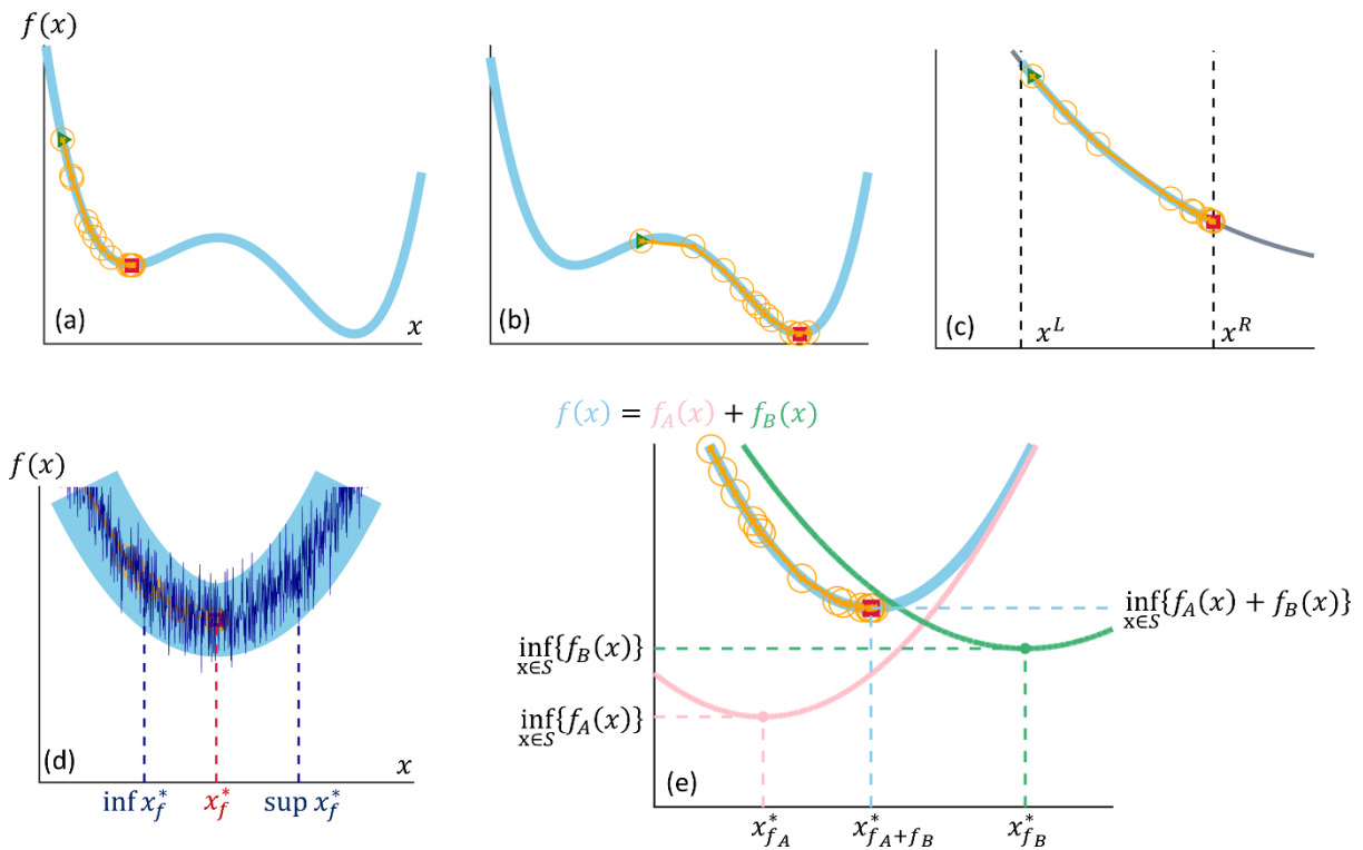
Figure II-2. (a-b,d) Illustrations of nonconvex goals; (c) convexification by adding boundaries x^L \leq x \leq x^R ; (d) nonconvex problem combining a convex problem with Gaussian white noise ( \inf x_f^* and \sup x_f^* are the bounds of the domain where the minimum can occur); (e) composition of two convex goals. The green triangle represents the initial guess and the red square the final solution of a randomized steepest descent algorithm. The intermediate positions are depicted with connected orange circles. In non-convex problems, the final solution may depend on the initial guess (see (a) and (b)).
