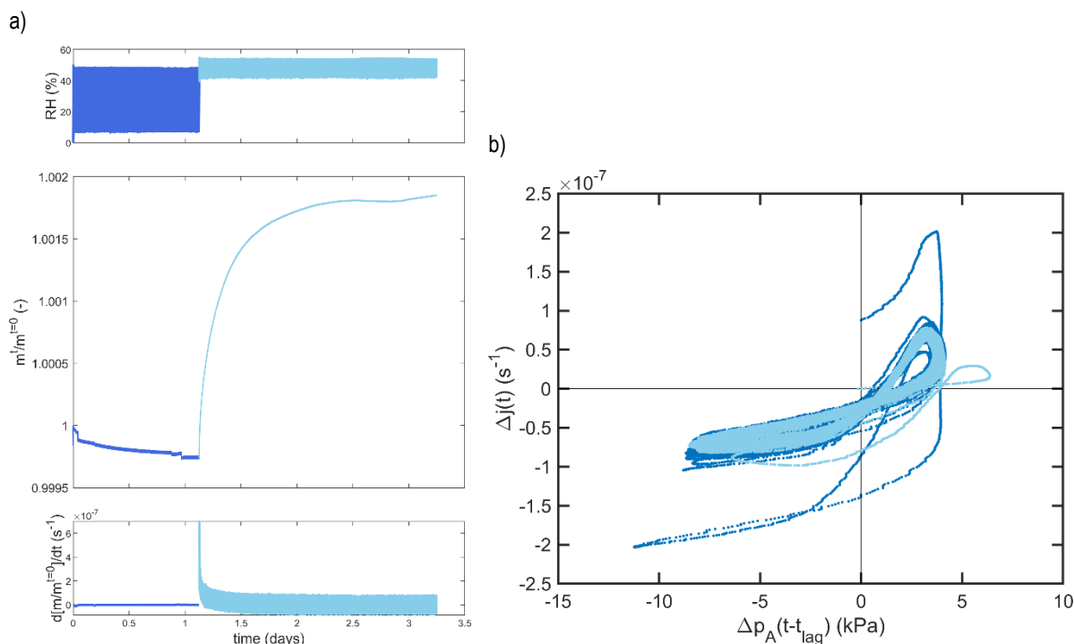
Figure V-40. Analysis of the fluctuations of mass uptake vs the fluctuations of relative humidity (period 240 s) in 12 \mu\text{m} thick PET bottle ( M ) at 50^\circ\text{C} : (a) raw results, (b) correlation between fluctuations when the average delay between has been removed.
