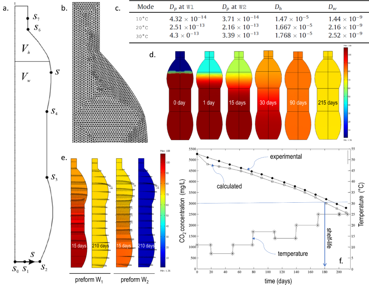
Figure II-34. Simulated \text{CO}_2 depletion in a PET bottle containing a carbonated beverage (Carrieri et al. , 2012): (a) simulated 2D wall profile along its axis of revolution; (b) details of the mesh (Lagrange quadratic); (c) diffusion coefficients of \text{CO}_2 in PET ( D_p for preforms W_1 and W_2 ), in the head-space ( D_h ) and in water ( D_w ); (d) 2D \text{CO}_2 concentration profiles in bottles ( W_1 ) quiver plot showing molar flux superimposed to concentration profiles; (e) evolution of \text{CO}_2 concentration in the bottle in variable temperature conditions.
