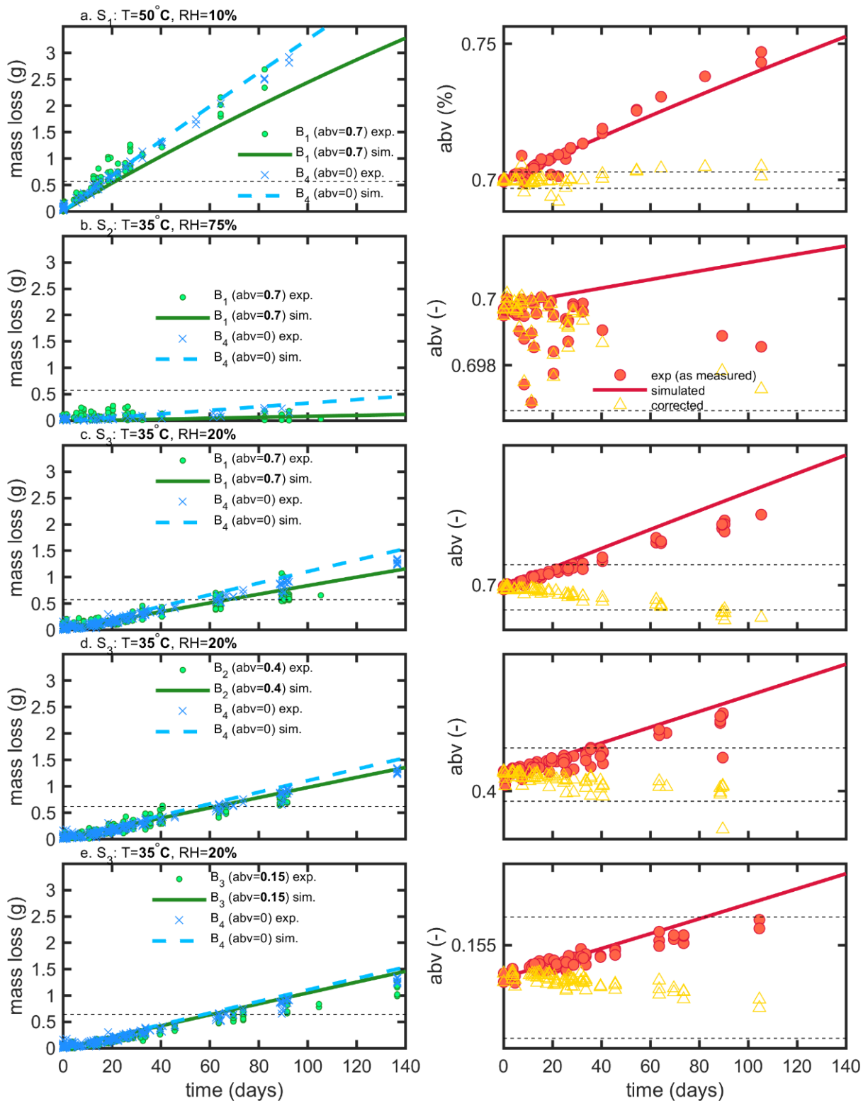
Figure V-6. Comparison of experimental ( exp ) and simulated ( sim ) mass loss and abv variations. The dashed lines plot the thresholds used to calculate shelf-life (see text). Empty symbols (triangles) represent the theoretical variation of abv when concentration effects due to water permeation are corrected.
