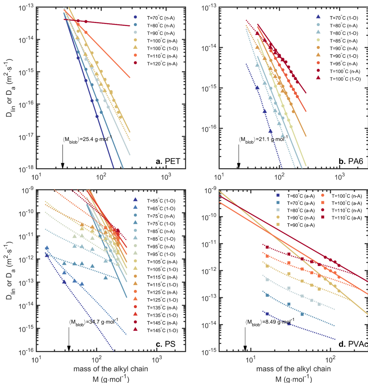
Figure V-25. Scaling of diffusion coefficients, D_{lim} or D_a , of n -alkanes ( n-A ), 1-alcohols ( 1-O ) and alkyl-acetates ( a-A ) with the molecular mass of the alkyl chain, M in: (a) PET, (b) PA6, (c) PS and (d) PVAc. Continuous and dotted lines correspond to the regression lines for regular solutes ( n -alkanes) and their generalization to anchored ones (1-alcohols and alkyl acetates) via Eq. (V.39), respectively. \langle M_{blob} \rangle was estimated the common intersection of all regression lines of \ln D_{lim} vs \ln M (see its interpretation in Eqs.(V.19) and (V.30)).
