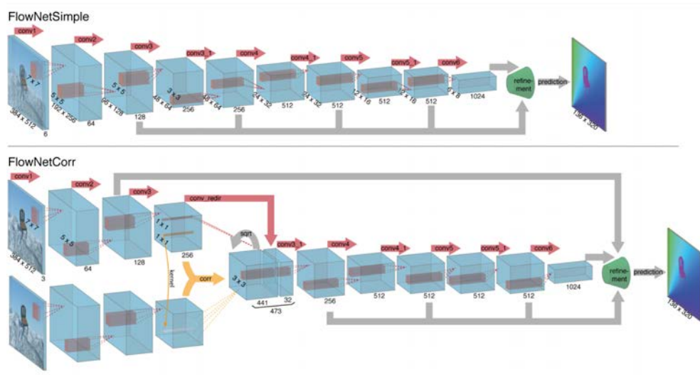
FIGURE 2.4 – FlowNetSimple (top) and FlowNetCorr (bottom), Philipp et al. (2015)
