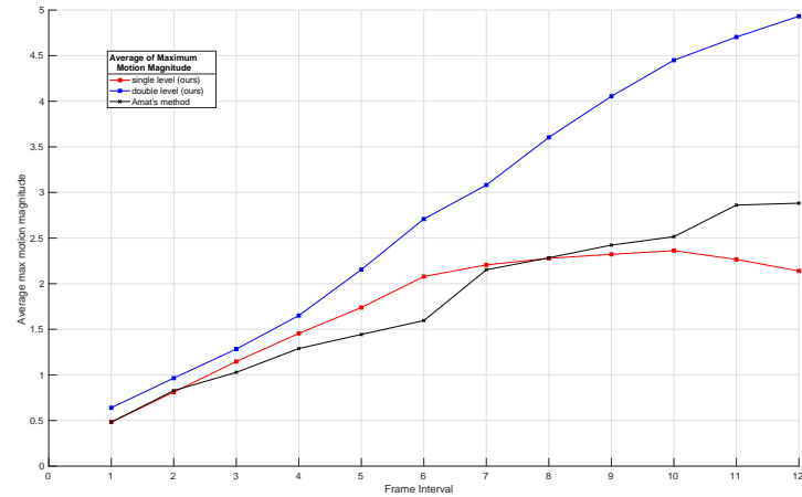
(a) Average maximum motion magnitude computed in the bleb region for pairs of volumes separated by time steps mentioned in x -axis of the plot.
