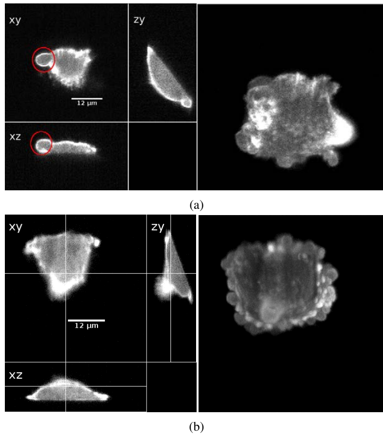
FIGURE 3.1 – Orthogonal slices (on left) and Maximum intensity projection (MIP, on right) in XY -plane of a volume in the sequence (a) MV3 A (b) MV3 B. A bleb in the cell surface of MV3 B. Several small sphere-like protrusions in the cell surface of MV3 B are the blebs.
