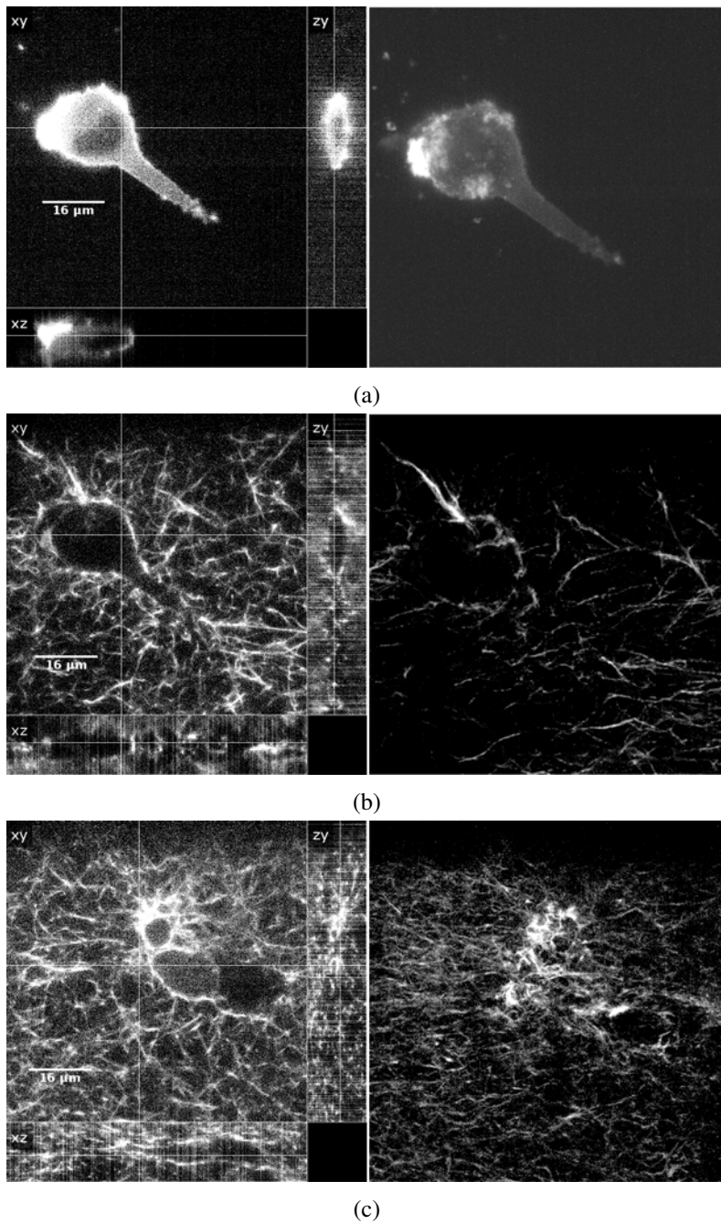
FIGURE 3.2 – Orthogonal slices (on left) and Maximum intensity projection (MIP, on right) in XY-plane of a volume in the sequence (a) MV3 C (b) Collagen 1 (c) Collagen 2.
