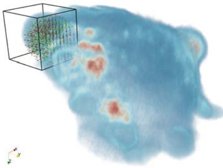
(a) Orthogonal (in red) and tangential (in green) components of the bleb region
