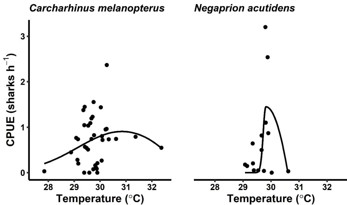
Figure 2.5 Thermal performance curves for reef shark neonate abundance around Moorea, French Polynesia. Optimal temperature for abundance for C. melanopterus was 30.85 °C and for N. acutidens was 29.82 °C. The curves intersect with the x-axis at an upper critical temperature, T_{crit} , where CPUE would be predicted to be zero ( C. melanopterus T_{crit} = 33.24 °C; N. acutidens T_{crit} = 30.60 °C). Each point represents mean CPUE and temperature during one season at individual sites for each species.
