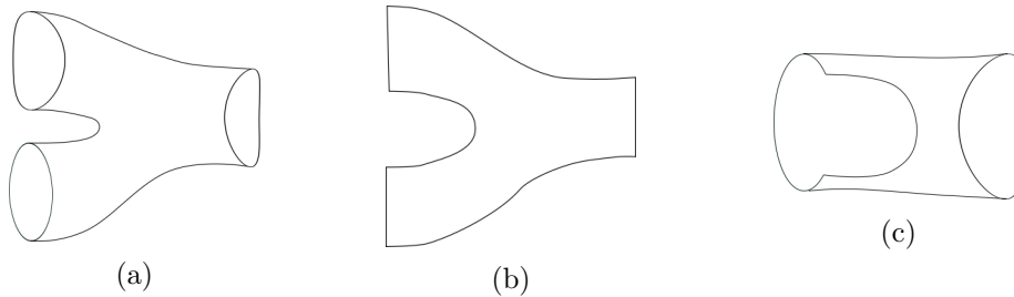
Fig. 2.2 String interactions. Closed and open strings can interact as in 2.2a and 2.2b, respectively. Open strings can also join their ends to form a closed string 2.2c.
