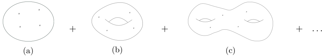
Fig. 2.3 The sum over all string worldsheets decompose into a sum over all topologies because of Weyl invariance.
