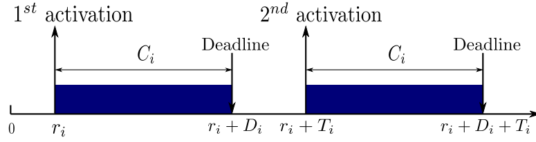
Fig. 5.2 Simplification of Liu and layland's model
