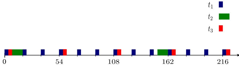
Fig. 6.16 A feasible schedule of the strictly periodic system represented in Table 6.2 and Figure 6.15. The tasks starting dates are respectively equal to s_1 = 0, s_2 = 8 and s_3 = 4 .
