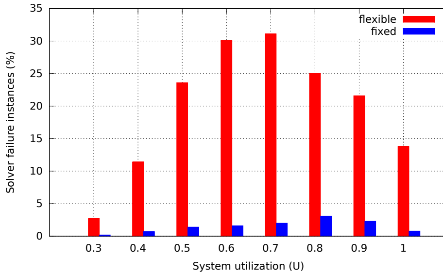
Fig. 7.8 Percentage of solver failure instances for fixed and flexible cases with respect to the system utilization. The RTSDFG size |\mathcal{T}| was fixed to 20 tasks.
