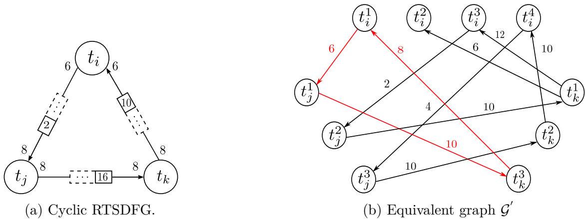
Fig. 5.14 A cyclic RTSDFG with its equivalent graph that models the precedence and dependence constraints between the tasks executions.
