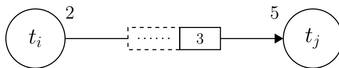
Fig. 3.3 A simple example of Synchronous Data Flow Graph.
