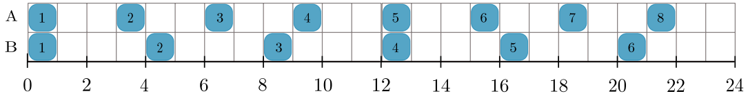
Fig. 6.4 A feasible periodic schedule of the SDFG depicted in Figure 6.3a.
