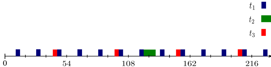
Fig. 6.20 A feasible schedule resulting from applying Algorithm 5 on the periodic system composed of t_1 = (10, 4, 14, 18) , t_2 = (120, 10, 50, 144) and t_3 = (40, 4, 14, 54) . The tasks starting dates are respectively equal to s_1 = 10 , s_2 = 122 and s_3 = 42 time units.
