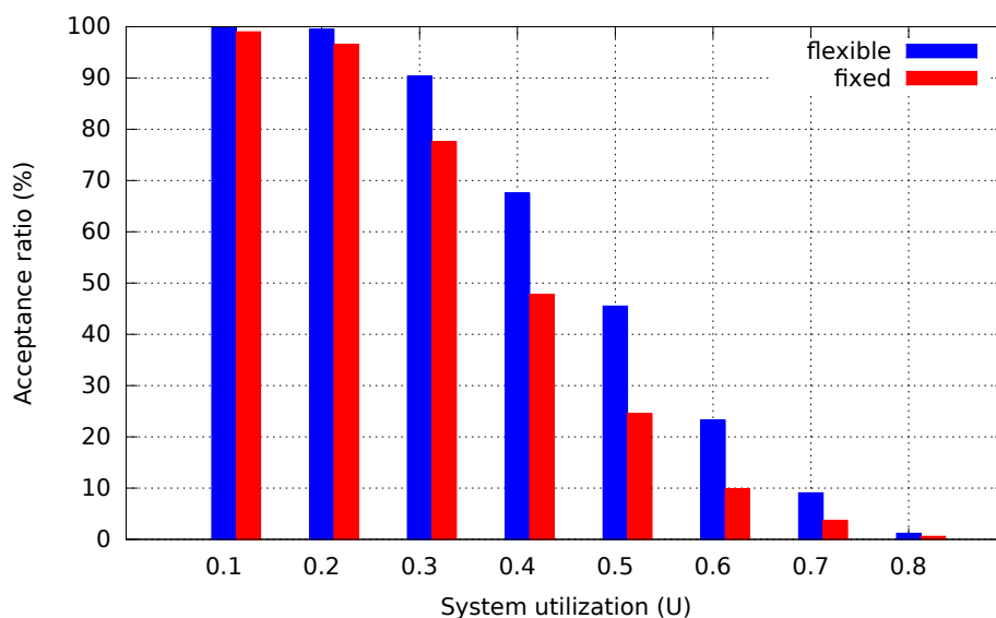
Fig. 7.18 The mega-heuristic acceptance ratio on harmonic instances with release dates. The RTSDFG size |\mathcal{T}| was fixed to 30 tasks.
