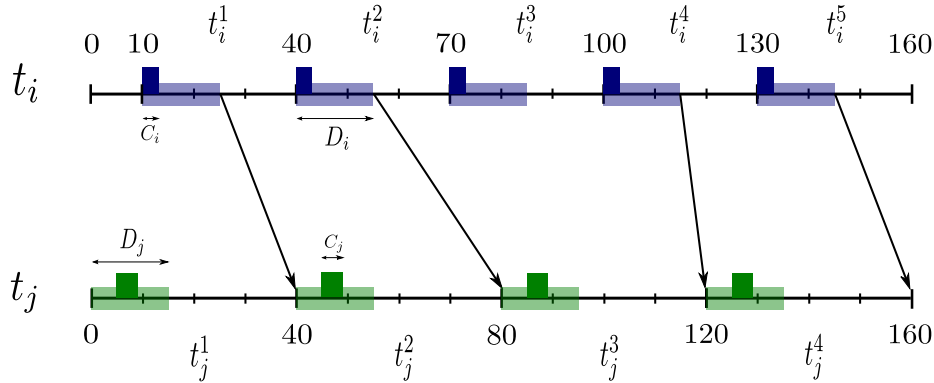
Fig. 6.5 Communications constraints between the executions of two strictly periodic tasks t_i = (10, 3, 15, 30) and t_j = (0, 4, 15, 40) .
