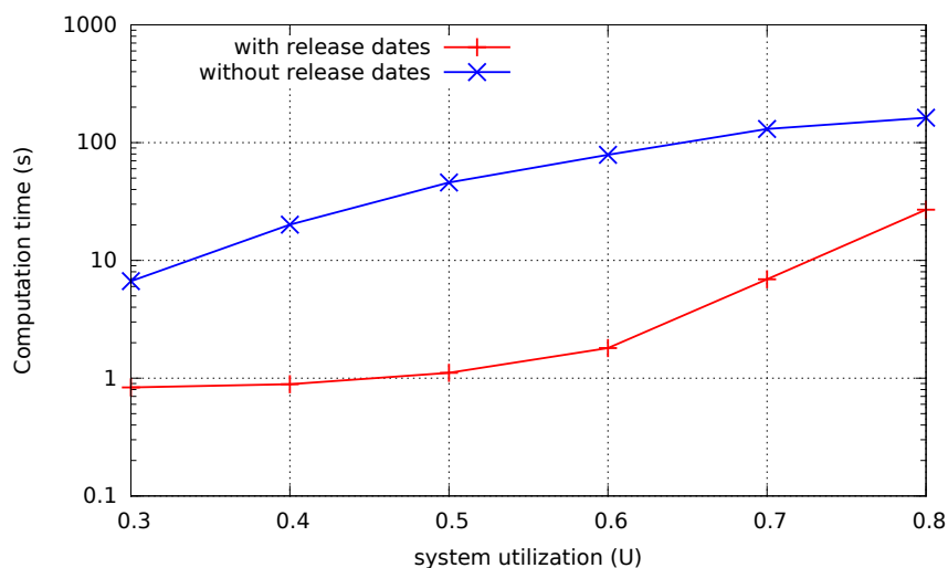
(b) Average computation time to find a feasible solution.
