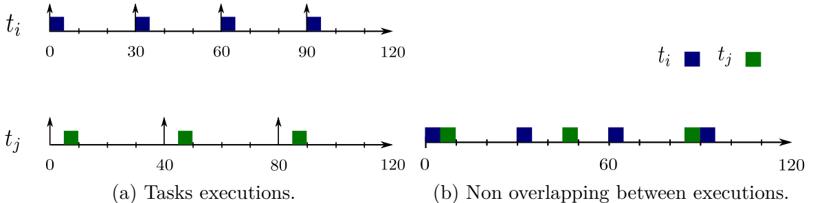
Fig. 6.2 Scheduling two strictly periodic tasks t_i = (0, 5, 30) and t_j = (5, 5, 40) on the same processor.
