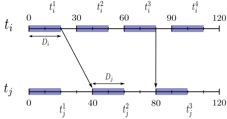
Fig. 5.3 Example of multi-periodic communication model
