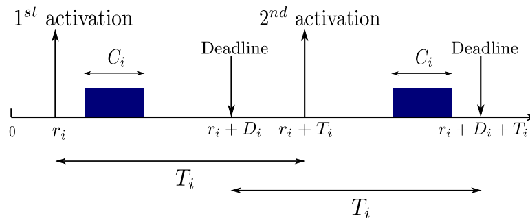
Fig. 5.1 Liu and Layland model
