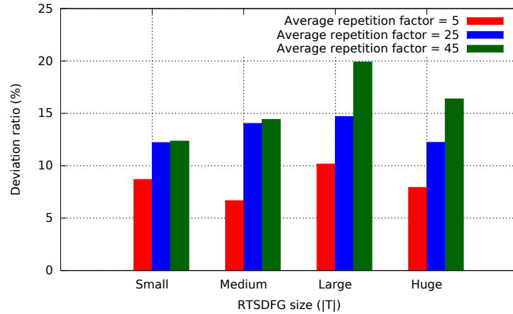
(a) Upper bound.
