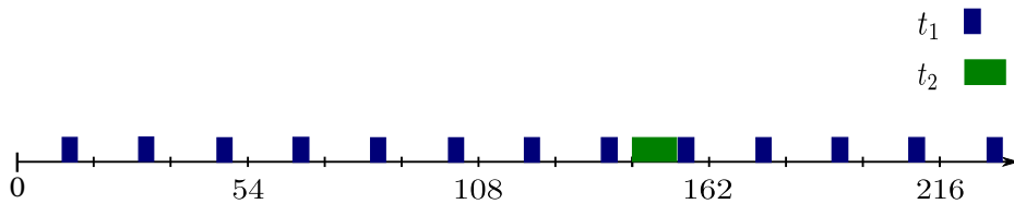
Fig. 6.19 Scheduling task t_2 = (120, 10, 50, 144) such that the end of its execution corresponds to the beginning of task t_1 = (10, 4, 10, 18) which is already scheduled with a starting date s_1 = 10 time units.
