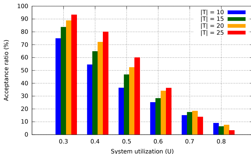
(a) MILP acceptance ratio (%).
