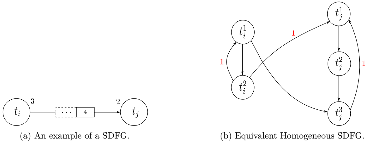
Fig. 3.8 Example of SDFG transformation into equivalent HSDFG using the expansion .
