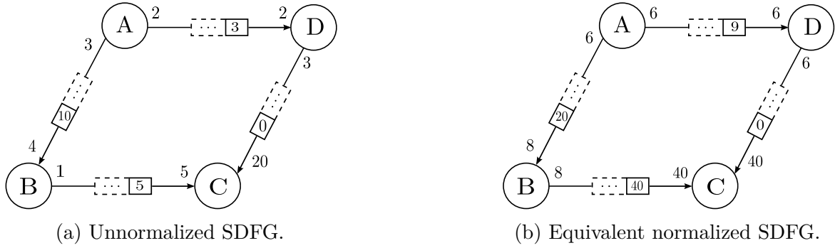
Fig. 3.6 Example of Synchronous Data Flow Graph normalisation .
