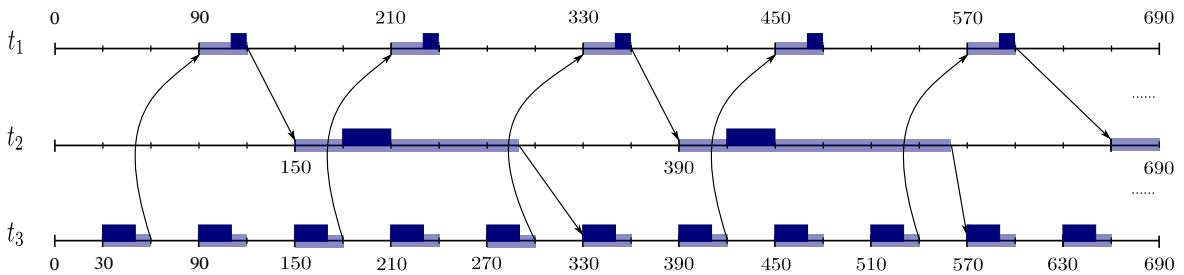
Fig. 6.8 A feasible Schedule of a strictly periodic system with communication constraints.
