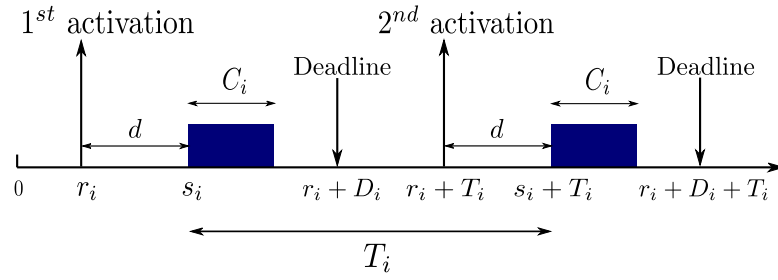
Fig. 6.1 Non-preemptive strictly periodic task.
