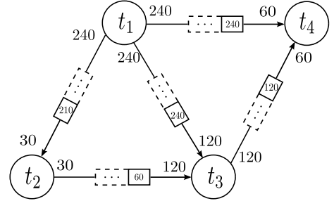
Fig. 6.21 RTSDFG \mathcal{G} = (\mathcal{T}, \mathcal{A}) .
