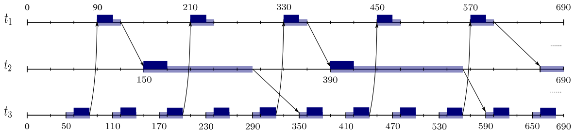
Fig. 6.10 A feasible schedule of the example depicted in Figure 6.9. Communication constraints are respected and there is no overlapping between the tasks executions.
