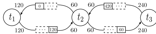
Fig. 6.11 RTSDFG \mathcal{G} = (\mathcal{T}, \mathcal{A}) modeling the communication constraints between the executions of t_1 = (110, 10, 25, 120) , t_2 = (15, 15, 30, 60) and t_3 = (190, 45, 200, 240) .
