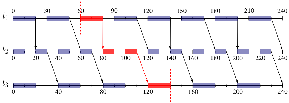
Fig. 5.10 Communication and execution model of the path pth = \{t_1, t_2, t_3\} depicted in Figure 5.9.
