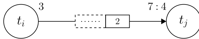
Fig. 3.2 Example of Computation Graph.
