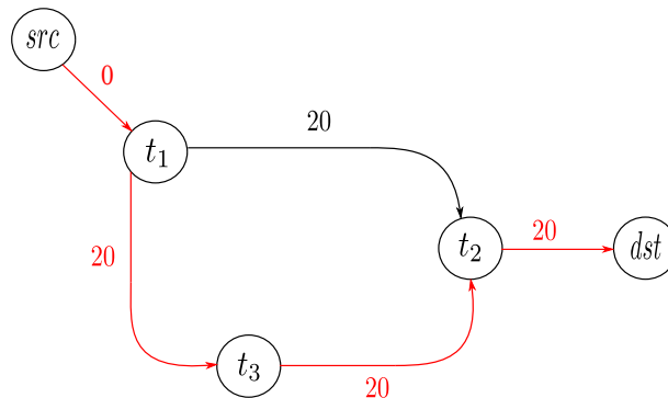
Fig. 5.16 Latency lower bound computation of the RTSDFG depicted in Figure 5.15a using the weighted graph \mathcal{G}_{min} .
