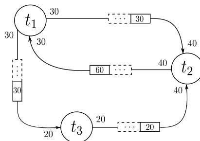
Fig. 5.7 The RTSDFG that models the communications between the tasks' executions of the multi-periodic system presented in Table 5.1 and Figure 5.6
