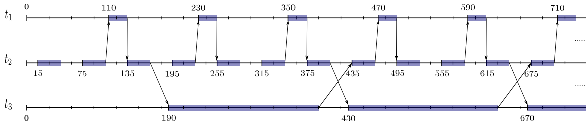
Fig. 6.12 Communication scheme between the executions of t_1 = (110, 10, 25, 120) , t_2 = (15, 15, 30, 60) and t_3 = (190, 45, 200, 240) .
