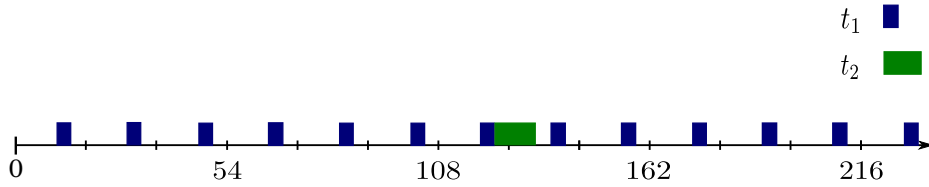
Fig. 6.18 Scheduling task t_2 = (120, 10, 50, 144) at the end of the execution of task t_1 = (10, 4, 10, 18) which is already scheduled with a starting date s_1 = 10 time units.
