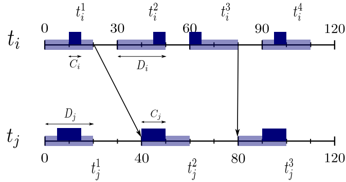
Fig. 5.5 An example of scheduling which respects the communication constraints between the tasks t_i = (0, 5, 20, 30) and t_j = (0, 10, 20, 40) .
