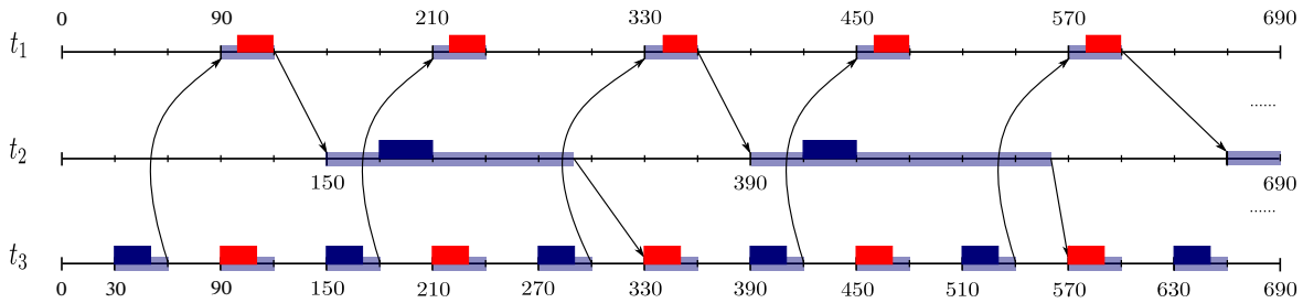
Fig. 6.9 Example of an infeasible solution where the resource constraints are not fulfilled. There is an overlapping between the executions of t_1 and that of t_3 .
