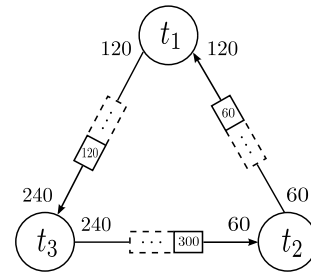
Fig. 6.7 RTSDFG \mathcal{G} = (\mathcal{T}, \mathcal{A}) .
