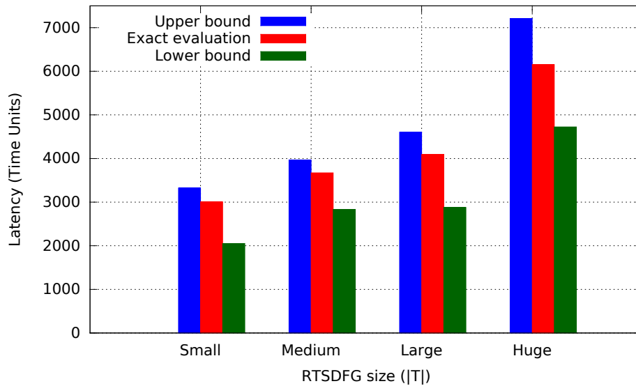
Fig. 7.1 Average latency value using the evaluation methods with respect to the graph size |\mathcal{T}| . The average repetition was fixed to 125.
