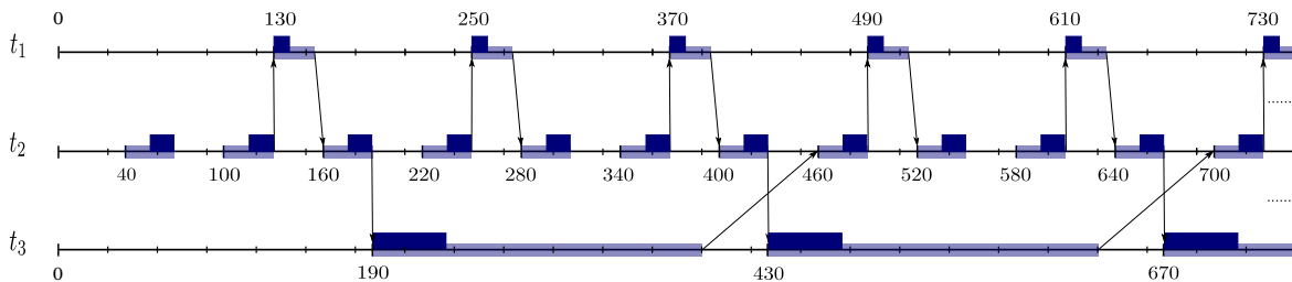
Fig. 6.13 Scheduling the strictly periodic communicating tasks t_1 = (110, 10, 25, 120) , t_2 = (15, 15, 30, 60) and t_3 = (190, 45, 200, 240) on the same processor.
