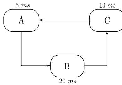
Fig. 2.4 Example of a harmonic multi-periodic system. The tasks periods are equal T_A = 5\text{ ms} , T_B = 20\text{ ms} and T_C = 10\text{ ms} .
