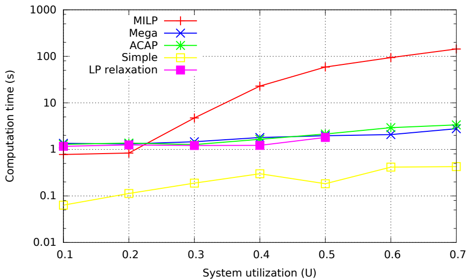
Fig. 7.16 Average computation time to find a feasible solution. MILP represents our exact method while Mega, ACAP, simple and LP relaxation represent our heuristics.
