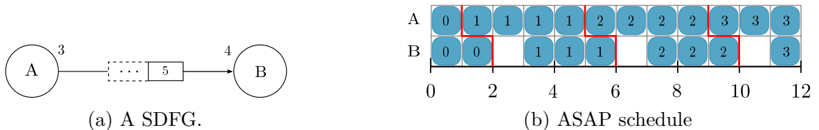
Fig. 6.3 Example of a SDFG and its ASAP schedule.
