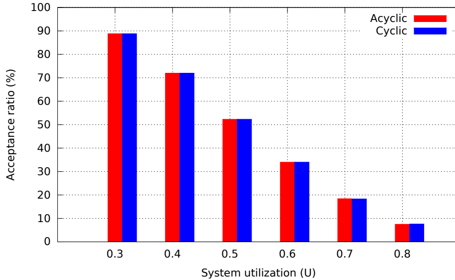
Fig. 7.6 MILP acceptance ratio on harmonic acyclic and cyclic instances with respect to the system utilization. The graph size |\mathcal{T}| was fixed to 20 tasks.
