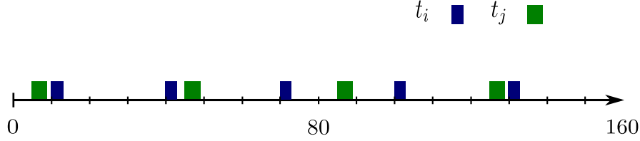
Fig. 6.6 Scheduling on the same processor the strictly periodic communicating tasks t_i = (10, 3, 15, 30) and t_j = (0, 4, 15, 40) of the example in Figure 6.5.
