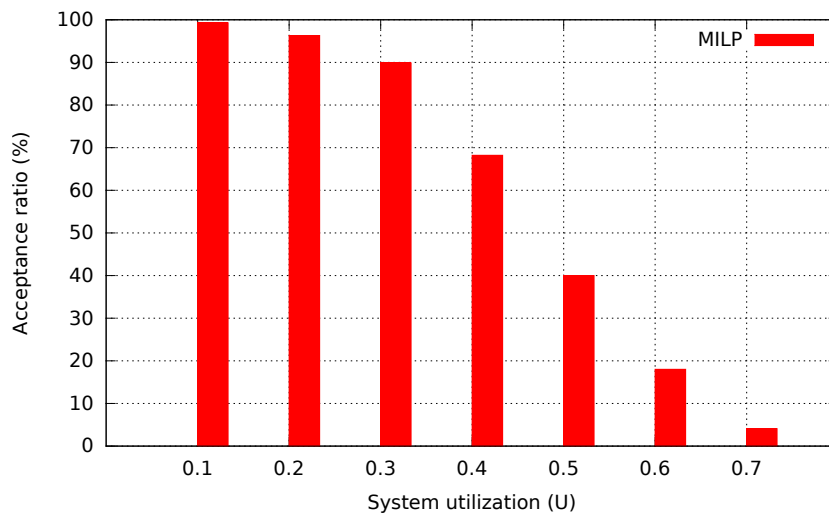
(a) MILP acceptance ratio for the fixed case.
