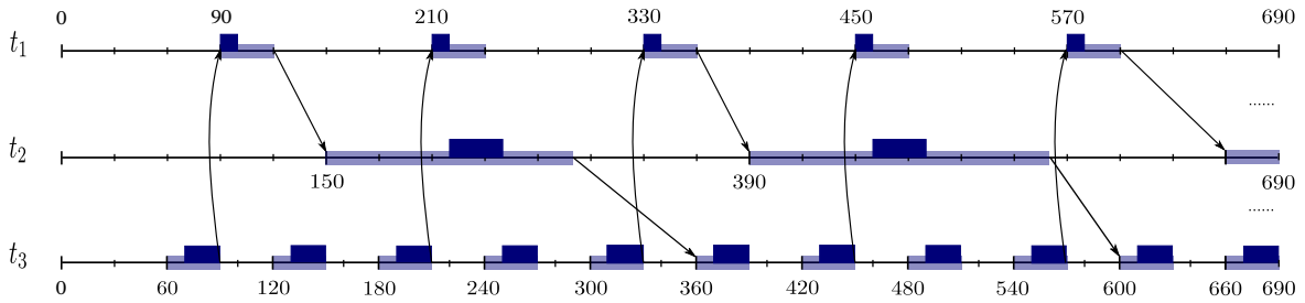
Fig. 6.14 A feasible solution for the scheduling problem is obtained by solving the new LP with k_{12} , k_{13} and k_{23} respectively equal to 1, -1 and -3 .
