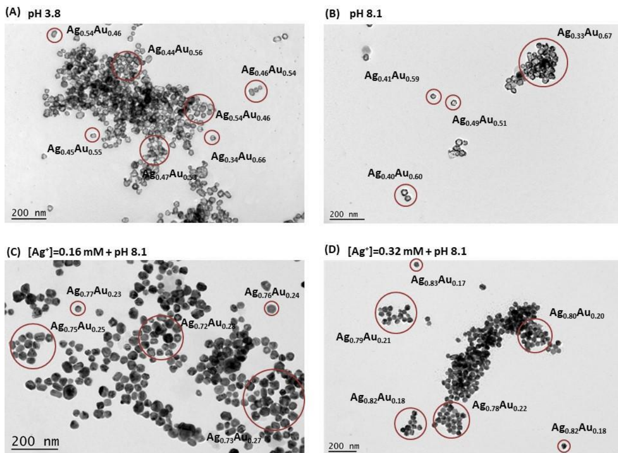
Figure S2. TEM micrographs with X-ray Energy-Dispersive Spectroscopy (X-EDS) analysis at (A) pH 3.8, (B) pH 8.1 and (C-D) after adding the silver nitrate ( [Ag^+] = 0.16 \text{ mM} and [Ag^+] = 0.32 \text{ mM} , respectively) in suspension at pH 3.8 and then, raising the pH until pH 8.1.
