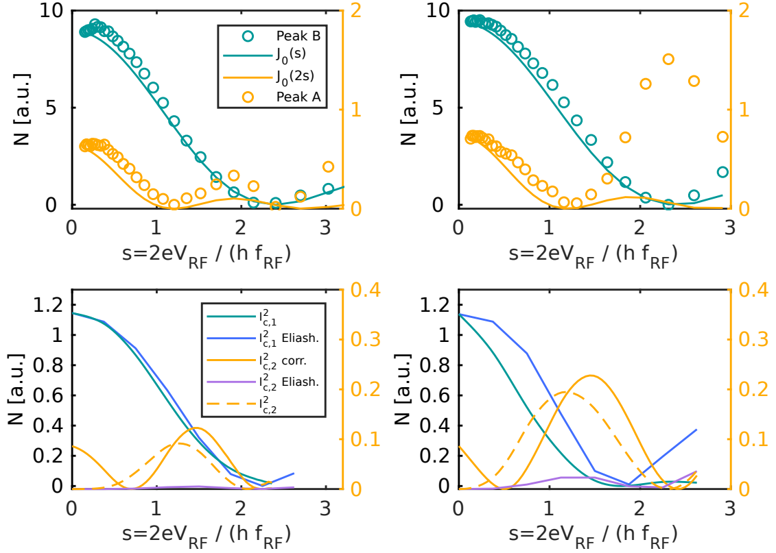
Figure 6.12: Top left: the observed amplitudes of peaks A and B as a function of microwave power at T = 1.6 K and f = 20.72 GHz. In all four panels the 2nd harmonic is shown on the right scale. The calibration of s was done such that the low power behavior of peak B follows J_0(s) . The second harmonic (peak A ) roughly follows J_0(2s)^2 . Top right: the same as top left but at f = 35.18 GHz - at high powers the second harmonic (peak A ) is significantly increased compared to A(s=0)J_0(2s)^2 . Bottom left (right): theoretical curves computed using the theory presented in chapter 5.3, with \Gamma/E_T = 0.4 , k_B T/E_T = 7 , \Delta/E_T = 55 and \hbar\omega_{RF}/E_T = 3 ( \hbar\omega_{RF}/E_T = 7 ), respectively. Within the Eliashberg approximation the second harmonic is negligible at all powers. Using the full theory the amplitude of the second harmonic is qualitatively in agreement at high s but it fails to reproduce the component at s = 0 as k_B T > E_T . Using I_{c,2} = I_{c,2}^0 J_0(2s) + I_{c,2}^{th}(s) , where I_{c,2}^0 (< 0) is a free parameter produces a good qualitative match at all values of s .
