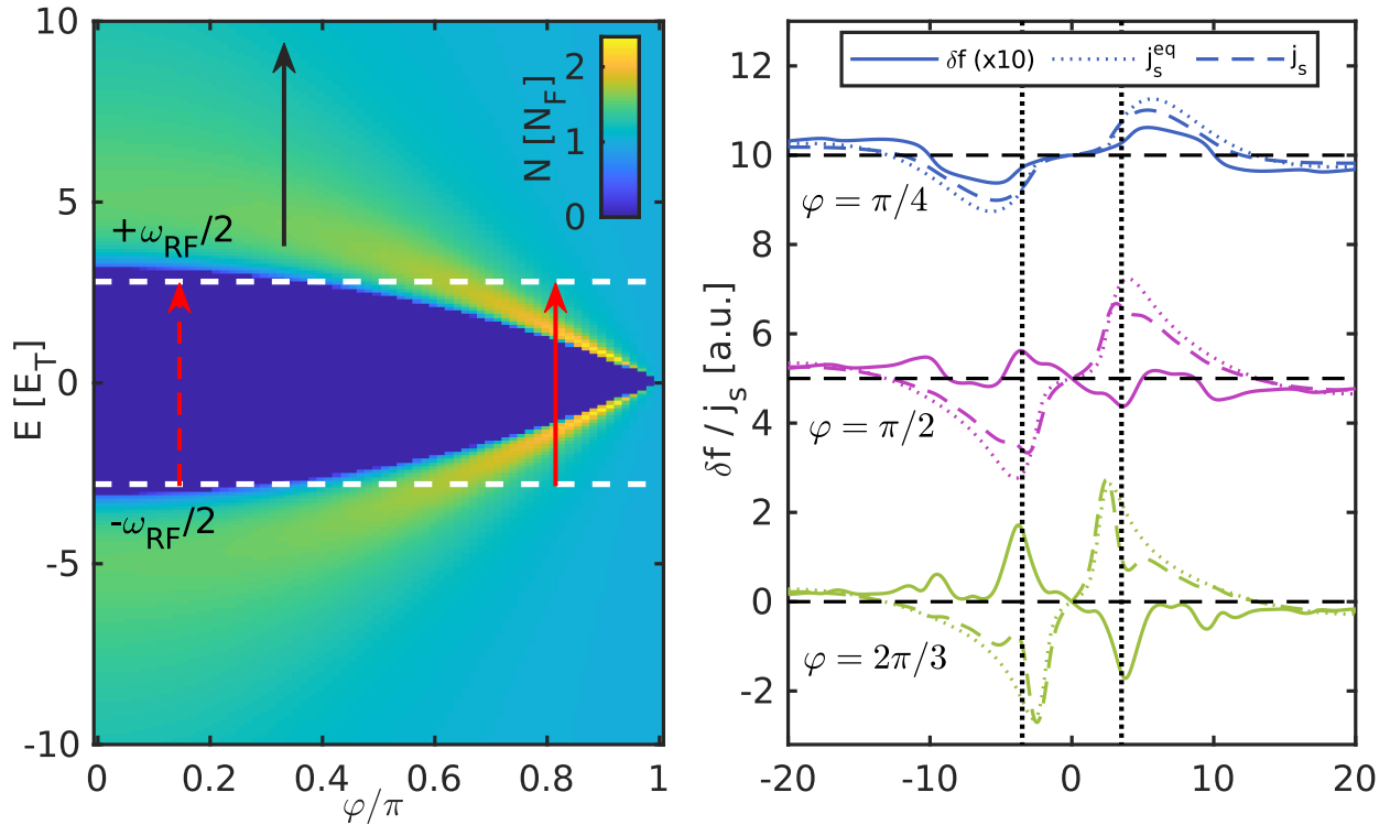
Figure 6.13: Left: a schematic of the microwave induced transitions, the white dashed lines indicate the microwave frequency, the black arrow shows the allowed intraband transition, while the (dashed) red arrows show the (dis)allowed interband transition, due to the phase dependent minigap. The induced changes to the spectral supercurrent and the distribution function, calculated using the microscopic theory, are shown on the right panel, where the dashed vertical lines indicate the microwave frequency. If the minigap is sufficiently low (i.e. if the phase is close to \pi ) there are significant changes with respect to the equilibrium values, especially at E = \pm \hbar\omega_{RF}/2 as a consequence of the absorption peak shown in 5.16. The parameters used for the calculation are the same as in figure 6.12 with \hbar\omega_{RF}/E_T = 7 .
