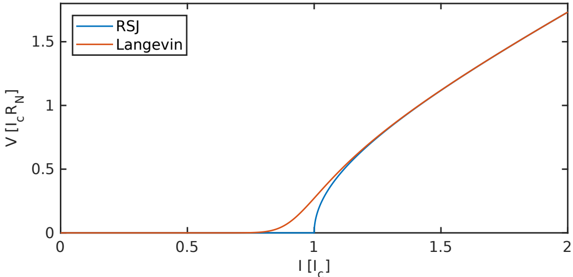
Figure 5.1: The V(I) curve of a junction based on the RSJ model without fluctuations (blue) and with a Langevin term ( \gamma = \frac{\hbar I_c}{ek_B T} = 50 , red curve).
