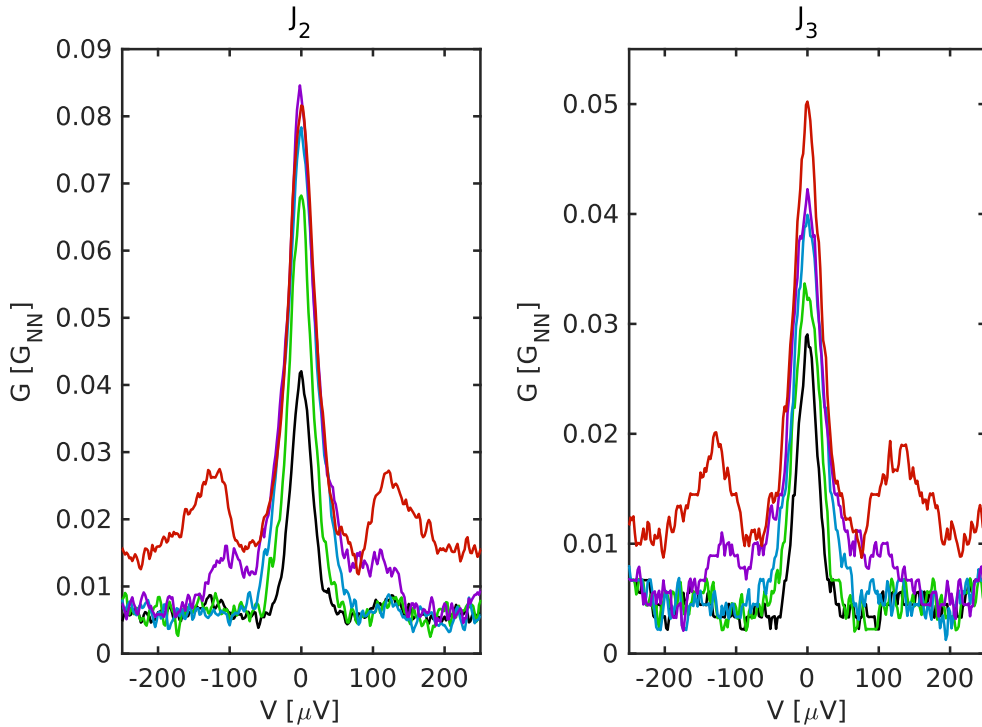
Figure 4.8: The sub-gap G(V) curve of detector J_2 (left) and detector J_3 (right) as a function of the injection current ( H = 1T ). The traces are color coded and correspond to the same injection currents as in 4.7.
