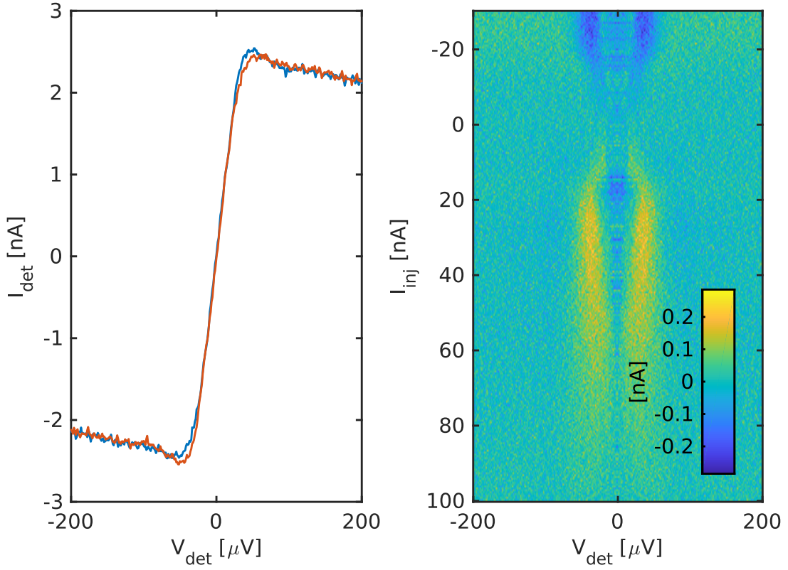
Figure 4.14: Left: an I(V) curve (blue) and -I(-V) (red, numerically obtained) from a spin-insensitive detector at H = 1.4\text{T} , T = 70\text{mK} and I_{\text{inj}} = 25\text{nA} showing an odd component localized close to the superconducting gap \Delta . Right: the (numerically obtained) odd component at the same field and temperature as a function of the injection current.
