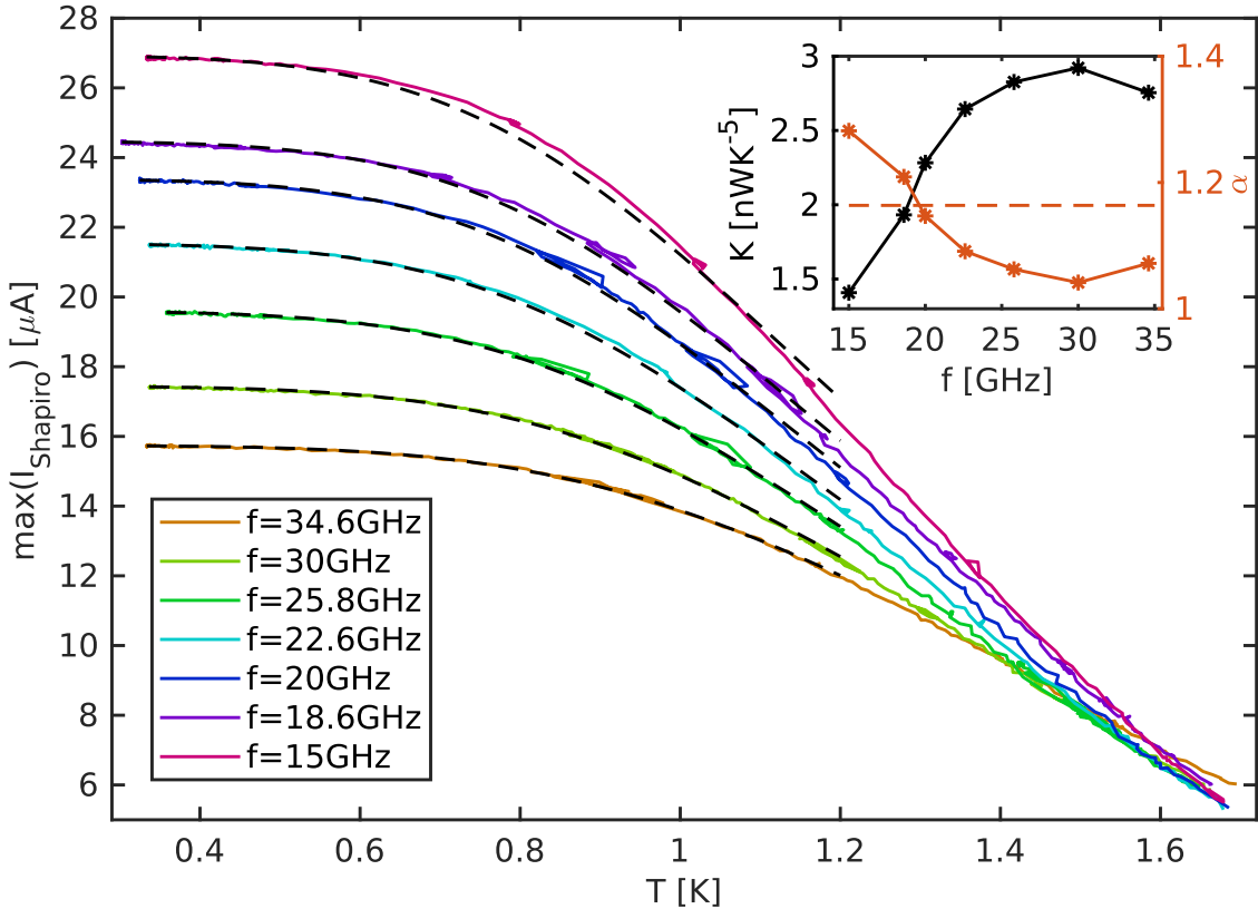
Figure 6.8: The measured temperature dependence of the maximum Shapiro step width for several frequencies (all above 2eI_cR_N\hbar^{-1} ) as a function of temperature. Due to the electron overheating the steps saturate to a frequency dependent value at low temperature. A thermal model (black dashed traces), allows for the extraction of the effective electron-phonon coupling (shown in the inset).
