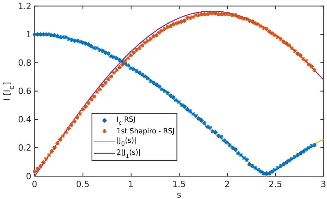
Figure 5.3: The calculated power dependence of the critical current (blue dots) and the full width of the 1st Shapiro step (red dots) from the RSJ model ( \omega_{RF} = 3\frac{2eI_cR_N}{\hbar} ) versus the power of the microwave drive s , as well as the absolute value of the first two Bessel functions.
