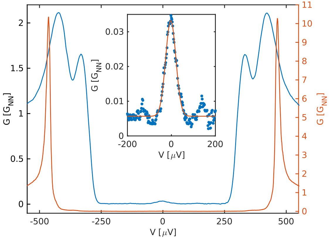
Figure 2.10: The G(V) curve of J_1 at H = 1\text{T} which shows the "splitting" of the coherence peaks at |eV_{det}| = |\Delta \pm \mu_B H + \Delta_D| , which is explained in detail in the section 2.3. The small Josephson contribution, close to V = 0 , can be modeled as a Gaussian peak and subtracted from the data, as shown in the inset. The red trace (shown on the right scale) is from a previous device with a Zeeman-split detector, also at H = 1\text{T} .
