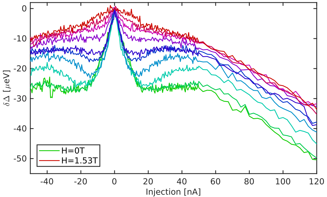
Figure 3.7: The gap suppression \delta\Delta(I_{inj}) = \Delta(I_{inj}) - \Delta_0 measured at J_1 as a function of the applied magnetic field (10 equidistant steps from H = 1.53\text{T} to H = 0\text{T} ) and the injection current.
