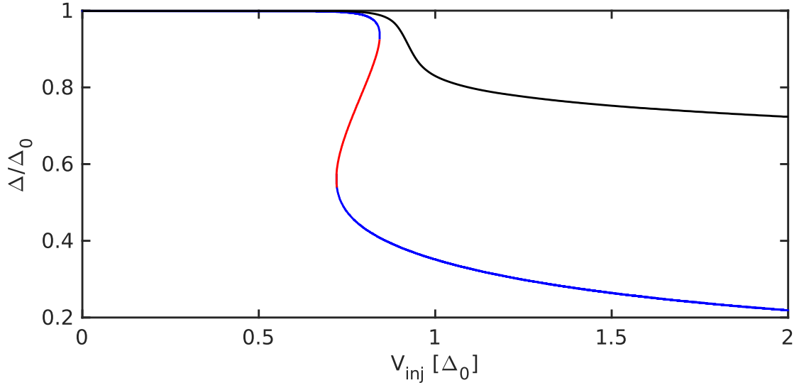
Figure 1.9: The suppression of the superconducting order parameter \Delta as a function of the voltage applied to the normal metal injector. The black curve is calculated for \frac{D_0 \bar{r}}{L} = 0.05 and it is stable everywhere. The red-blue curve is calculated for \frac{D_0 \bar{r}}{L} = 0.2 . It exhibits an S-shaped region of bistability, where the stable branches are given in blue, and the unstable one in red. The temperature of the normal metal is T = 0.05\Delta_0 which accounts for the suppression at eV_{inj} \approx \Delta_0 - 3.5k_B T .
