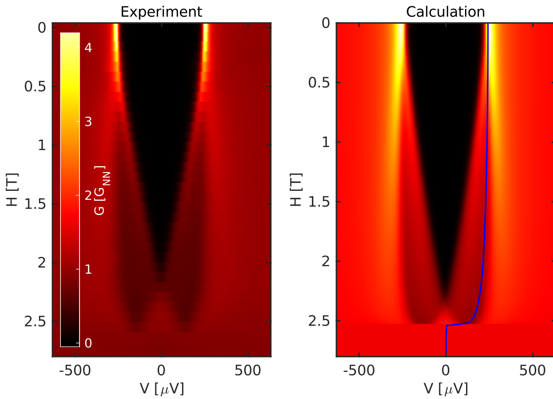
Figure 2.4: A color-map of the NIS G(V) curves as a function of the magnetic field, from the experiment (left), and from the theory (right) using the equilibrium self-consistent \Delta(H) (blue curve).
