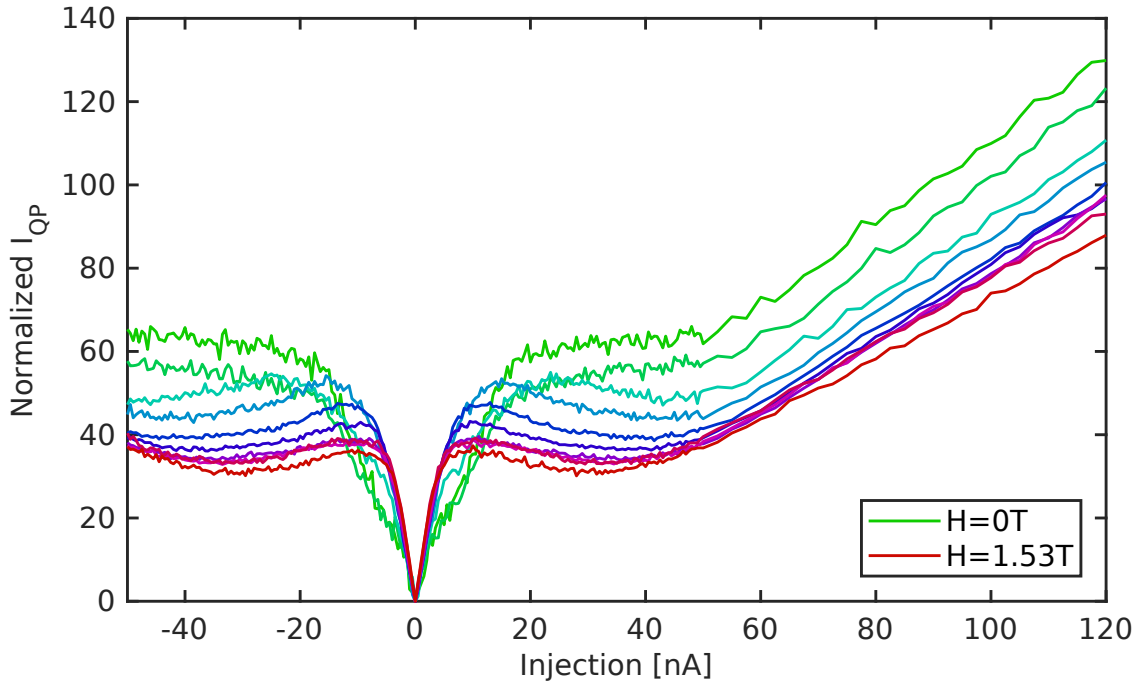
Figure 3.6: The number of quasiparticles measured at J_1 as a function of the applied magnetic field (10 equidistant steps from H = 1.53\text{T} to H = 0\text{T} ) and the injection current.
