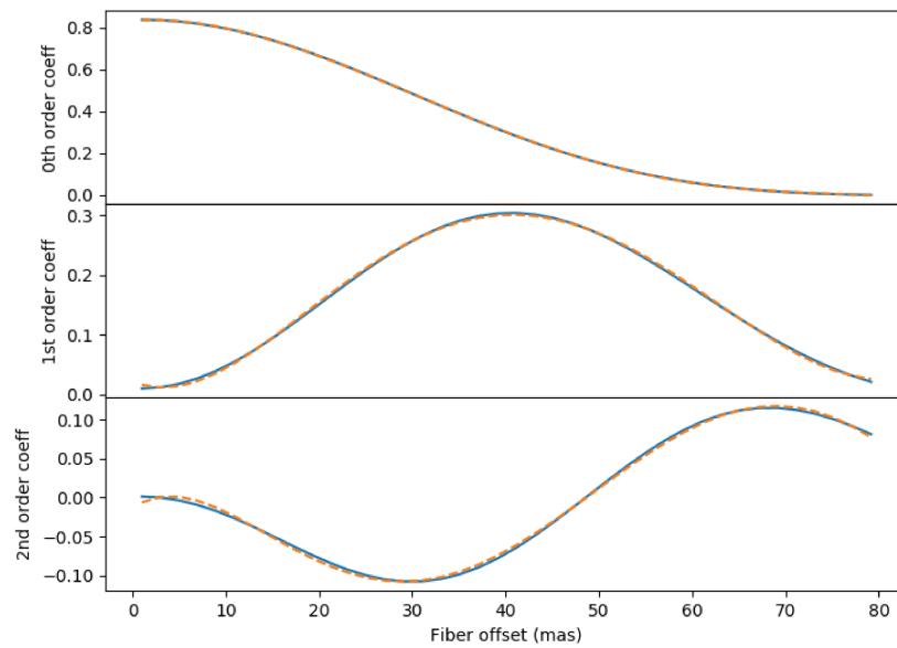
Figure A.5: Coefficients a_0 (top), a_1 (middle), and a_2 (bottom) versus fiber offset \theta in milli-arcsecond. The blue line represent the numerical calculation (assuming a circular aperture), and the orange dotted line is a 5-th order polynomial fit. The coefficients of the different fits are given in Table A.1
