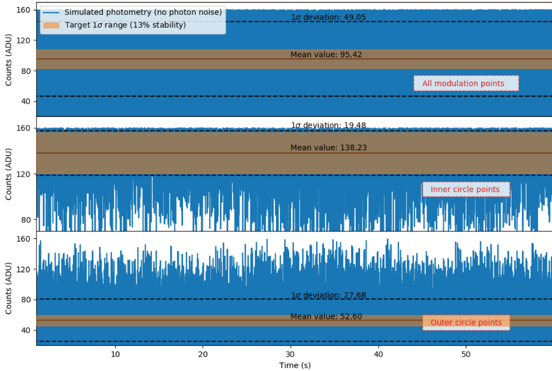
Figure 4.25: Same as Figure 4.22, for Scenario 3 (ASTERIA errors, scaled up to 10 as at 1\sigma , but now using a star modulation pattern with an inner circle radius of 0.1 FWHM, an outer circle radius of 0.5 FWHM, and adding in the measurements from the gyroscope to help stabilize the whole control loop.
