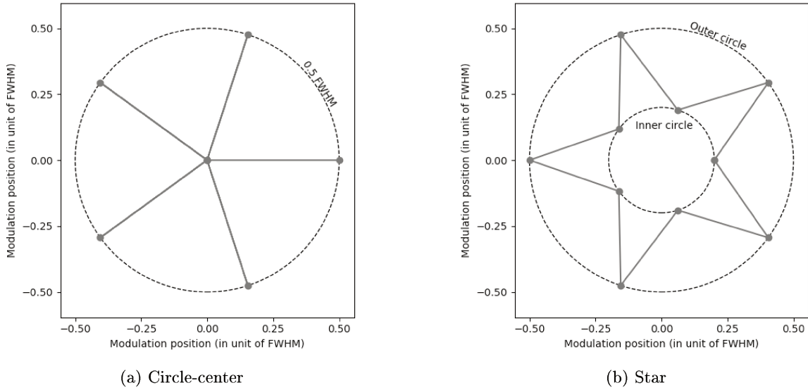
Figure 4.21: Two alternative modulation patterns which can be used to improve the performance of the algorithm.
