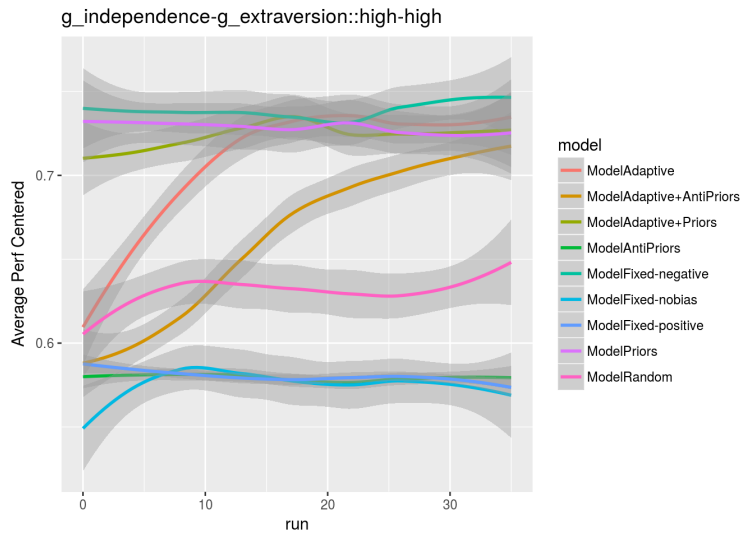
Figure 5.8: Evolution of performance within runs for a virtual user that is highly independent and highly extroverted, denoted as g\_independence-g\_extraversion::high-high ( g_ stands for group). For this user, negative fixed model performs best.
