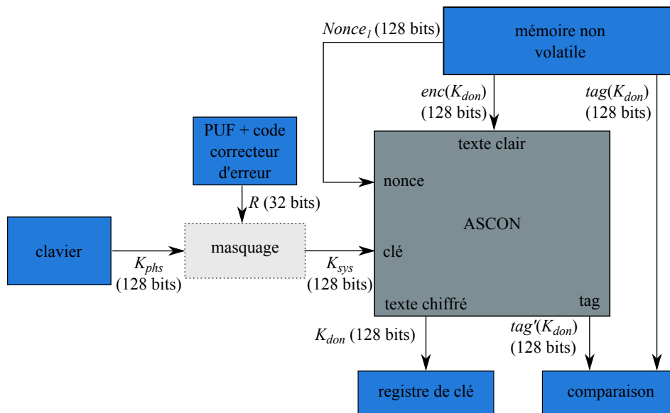
FIGURE 2.12: Phase d'activation
