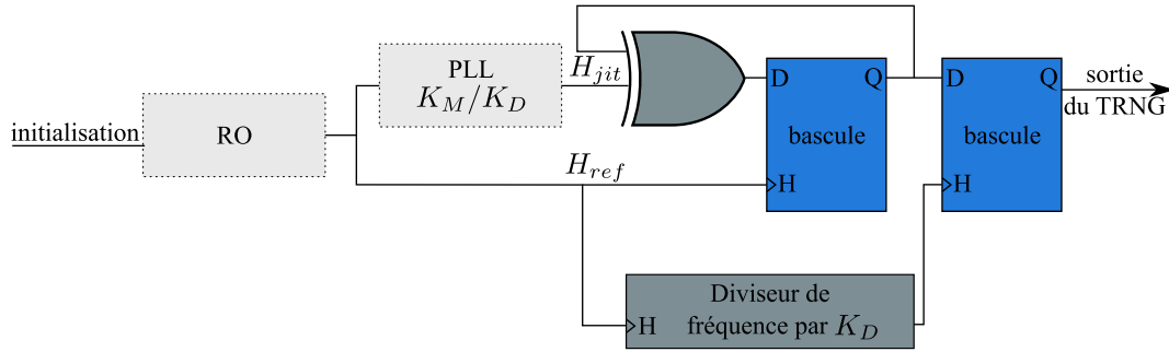
FIGURE 1.11: Structure PLL-TRNG
