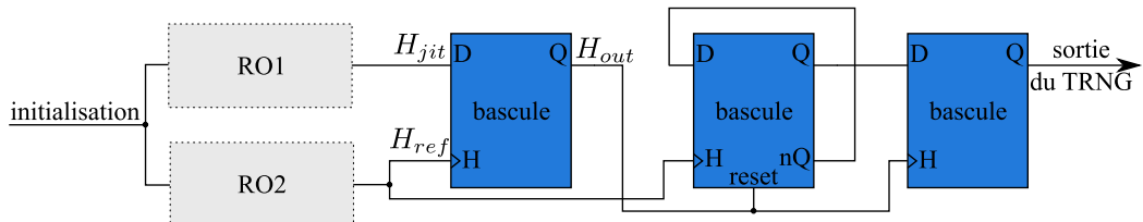
FIGURE 1.13: Structure COSO-TRNG
