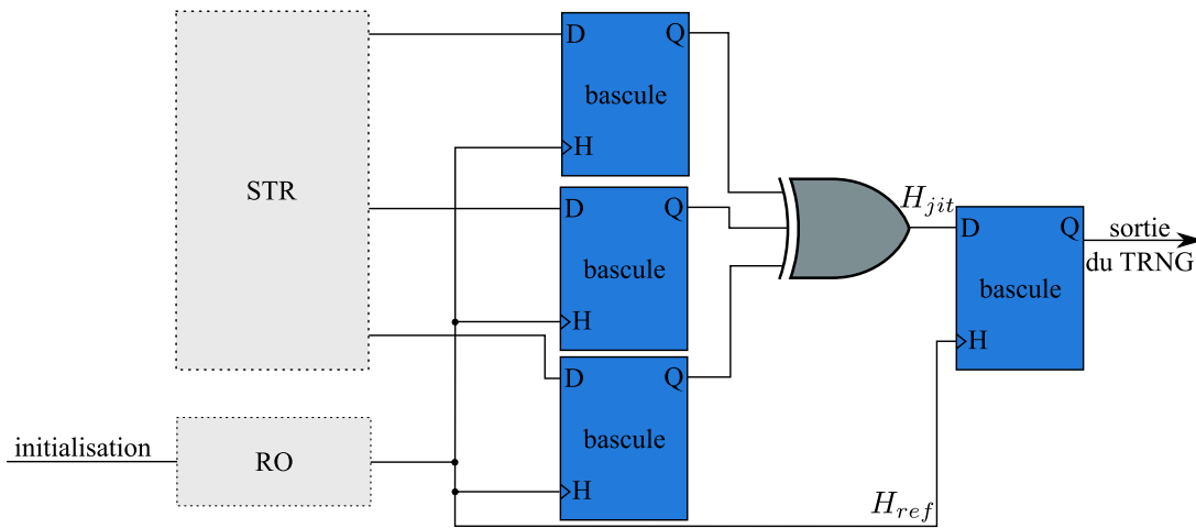
FIGURE 1.16: Structure STR-TRNG
