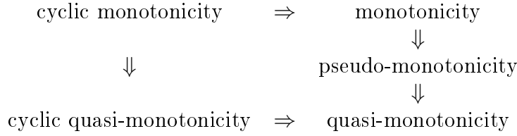
Figure 1: Generalized monotonicity properties
