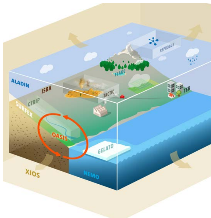
Figure 2.1: Schematic of the components of the CNRM-RCSM6 model. Credits: CNRM
