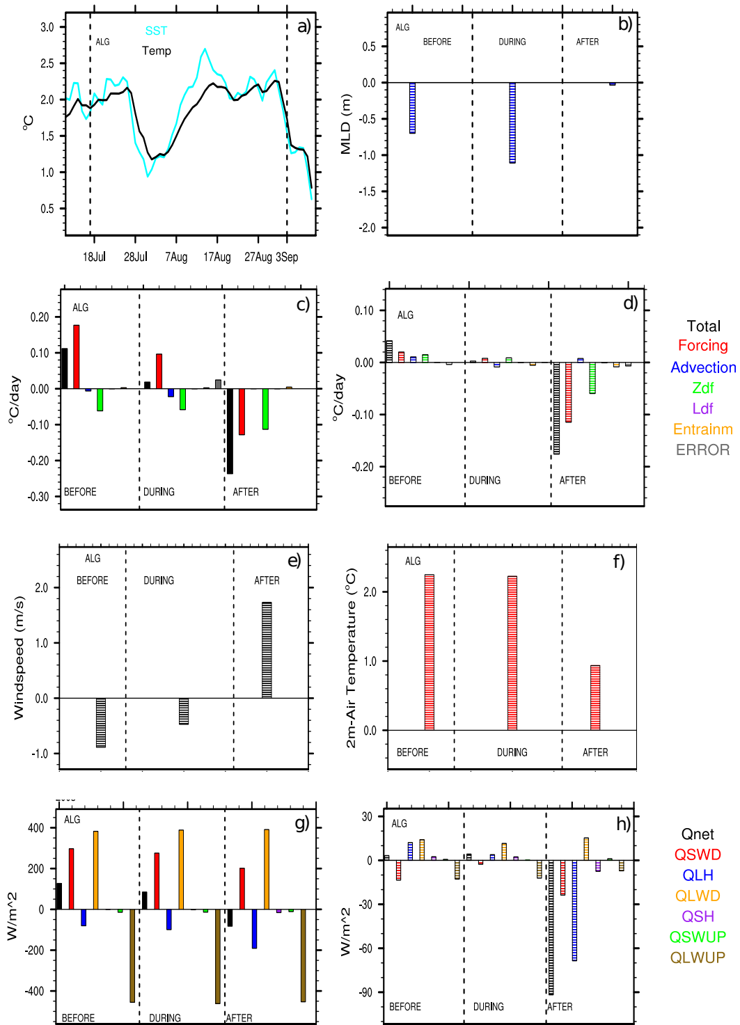
Figure 4.7: As in Fig.4.4 but for the Algerian Sea domain.
