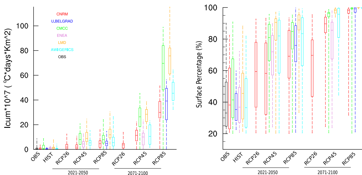
Figure 5.12: Whisker diagram of (left) Severity ( Icum ) and (right) maximum surface coverage of every observed and simulated MHW during HIST, 2021-2050 and 2071-2100. Box plots illustrate minimum, 25th percentile, median, 75th percentile and maximum values of each variable for a given model, scenario and period.
