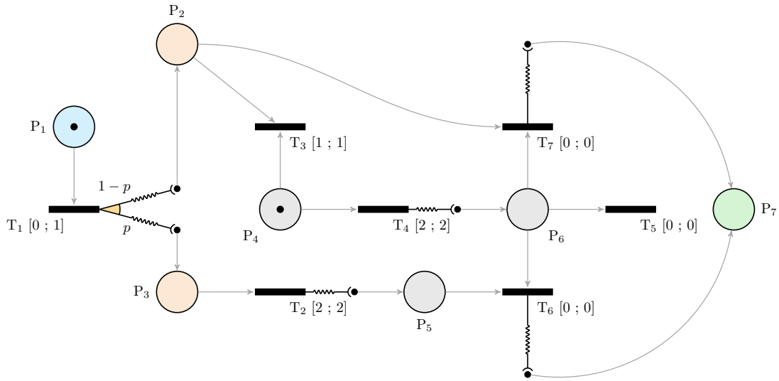
Figure 3.7 – The probabilistic time Petri net \mathcal{N}_1
