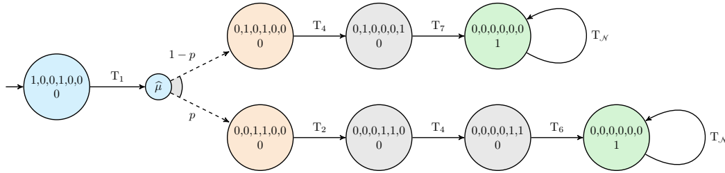
Figure 3.10 – Abridged representation of the duplicitious adversary \Lambda_1
