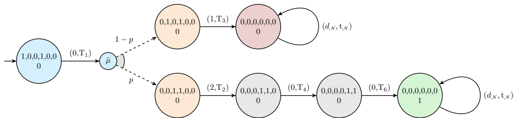
Figure 3.8 – Abridged representation of the scheduler \mathfrak{S}_1
