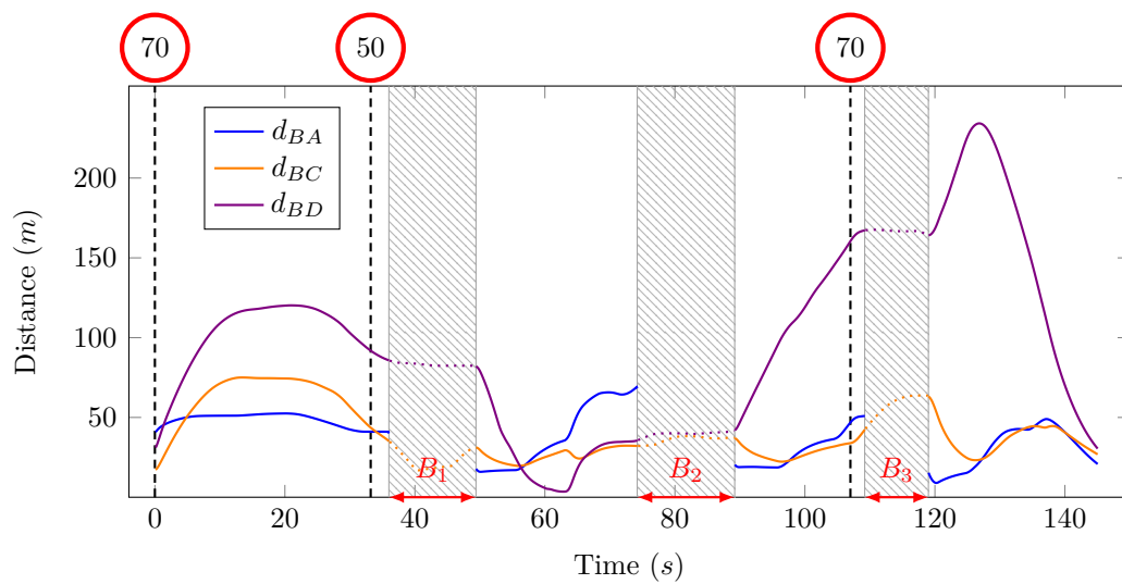
Figure 5.7 – Inter-vehicle distances when v_A is set to 20 \text{ km.h}^{-1} in scenario S_2
