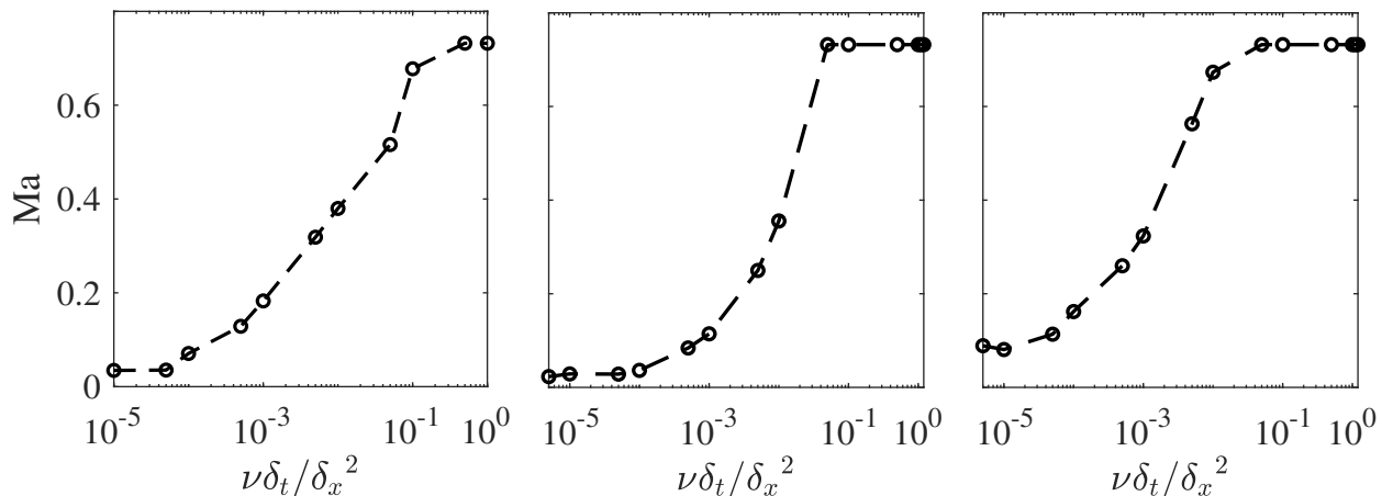
Figure 3.8: Linear stability domains of SRT collision operator with EDFs of orders (from left to right) two, three and four
