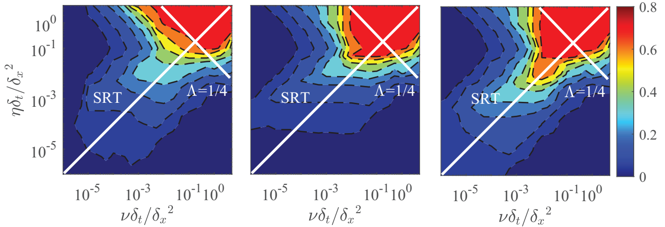
Figure 3.17: Linear stability domain of the TRT collision operator for EDF of orders (from left to right) two, three and four. The color bar shows the maximum achievable Mach number.
