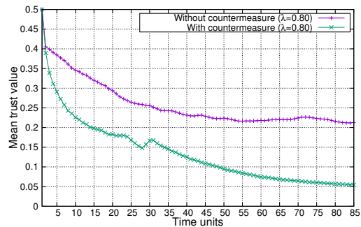
Figure 5.9 – Trust under cooperative ballot-stuffing attacks
