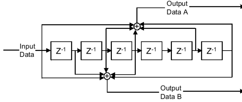
Figure 4.2 – Convolutional Encoder.
