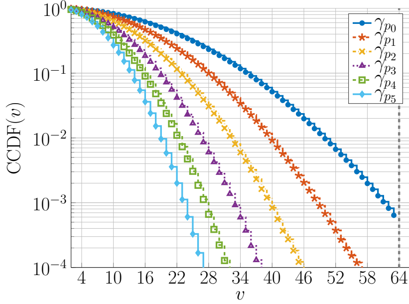
Figure 3.5 – CCDF of the required number ( v ) of IFFTs with different thresholds \gamma_{p_i}[\text{dB}] .
