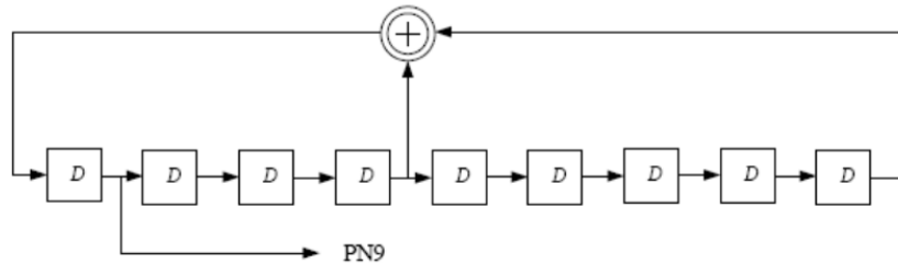
Figure 4.3 – The PN9 sequence.
