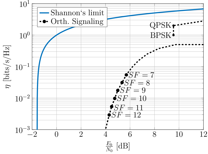
Figure 3.11 – The spectral efficiency as a function of the required SNR per bit to attain a \text{BER} = 10^{-5} for orthogonal signaling modulations and BPSK/QPSK modulation.
