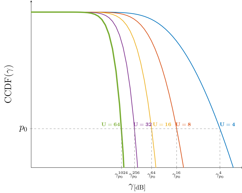
Figure 3.1 – \text{CCDF}(\gamma) for GreenOFDM with a given number of subcarriers N = 64 and a given set of values of U = 4, 8, 16, 32 and 64 .
