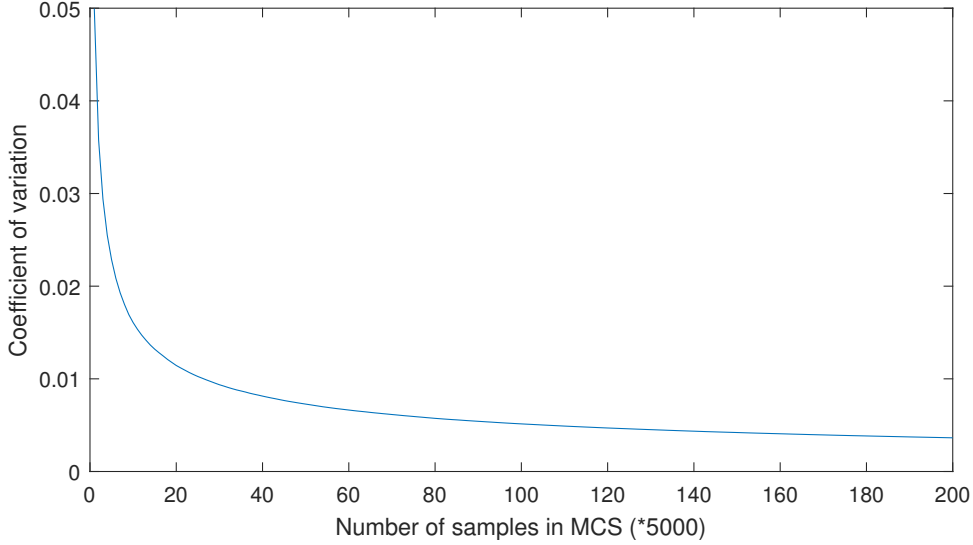
Figure 2.6: Coefficient of variation of the estimated P_f
