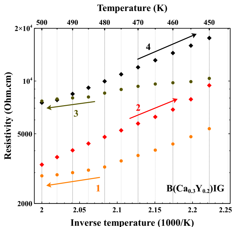
FIGURE 5.5: Resistivity (logarithmic scale) as a function of inverse temperature for B(\text{Ca}_{0.3}\text{Y}_{0.2})\text{IG} under air atmosphere during heating (1 and 3) and cooling (2 and 4). The numbers (1,2,3 and 4) indicate the order in which the measurements were done.
