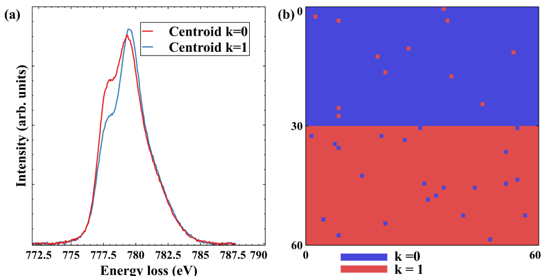
FIGURE 3.25: a) centroids output of the K-means++ algorithm on a synthetic SpIm. b) map of the labels of a synthetic SpIm as computed by the cluster analysis.
