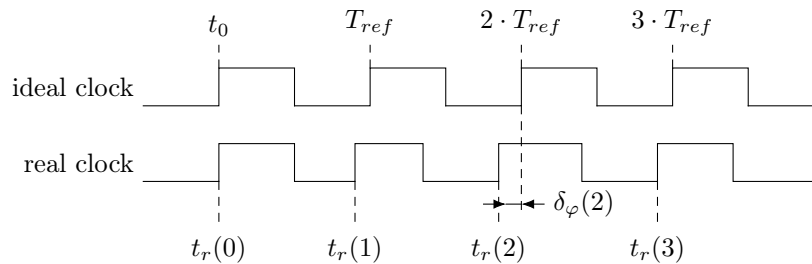
Figure 1.3: Illustration of the phase jitter of the second rising edge of the clock signal
