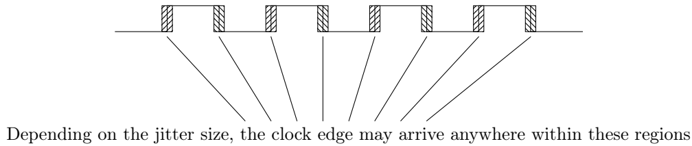
Figure 1.1: Clock jitter
