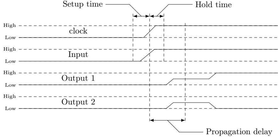
Figure 1.8: Example waveforms of a metastable register
