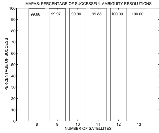
(b) Percentage of successful trials (MAPAS)
