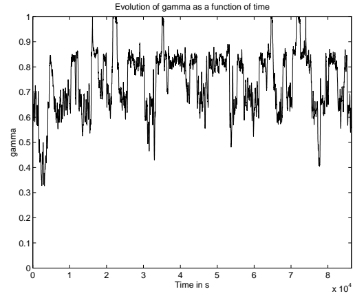
(b) Evolution of \gamma over 24h (primary satellites with minimum PDOP). Mean = 0.7, std = 0.12, min = 0.33, max = 1.
