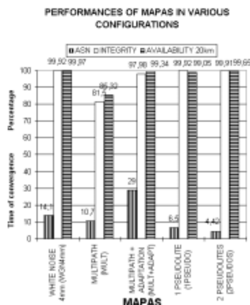
Figure 8.12: Summary of MAPAS simulation results
