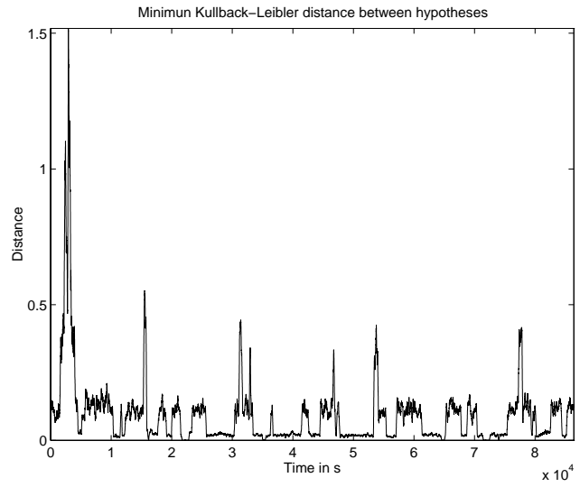
(b) Average minimum distance between 2 hypotheses over 24h (primary satellites with PDOP close to 7.5). Mean = 0.09, std = 0.13, min = 5.0 \times 10^{-4} , max = 1.52.
