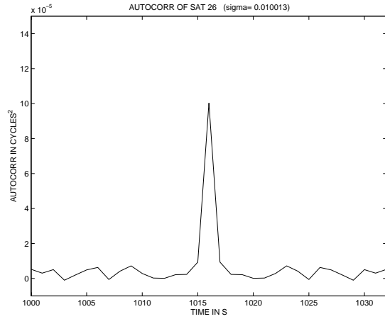
(c) Zoom of autocovariance of double differenced phase noise of satellite 26
