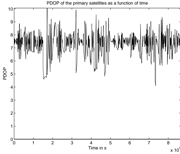
(a) PDOP of the primary satellites (second case).
