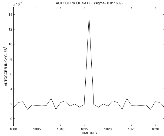
(d) Zoom of autocovariance of double differenced phase noise of satellite 6
