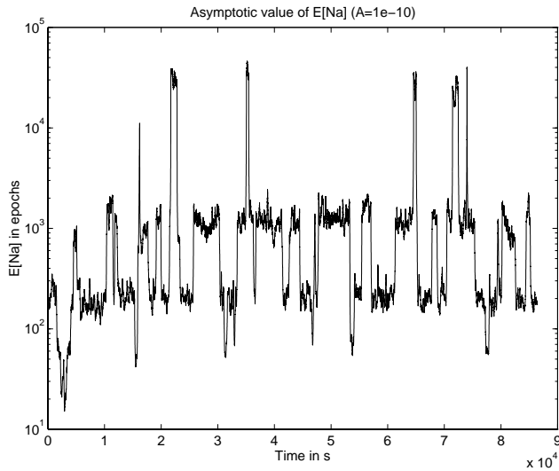
(c) Asymptotic value of the expected stopping time over 24h (primary satellites with PDOP close to 7.5). Mean = 1674, std = 5.3 \times 10^3 , min = 15.2, max = 4.6 \times 10^4 .
