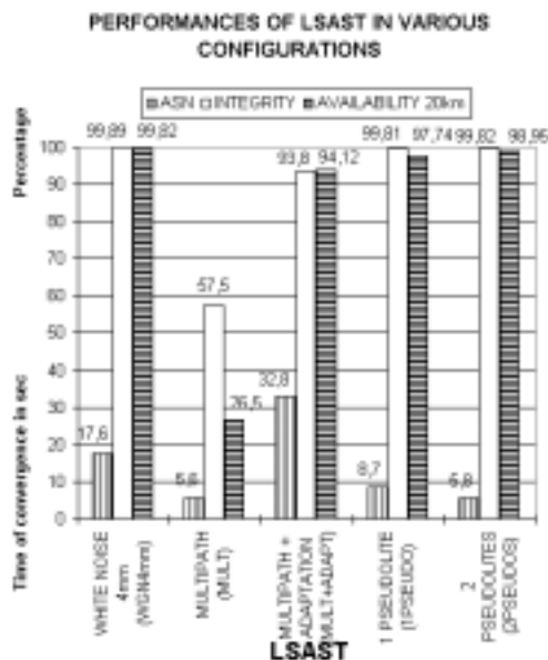
Figure 8.11: Summary of LSAST simulation results
