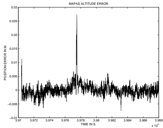
(d) Altitude error of MAPAS (with respect to GEOTRACER solution).
