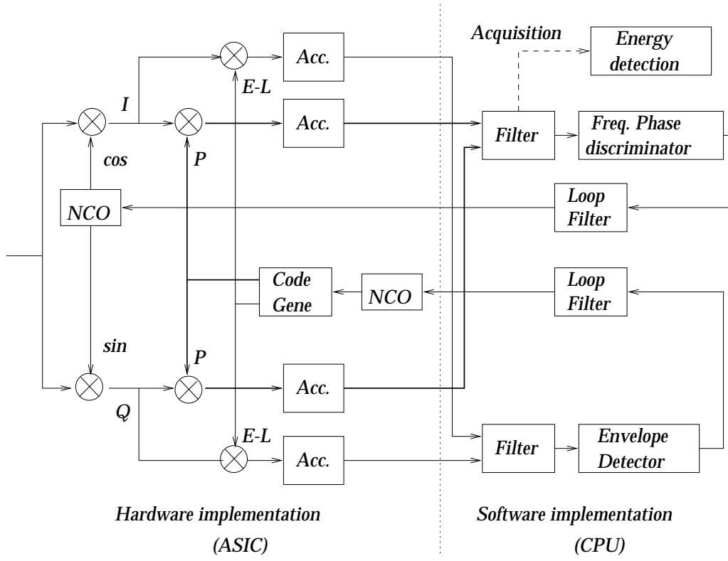
Figure 3.7: Typical architecture of a modern GPS receiver.
