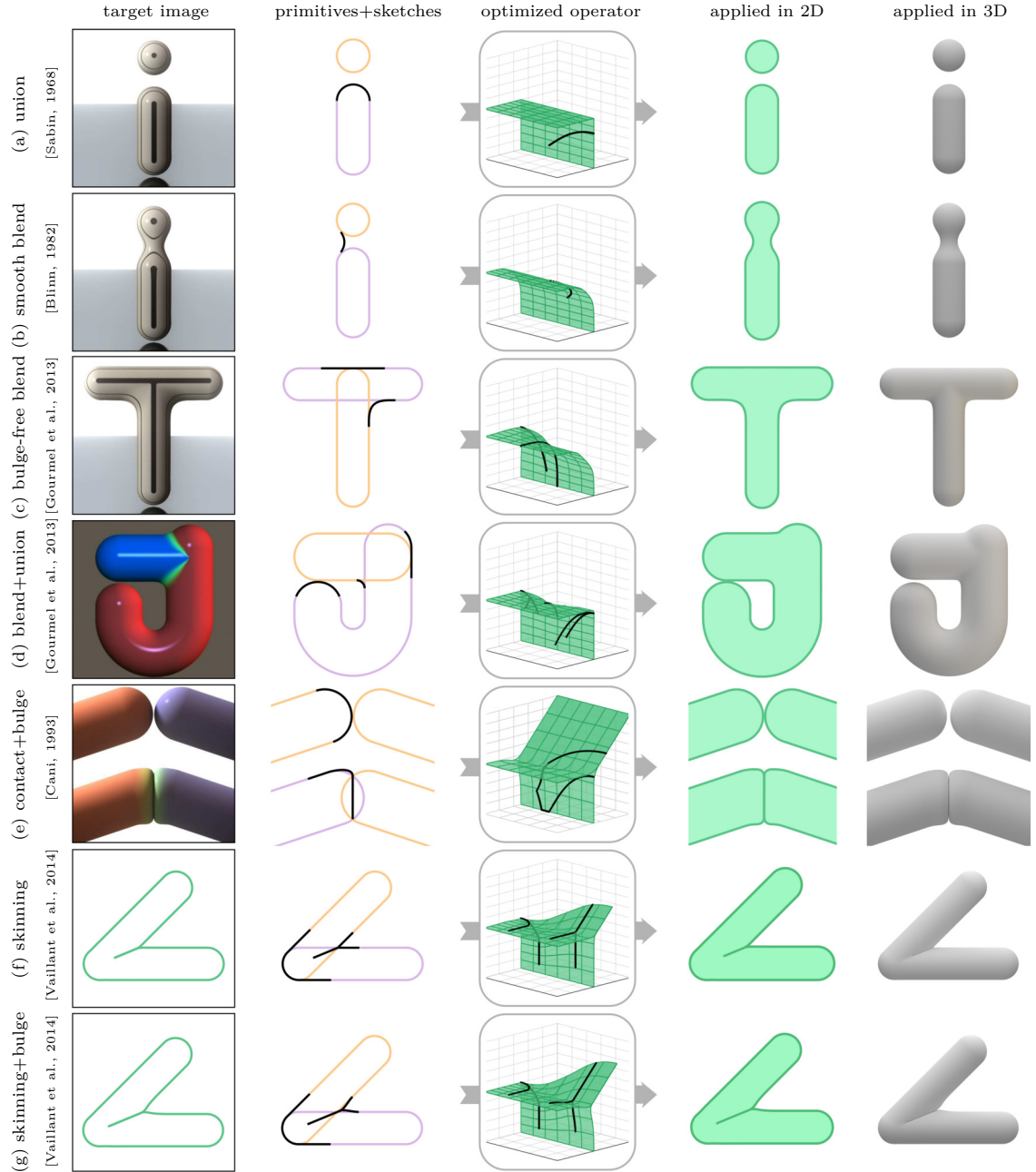
Figure 2.21: Our sketch-based construction method can be used to effortlessly produce every gradient blend operator proposed in past literature (pioneering citation is indicated). Starting from images depicting the final results of each operator (leftmost column), we simply sketched over 2D contour (second column). From these sketches, our system reverse-engineers the operator (central column). This can be applied (in 2D or 3D alike, rightmost columns) to reproduce the same results. Our target images are courtesy of [Gourmel et al., 2013] and [Vaillant et al., 2014].
