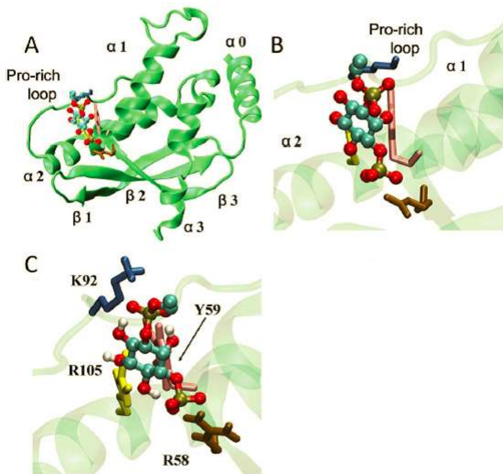
Figure 28. PI3P bound to P40 phox PX domain.
