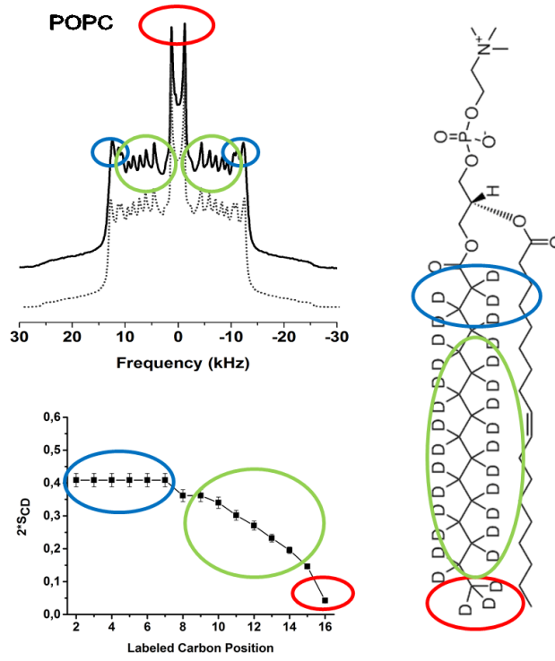
Figure 39: Order Parameter Profile. Top: NMR spectrum and its simulation (dotted line) of 2 H-POPC in MLV. Right: Molecular structure of 2 H 31 -POPC. Bottom: order parameter profile representing S_{CD} as a function of deuterated carbon number of 2 H 31 -POPC.
