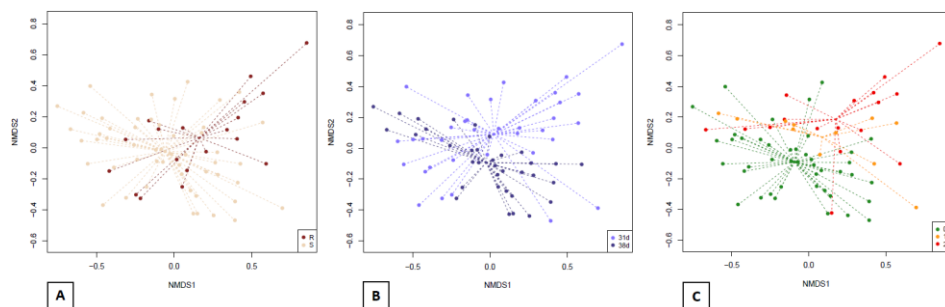
Figure 1: Plots include only the samples obtained from T0. Dissimilarities in gut microbiota composition represented by the non-metric multidimensional scaling (NMDS) ordination plot, with Bray-Curtis dissimilarity index calculated on unscaled OTU abundances. The centroids of each group are features as the group name on the graph (“envfit”; Vegan R package). Samples are coloured by MUC4 gene (A): resistant (R, red) and susceptible (S, pink) genotypes; by age (B): 31 days-old (31d, light blue) and 38 days-old (38d, blue) and by faecal score (C): category 0 (green), 1 (orange) and 2 (red).
