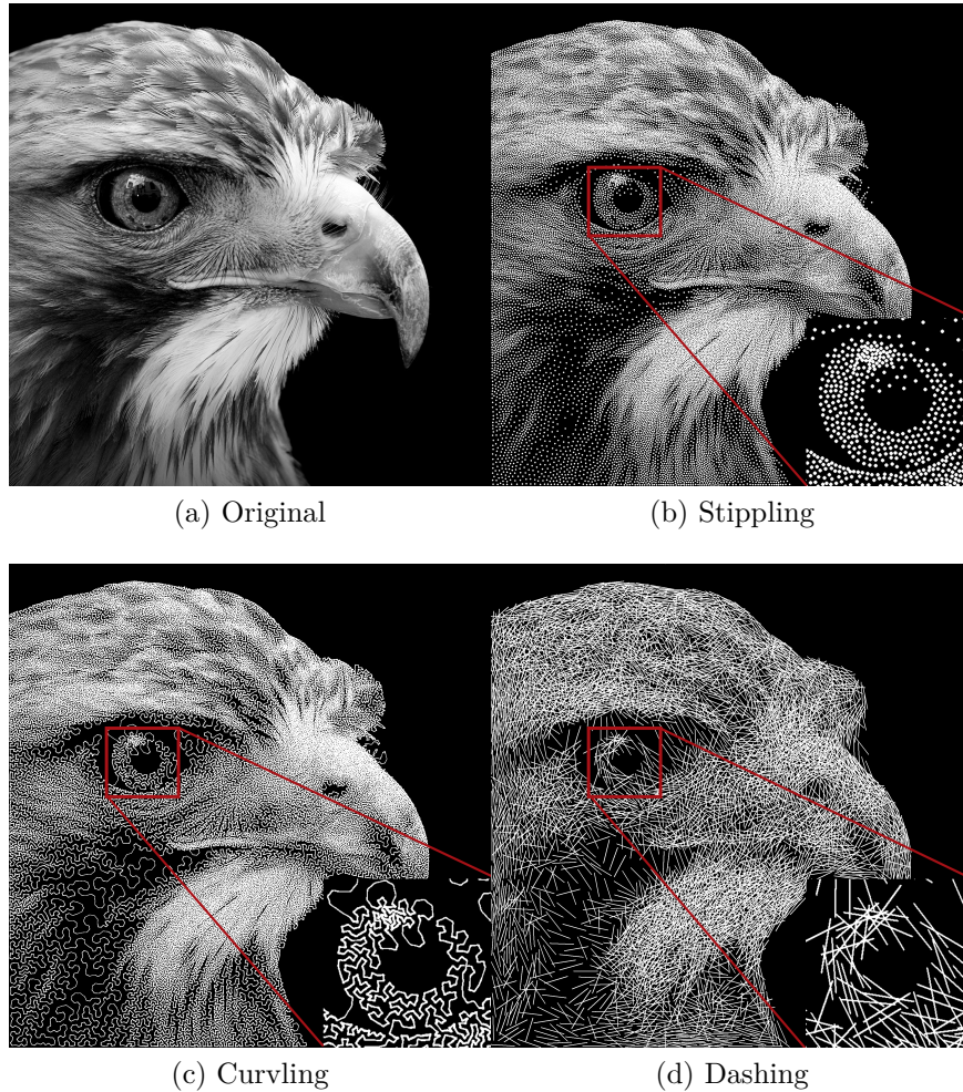
FIGURE 5.1 – Approximating an image with a measure supported on points (stippling, 100k, 202"), curve (curvling, 100k, 313") or segments (dashing, 33k, 237"). In each case, the iterative algorithm starts from a set of points drawn uniformly at random.
