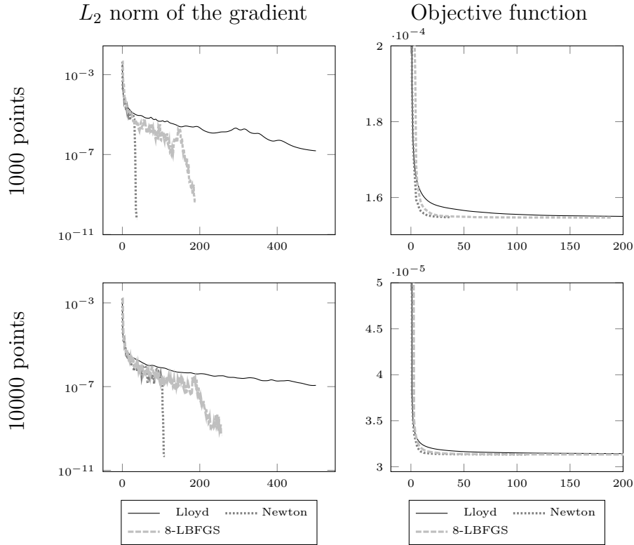
FIGURE 4.4 – Blue Noise problem with 1Kpts (Top) and 10 Kpts (Bottom). Left : norm of the gradient, Right : evolution of the cost function.
