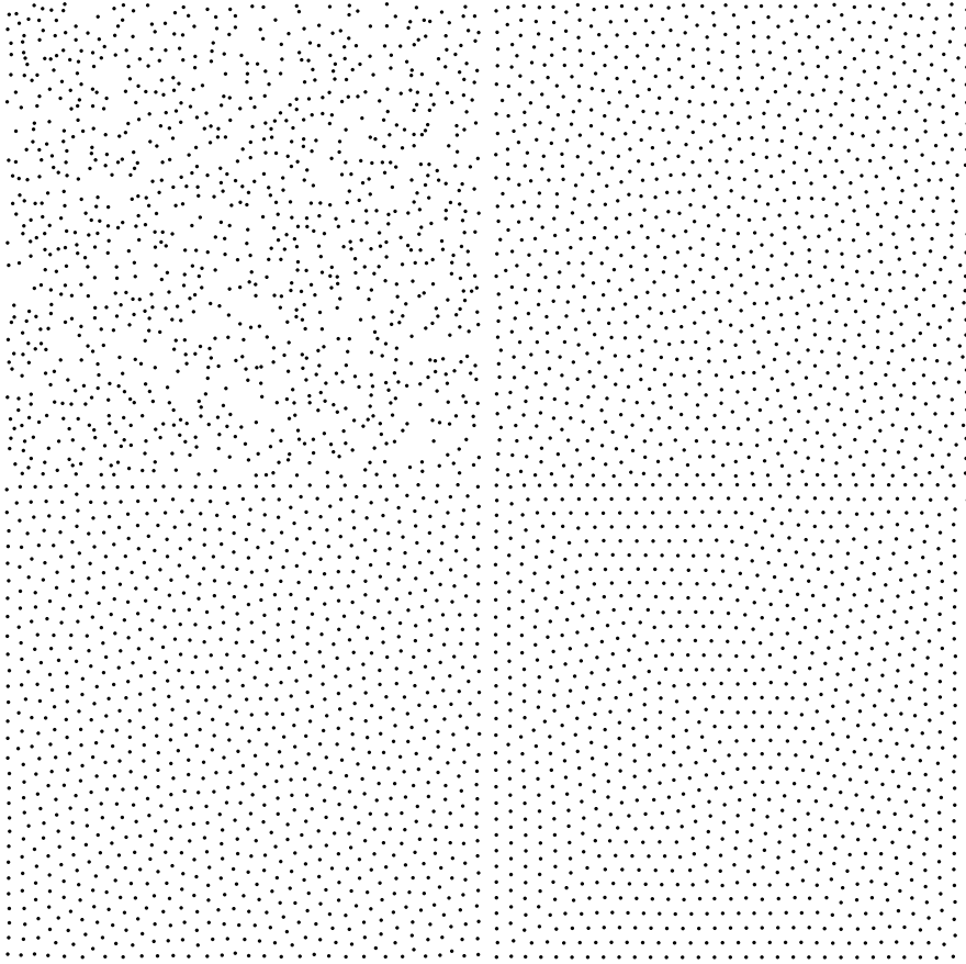
FIGURE 5.3 – Evolution of the PSNR through iteration : top left 8dB, top right 25dB, bottom left 31dB, bottom right 34dB
