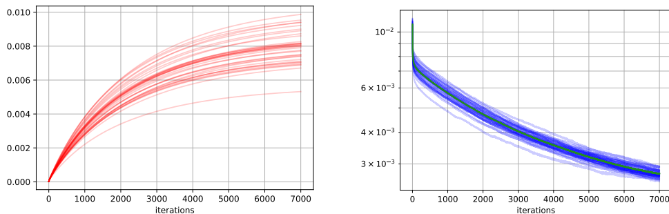
FIGURE 6.6 – Gradient ascent method : cost function history (left) and norm of the gradient (right). Method stopped by the max iteration criterion.
