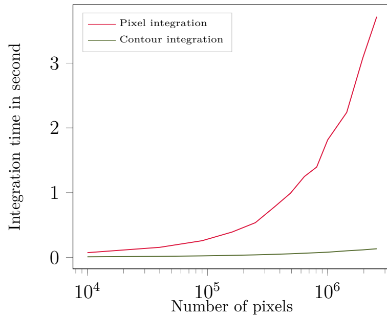
FIGURE 8.1 – Time to compute the gradient of the Monge Kantorovitch functional for an increasing number of pixels and a fixed number of Dirac masses in the discrete measure.
