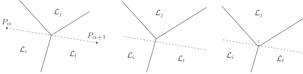
FIGURE 6.3 – Example of non-uniqueness to the minimization problem (6.23). At the left the polyline [P_\alpha, P_{\alpha+1}] intersects the junction of 3 Laguerre cells (i, j, l) . In the center k = l chosen as expected. At the right k = j chosen and t_e^{j\alpha} - t_s^{j\alpha} = \varepsilon , a small error occurs assigning a bit of the segment to the j th Laguerre cell.
