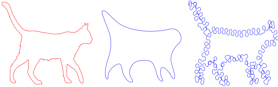
FIGURE 5.4 – Examples of projections of a curve (in red) on spaces of curves with constraints (in blue). Center : projection on sets of curves with smaller length and bounded curvature. Right : projection on sets of curves with longer length and bounded curvature.
