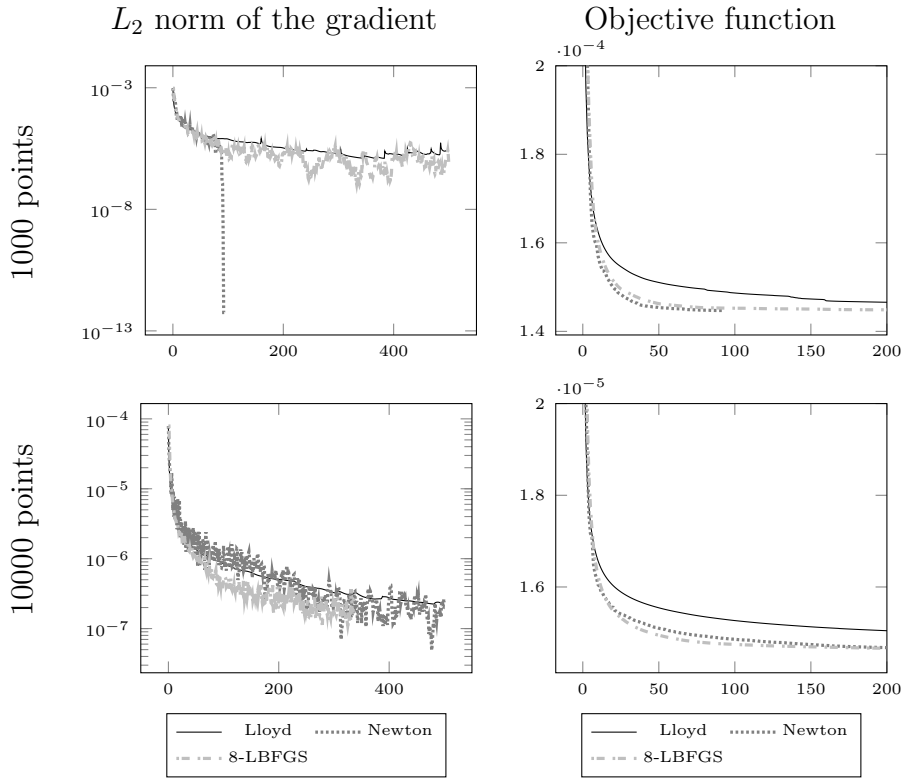
FIGURE 4.3 – Stippling problem with 1Kpts (Top) and 10 Kpts (Bottom). Left : norm of the gradient, Right : evolution of the cost function.
