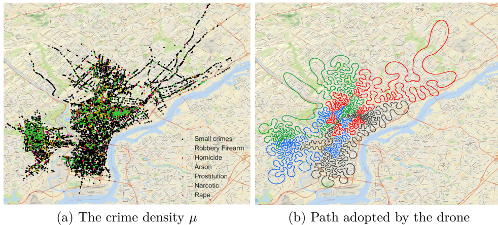
FIGURE 5.7 – The data superimposed on a map of Philadelphia. A possible drone trajectory made. In this example, the drone passes 4 times to its recharging location, explaining the different colors of the trajectory. In this example, the trajectory was discretized with 8k points and optimized in 30”.
