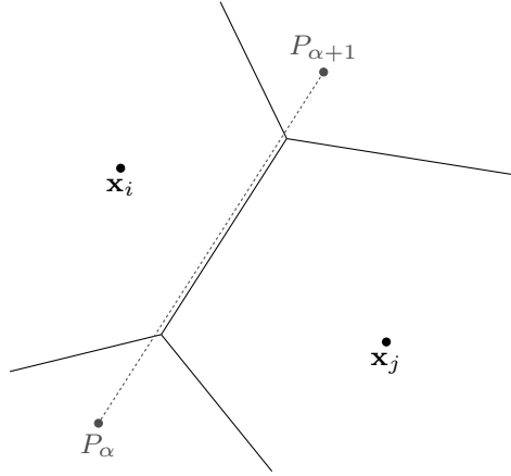
FIGURE 6.1 – When the hypothesis (H) is violated one can cook up a \phi such that the functional g in (6.5) is no longer \mathcal{C}^1 with respect to \phi . Here a small perturbation on \phi_i or \phi_j induces a discontinuity on \nabla_\phi g .
