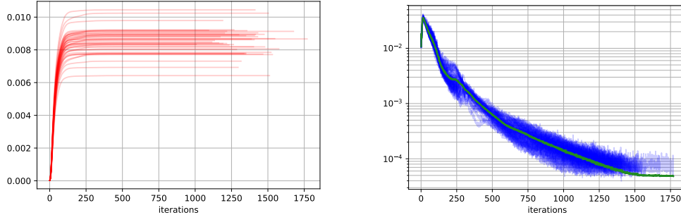
FIGURE 6.8 – L-BFGS method : cost function history (left) and norm of the gradient (right). Method converges to the targeted gradient norm 5.10^{-5} in a average of 1500 iterations.
