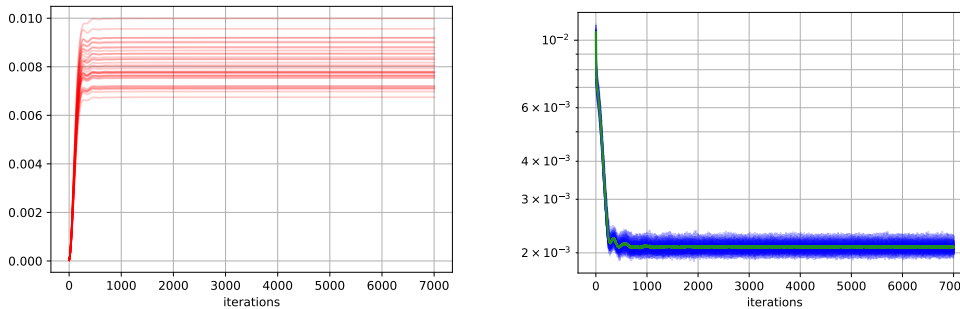
FIGURE 6.7 – Nesterov acceleration of gradient ascent : cost function history (left) and norm of the gradient (right). Method stopped by the max iteration criterion.
