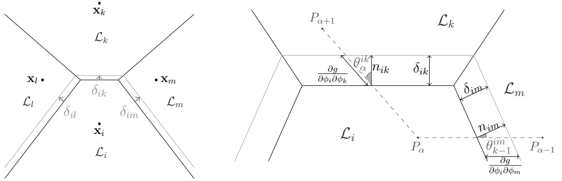
FIGURE 6.2 – (Left) Normal displacements (\delta_{il}, \delta_{ik}, \delta_{im}) of the boundary of the Laguerre cell when \phi_i increases and (\phi_l, \phi_k, \phi_m) remain constant. (Right) geometrical interpretation of the Hessian
