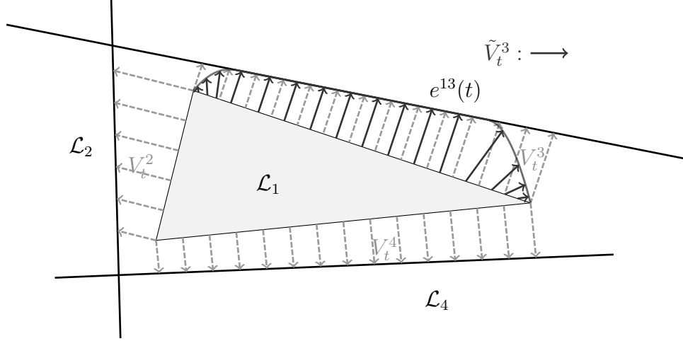
FIGURE 4.2 – Example of the vector fields V_t^3 and \tilde{V}_t^3 for i = 1
