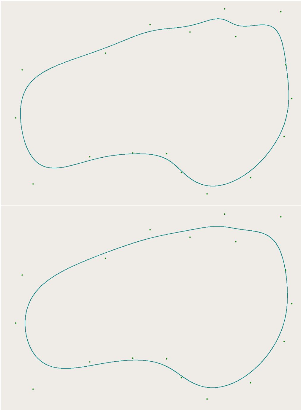
FIGURE 7.2 – Periodic approximation spline f (7.6) in blue for the controls points \mathbf{p} in green. The degree of the approximation spline is m = 5 (top) and m = 8 (bottom).
