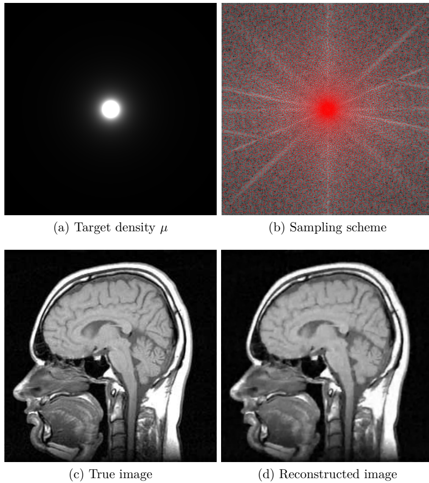
FIGURE 5.9 – Example of sampling scheme generation and image reconstruction in MRI. The target density \mu is shown in 5.9a. The sampling scheme generated by our algorithm is shown in 5.9b. The background shows the Fourier transform of u in log-scale. It contains one fourth of the total number of Fourier transform values. The true image and the reconstructed image are shown in Fig. 5.9c and 5.9d.
