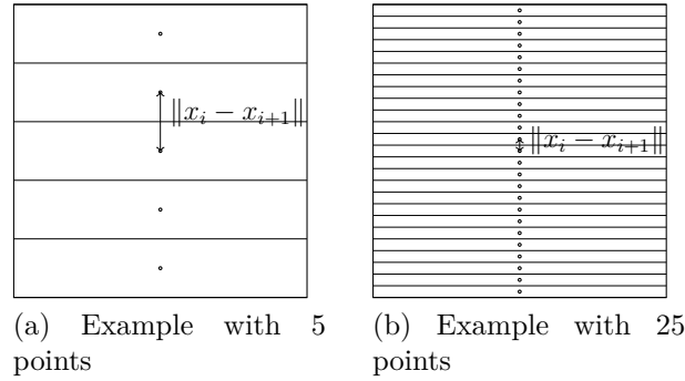
FIGURE 5.2 – Configurations of points generating a high Lipschitz constant for the gradient of g in \psi .
