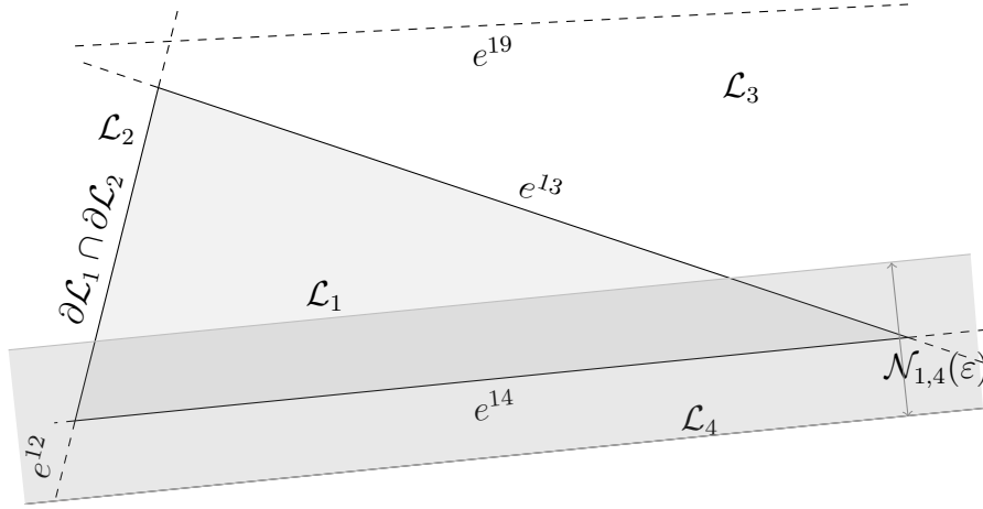
FIGURE 4.1 – Typical example of e^{ik} and the neighborhoods \mathcal{N}_{ik}(\varepsilon) for i = 1 .
