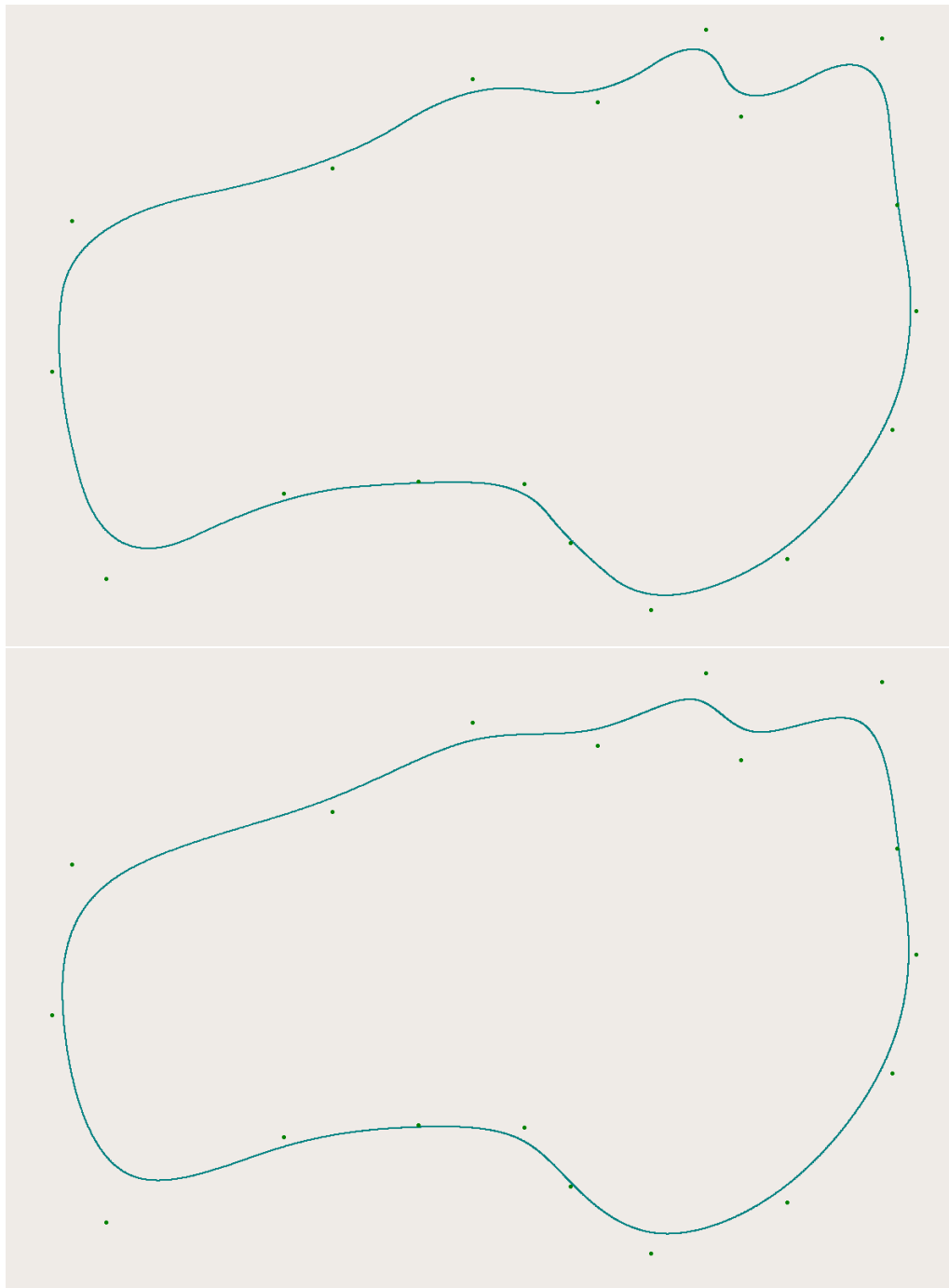
FIGURE 7.1 – Periodic approximation spline f (7.6) in blue for the controls points \mathbf{p} in green. The degree of the approximation spline is m = 3 (top) and m = 4 (bottom).
