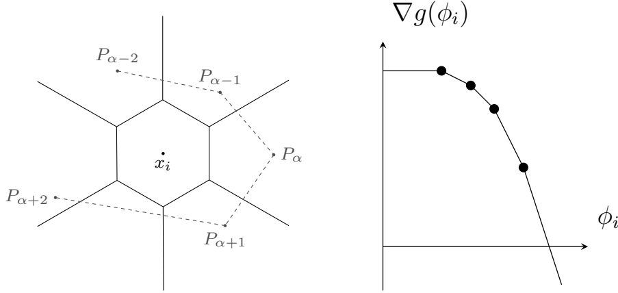
FIGURE 6.5 – Counter-example to the smoothness of \nabla g . Consider the a Laguerre tessellation and a set of segment as displayed in the left and increase \phi_i . The Laguerre cell \mathcal{L}_i increases and the gradient of g with respect to \phi exhibits kinks. Those kinks happen each time a Laguerre cell meets a line segment for the first time. Under Hypothesis (H) boundary segments of the Laguerre cell are never parallel to a line segment. If Hypothesis (H) is not met \nabla g may fail to exist.
