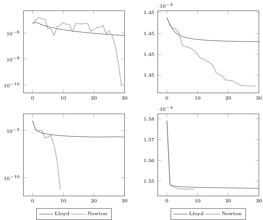
FIGURE 4.5 – Evolution of the cost function (Right) and the norm of the gradient (Left) for the Stippling problem (Top) and the Blue Noise problem (Bottom) when one point is added.
