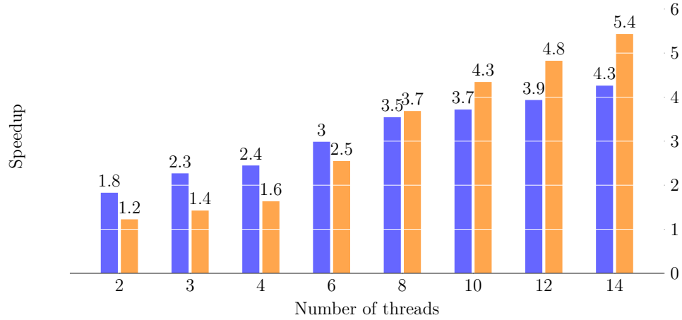
FIGURE 6.4 – Speedup for the computation of the cost function g with c++11 thread class in blue, and OpenMP in orange . The parallelism is placed over the segment integration for n = 200K points and p = 80K segments for an increasing number of threads with a super-calculator equipped with Intel Xeon ® E5-2680
