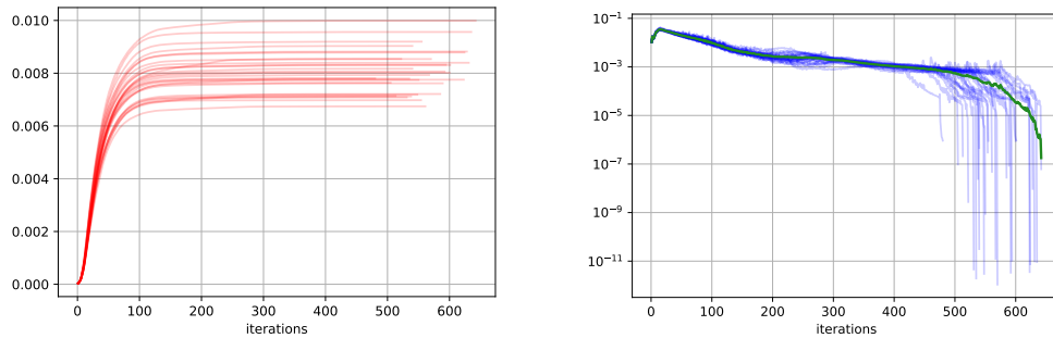
FIGURE 6.9 – Hybrid Newton method : cost function history (left) and norm of the gradient (right). The method converges to the targeted gradient norm 10^{-6} in 600 iterations on average.
