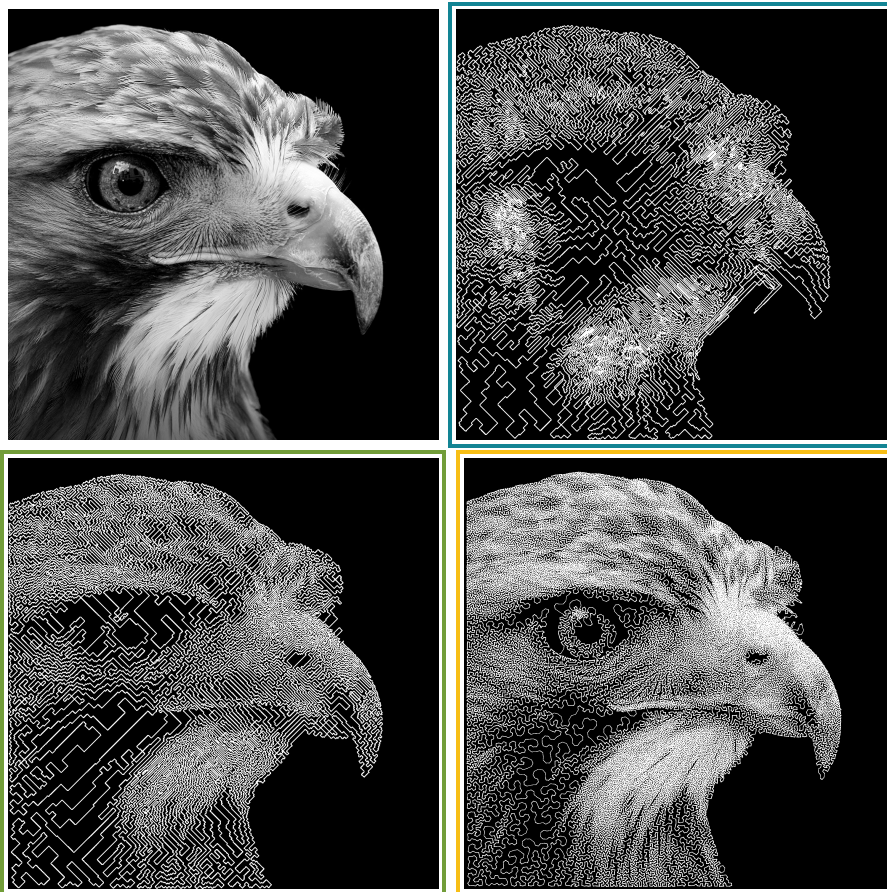
FIGURE 2.1 – The original image is top left. The other three images are curve approximations of the original one.
