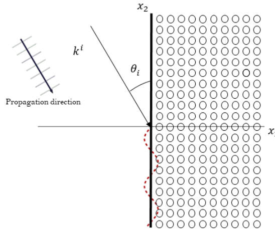
Figure 4.13: Simplified representation of the onset of an interface wave (in red) propagating along the interface between a homogeneous solid and a metamaterial. Depending on the relative stiffnesses of the two media, each of the existing low and high-frequency modes can either become Stoneley or remain propagative.
