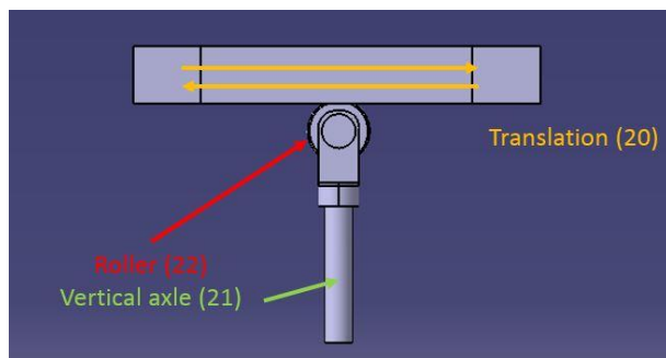
Figure P.2: XEHD Design, side view
