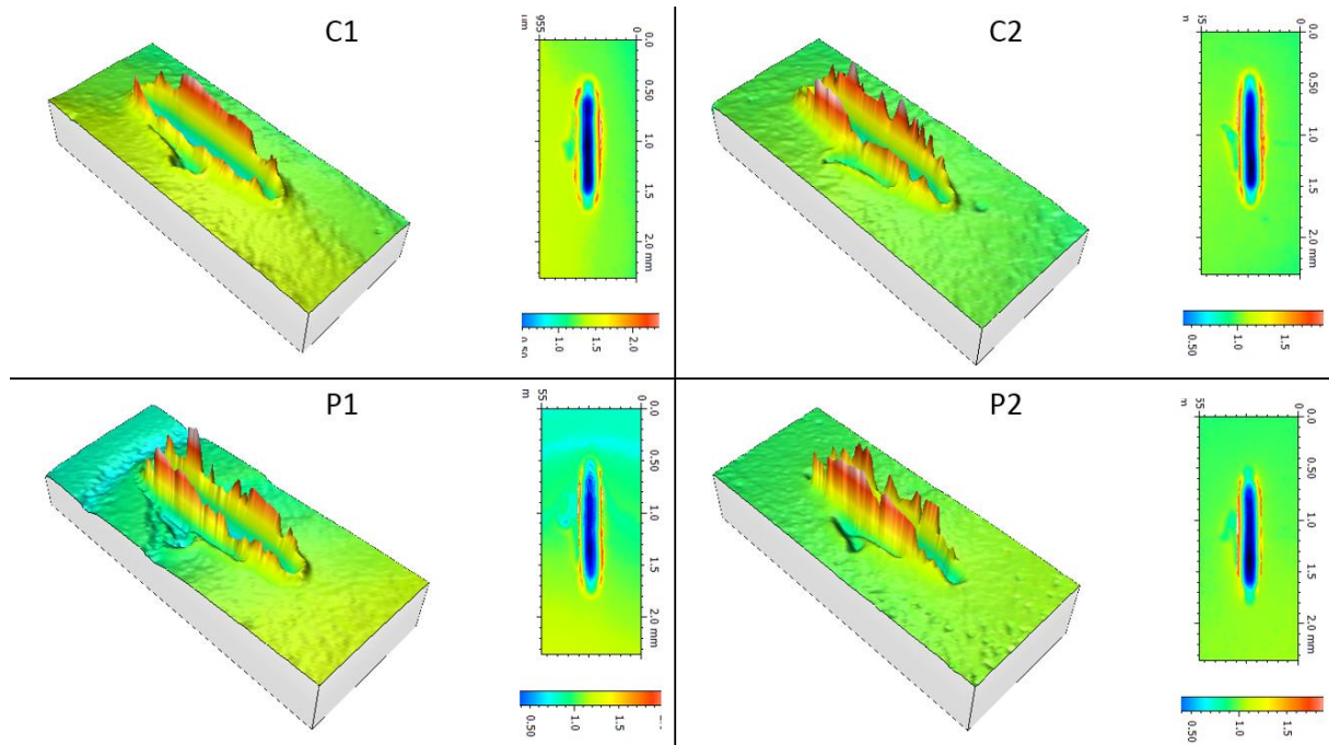
Figure 4.24: Interferometry example for 18h at 80°C
