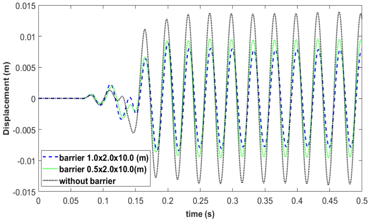
Figure 5-16 Time histories of displacement at the observation point in case of wave barriers with different depths, compared to the results obtained without barrier.
