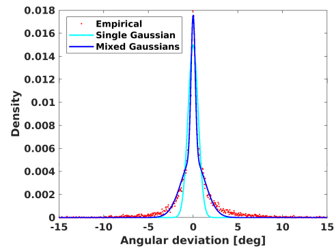
(d) source at (20, 20, 0) , 10 cm to the camera, 511 keV, FWHM = 1^\circ
