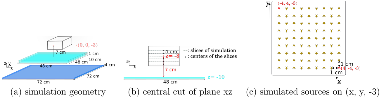
Figure 4.19: Illustration of the geometry of reconstruction for PSF estimation, the center of the reconstructed volume is located at (0, 0, -3) cm, distance 7 cm to the first scattering layer of the simulated Compton camera. The dashed lines in (b) correspond to the planes where the sphere sources were simulated. The plane closest to the camera is centered at (0, 0, -6) . The distance between each plane is 1 cm. (c) illustrates the 81 sphere sources (represented by stars) simulated separately on the plane z = -3 .
