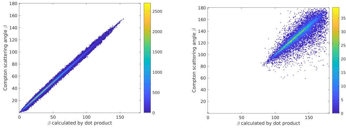
(a) First interaction occurs on the scatterers (sili- (b) First interaction occurs on the absorber (LaBr 3 con)
