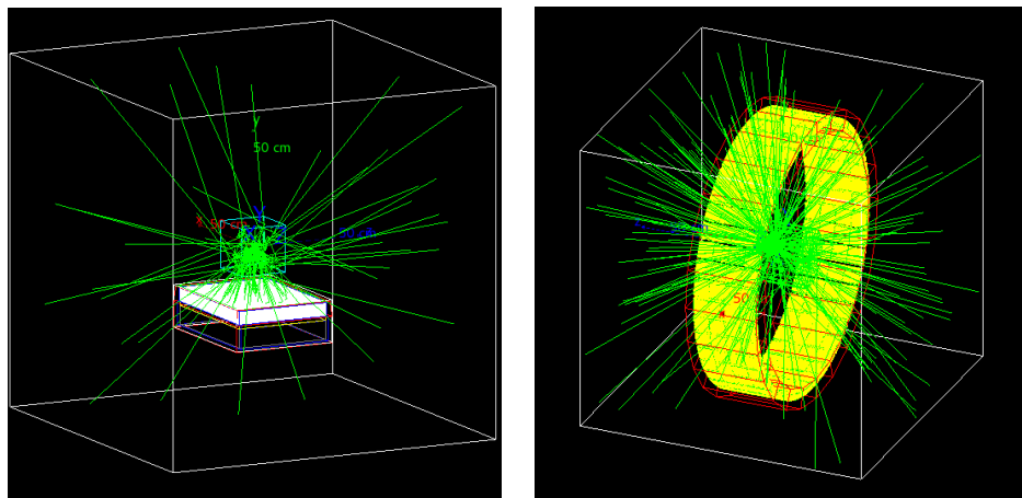
(c) A simplified simulation of a SPECT acquisition by a collimated camera. The emitted isotope is ^{111}\text{I} , the two emitted energies are 171 keV and 245 keV. The simulated phantom is water. (d) A simplified simulation of PET acquisition. The camera is composed of a 46x4 crystal block as a ring. Each crystal block contains 12x12 crystal. The phantom is a water cylinder. The source is in the cylinder, not centered.
