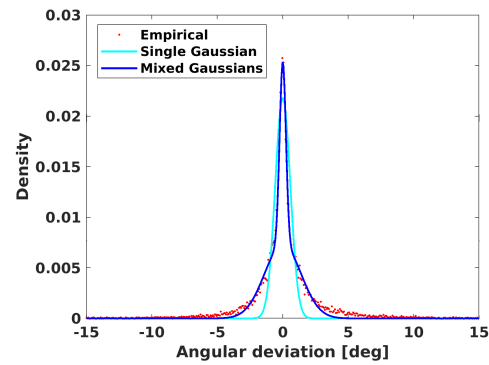
(b) source at (0, 0, 0) , 10 cm to the camera, 511 keV, FWHM = 1^\circ
