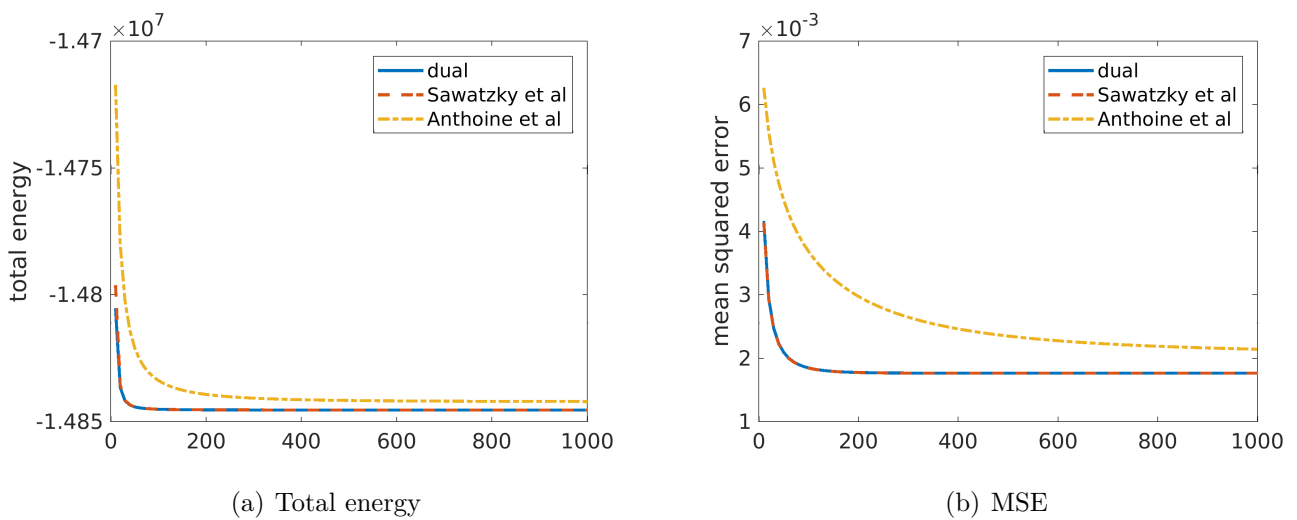
Figure 4.4: Figures of merit for the comparison of the proposed dual method (blue line), Sawatzky et al. method (red line) and Anthoine et al. method (yellow line) for MLEM reconstruction after 1 \times 10^3 iterations.
