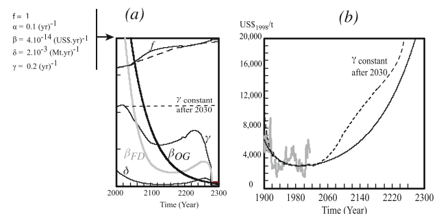
Figure 8. Evolution of (a) the model variables \beta_{OG} , \beta_{FD} , \delta , \gamma , and p_{TI} and (b) price where the gray, black, and dashed lines show historical data, conditions used to follow the reference price p_{TI} , and the case of constant \gamma_{OG} after 2030, respectively.
