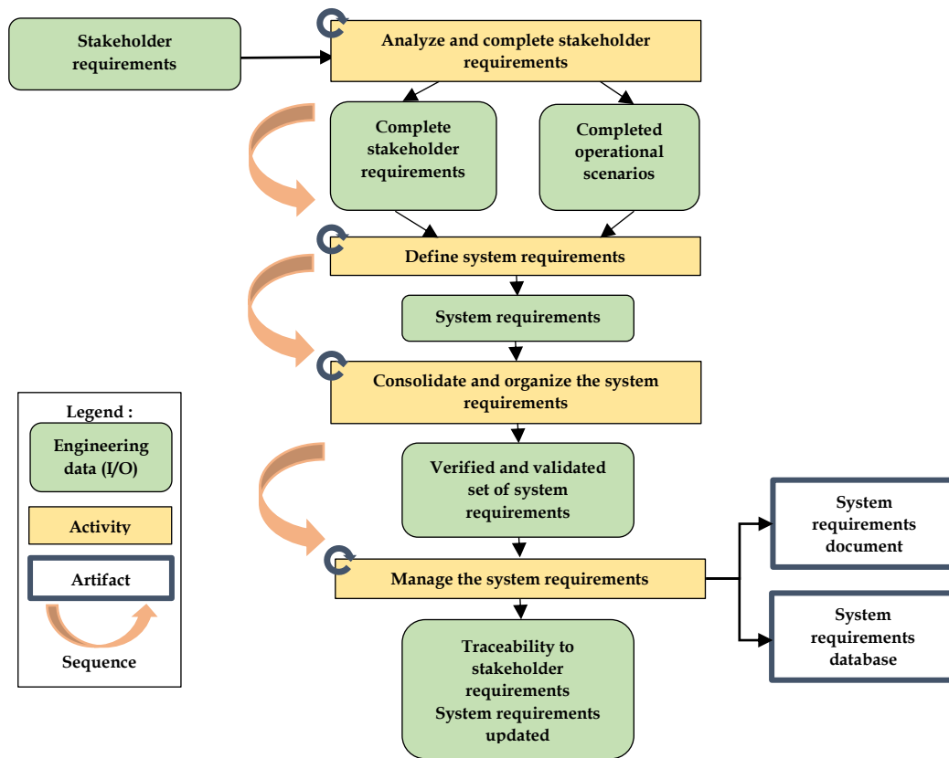
Figure 58 Activities of the System Requirements Definition Process (Faisandier, 2012, p.139)
