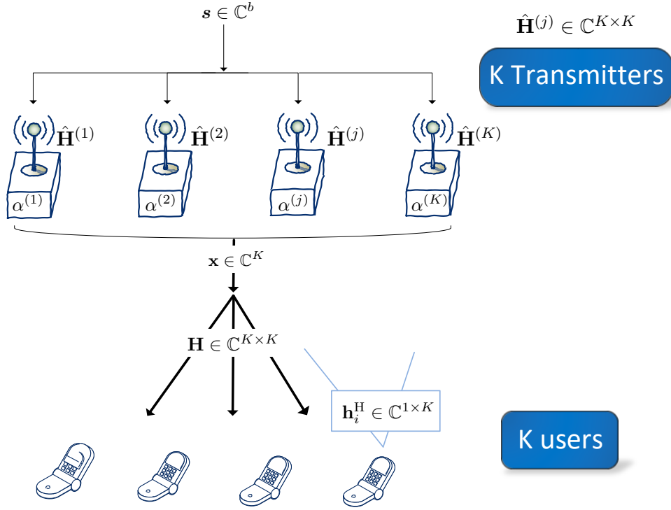
Figure 4.1 – K \times K Network MISO setting with Distributed CSIT. The accuracy of the channel estimate at TX j is modeled through the CSIT scaling coefficient \alpha^{(j)} .
