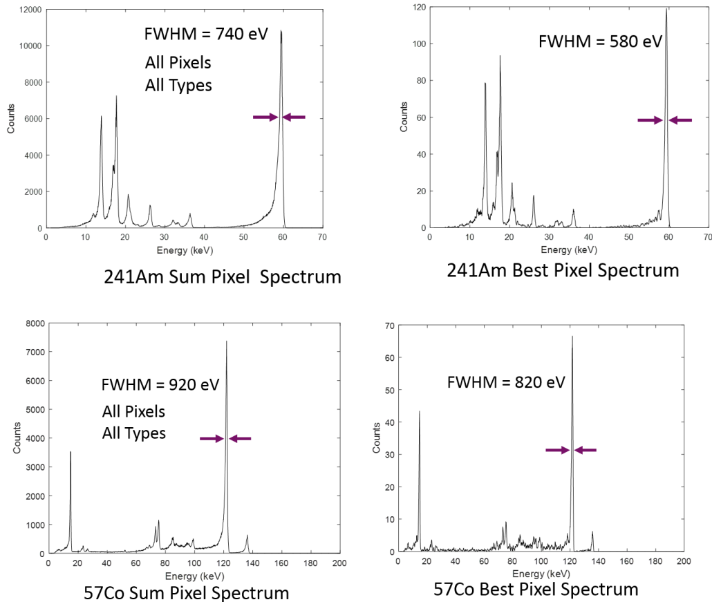
FIGURE 3.16 – Spectrum of ^{241}\text{Am} source (top) and ^{57}\text{Co} source (bot) performed at -6^\circ\text{C} . Left plots show the sum spectra with all types of interaction (meaning event with double events, triple or quadruple are considered) whereas right plots show the best spectrum with only one pixel and one event per trigger
