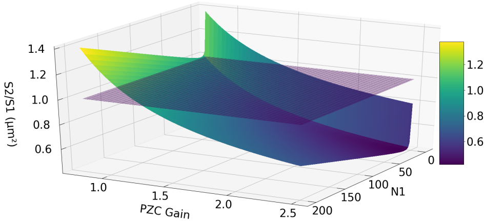
FIGURE 4.26 – Surface ratio between one stage PZC and two stages PZC. The plot shows that for a PZC gain larger than 1, the 2-stage solution is smaller.
