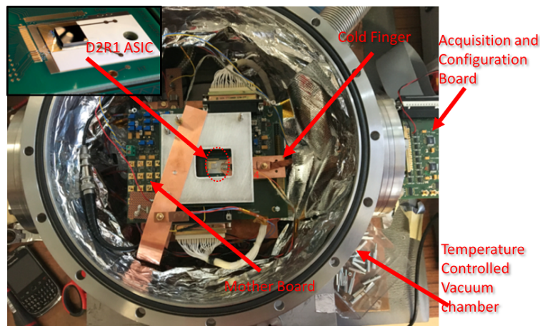
FIGURE 3.15 – Test bench for measurement of ASIC + Detector
