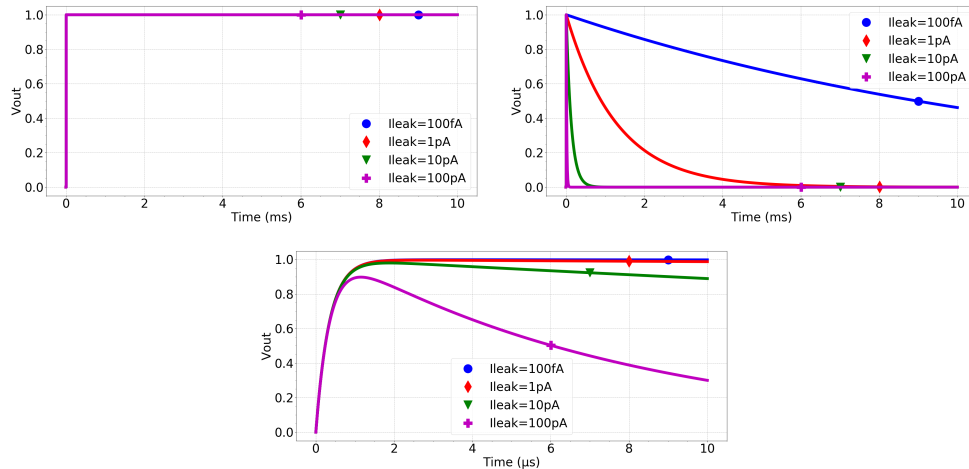
FIGURE 2.12 – Different CSA models. First is the ideal non reset CSA 2.5, second is ideal CSA with MOS reset 2.8. Third is the bandwidth limited CSA with MOS reset.
