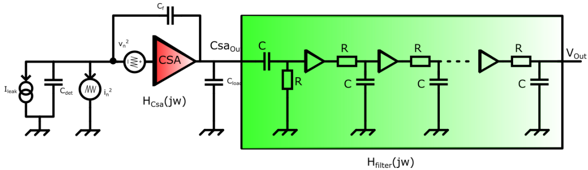
FIGURE 2.21 – CR – RC n Filter, ideal implementation: one CR filter followed by n RC filters.
