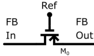
FIGURE 2.8 – Schematic of transistor acting like a resistor. It is biased using a fixed reference.
