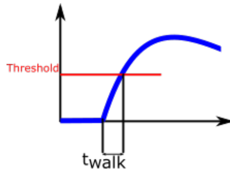
FIGURE 2.30 – Time walk description
