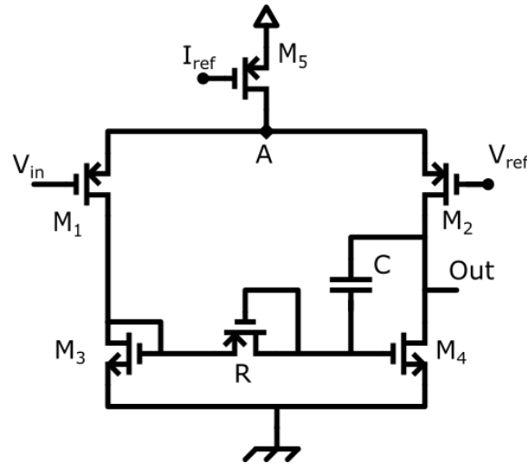
FIGURE 4.19 – NSNS schematic. High value resistor is made with an inverted diode connected MOS transistor. The equivalent resistor R is in the range of T\Omega .
