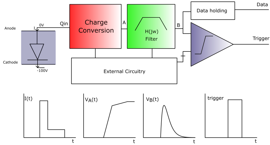
FIGURE 2.1 – Typical Charge detection chain schematic (top) and signals (bottom)
