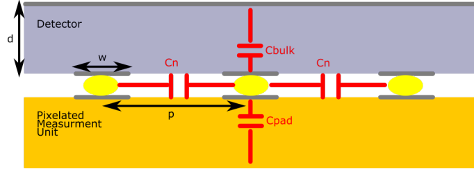
FIGURE 1.15 – Cross section view of capacitances in a pixelated detector
