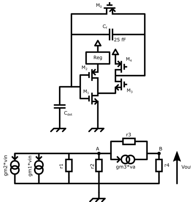
FIGURE B.1 – CMOS charge sensitive amplifier schematic (top) and small signal circuit (bot) The open loop gain of the amplifier is:
