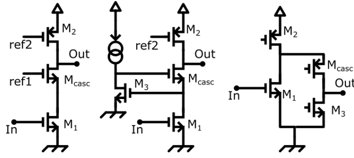
FIGURE 2.14 – Different amplifier architectures (telescopic cascode, regulated cascode, folded cascode)
