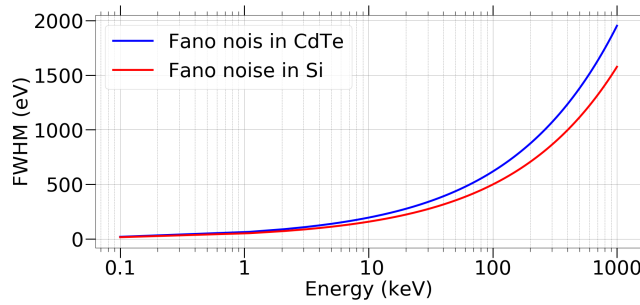
FIGURE 1.14 – Fano resolution versus Energy
