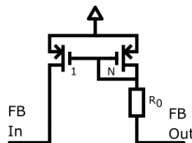
FIGURE 2.10 – Simplified schematic of Current Conveyor Reset
