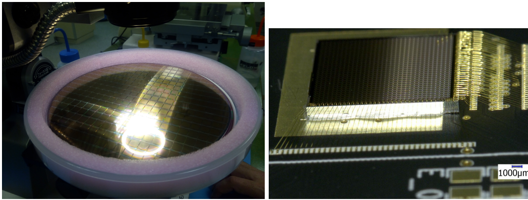
FIGURE 4.1 – Picture of the complete D^2R_2 wafer (left), and close up view of one chip bonded to its daughter board(right).
