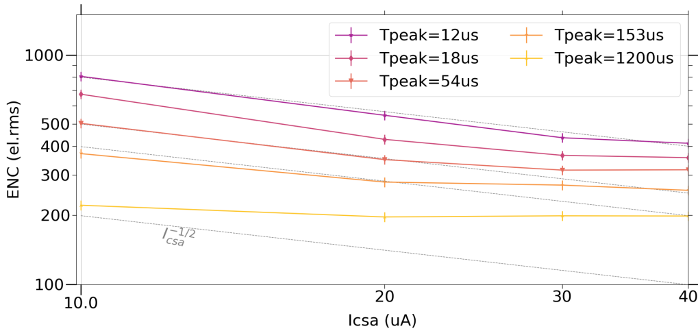
FIGURE 4.16 – ENC variation with leakage current for different peaking times with C_{det} = 1.5 pF
