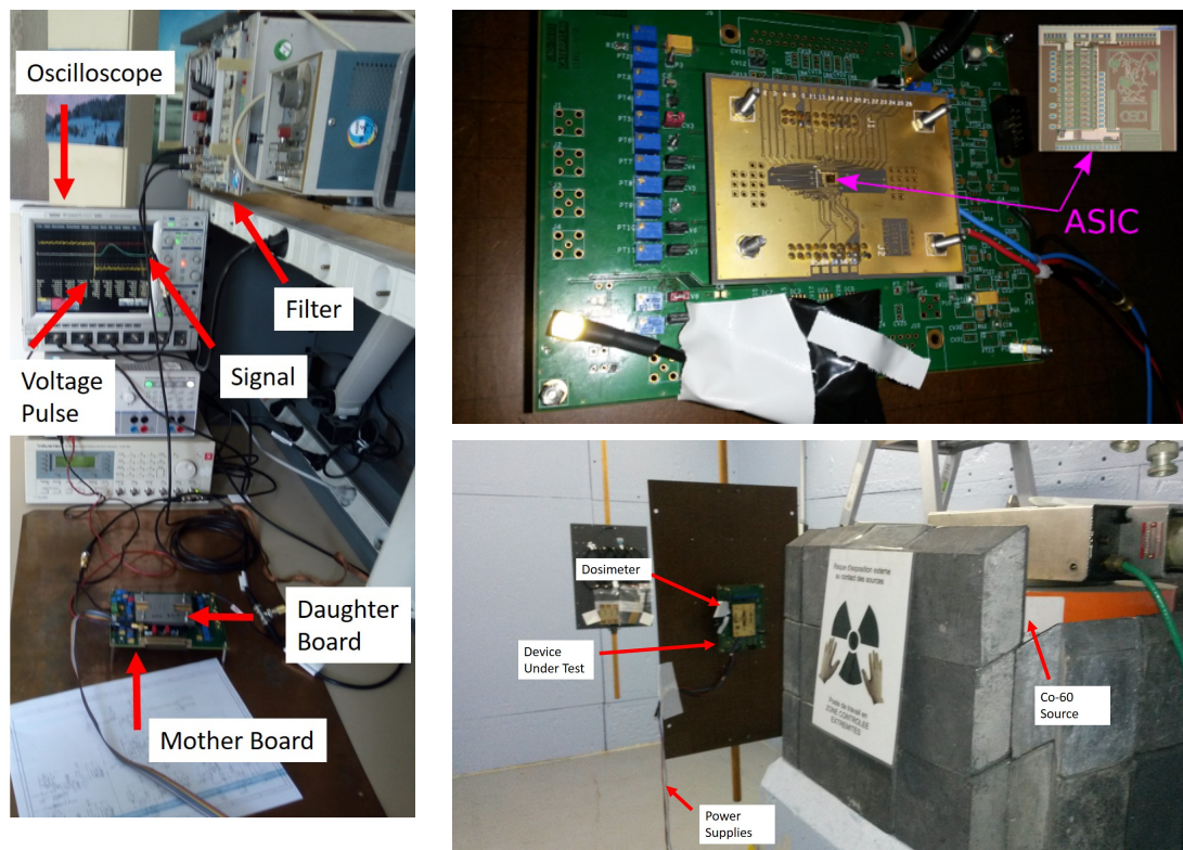
FIGURE 3.4 – Test setup for signal measurements(left) and irradiation setup (right)
