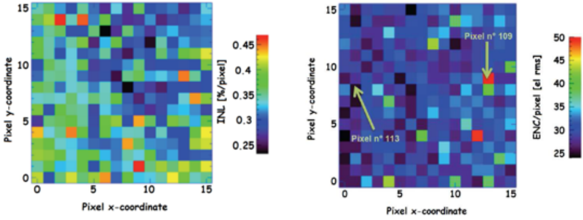
FIGURE 3.13 – Linearity map (left) and Equivalent Noise Charge Map(right) for charges from 1 fC to 6 fC
