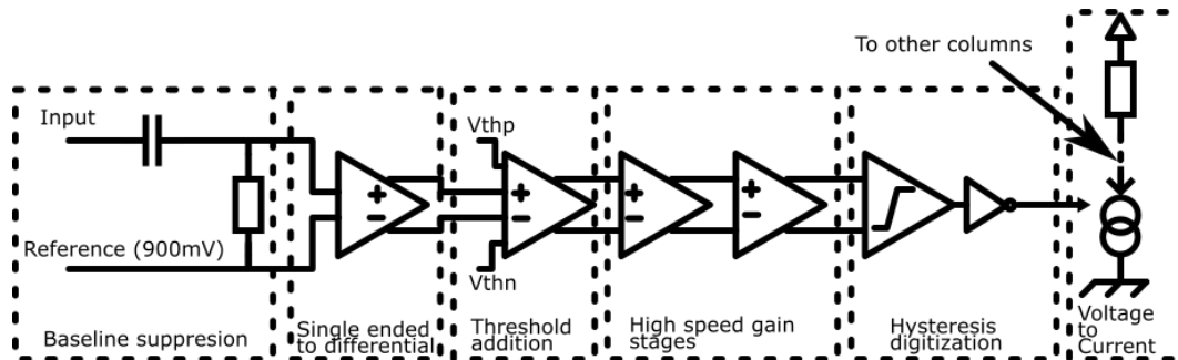
FIGURE 4.36 – D2R2 Discriminator schematic.
