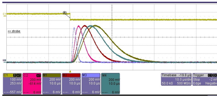
FIGURE 3.31 – Shaper signal at the output of the ASIC for varying peaking times (from 1\mu\text{s} to 11\mu\text{s} ). Yellow curve is the injection step voltage.
