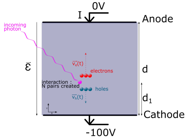
FIGURE 1.10 – Schematic of a one-pixel planar detector.
