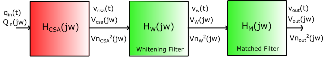
FIGURE 2.19 – Schematic of the matched filter theory, applied for radiation sensors application
