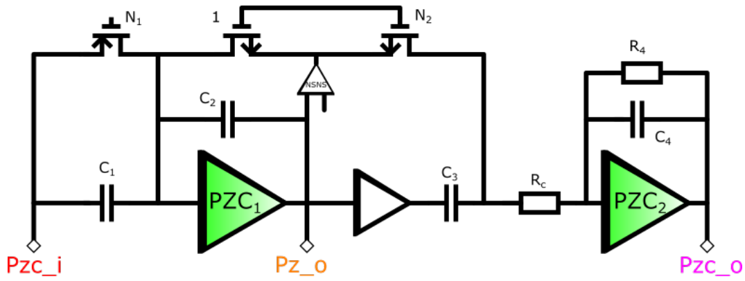
FIGURE 4.24 – Filtering stage schematic; The first two parts act as a pole zero cancellation circuit. The last amplifier acts as a low pass filter. A resistor R_c has been inserted between pole zero cancellation and lowpass filter to provide an additional pole.
