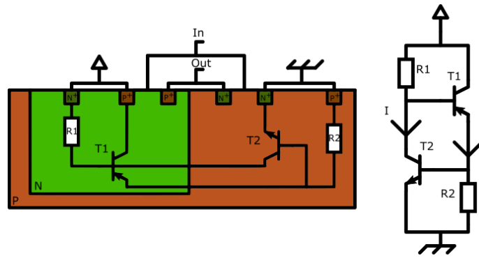
FIGURE 3.1 – Parasitic thyristor of an inverter. The I current is potentially destructive.
