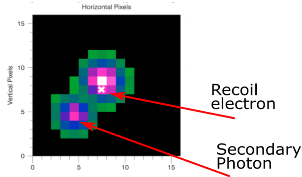
FIGURE 1.8 – Picture of Compton interaction occurring in pixelated gaseous detector Caliste MM [14]. Colours shows the amount of charge deposit (white is the higher charge, green the smaller).
