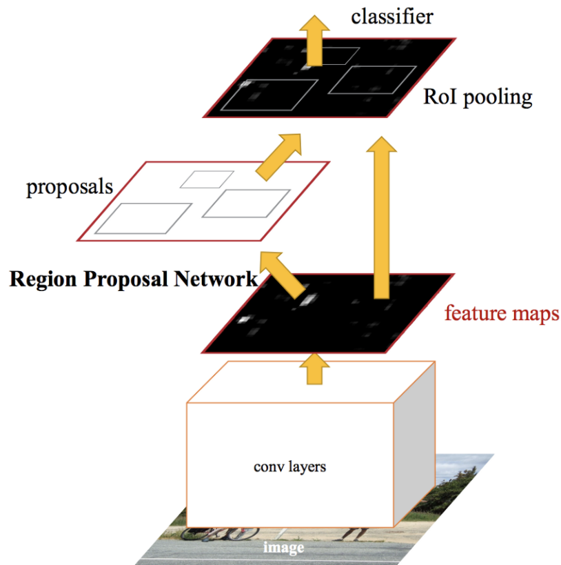
FIGURE 1.7 – Faster R-CNN
