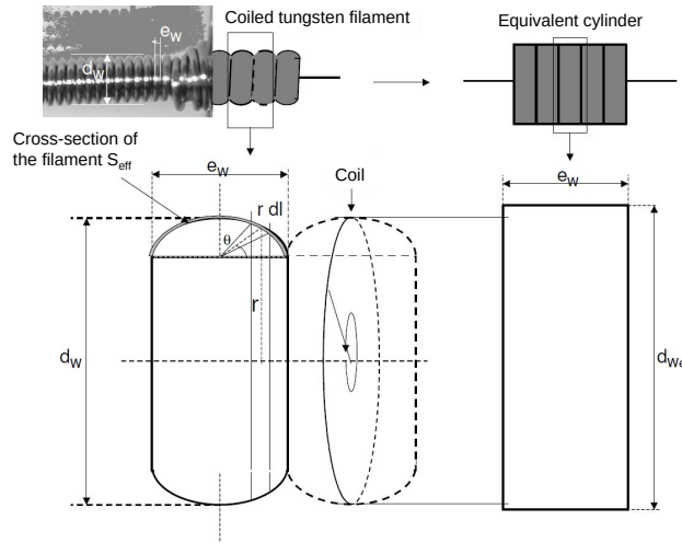
Figure 2.16 – Equivalent diameter of a coiled filament [Monteix2001]
