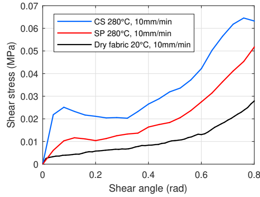
Figure 5.16 – Average shear stress versus shear angle curves for the preconsolidated (CS, blue) and semipreg (SP, red) specimens at 280 °C, and dry fabric at room temperature and 10 mm min -1 .
