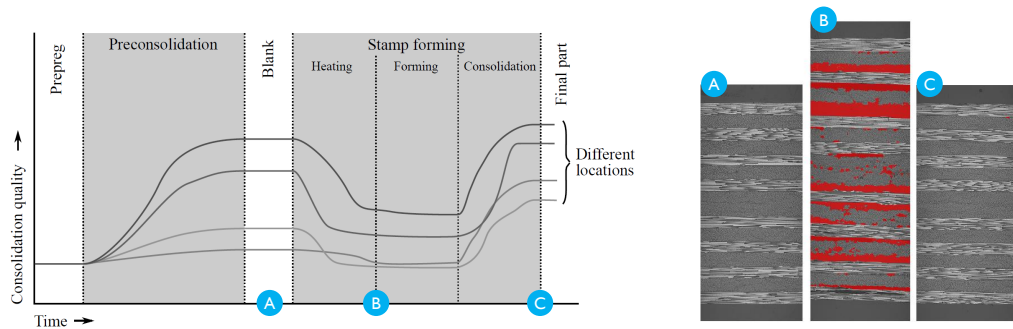
Figure 2.37 – Schematic representation of the evolution of consolidation quality during processing and micrographs of a unidirectional carbon/PEEK laminate after press forming consolidation, infrared heating and stamp forming (voids in red) [Slange+2016]
