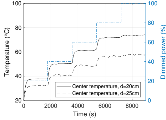
Figure 3.5 – Evolution of temperature at the center of the backface with varying lamp input power
