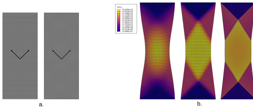
Figure 6.15 – a. Mesh aligned with sample principal directions (left) and yarn directions (right), b. Resulting shear angle field after 30 mm extension (l. to r.: M3D4 and M3D4R aligned with sample, M3D4R aligned with yarns)
