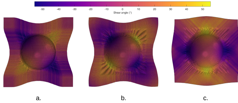
Figure 6.19 – Shear angle field, a. In-plane shear neglected ( G_{12} = 0 ), b. T = 300\text{ °C}/0^\circ , c. T = 300\text{ °C}/45^\circ
