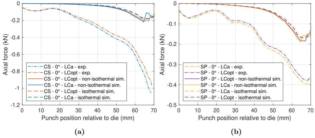
Figure 6.28 – Comparison between experimental axial force and prediction from isothermal and non-isothermal simulations. a. preconsolidated, b. semipreg
