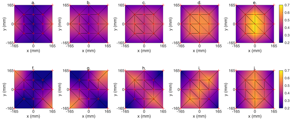
Figure 4.22 – Sensitivity of the temperature field to the lamp power. Left-to-right: lamp pairs P1 to P5, top: LCa, bottom: LCb
