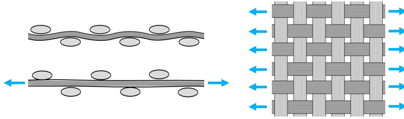
Figure 2.19 – Decrimping during uniaxial tension (plain weave)
