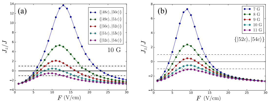
FIGURE II.5 On the left we show the J_z/J ratio for \{|nc\rangle, |(n+2)c\rangle\} pairs. The plot is done for B = 10 G and as a function of the electric field F . Atoms are 5 \mu\text{m} apart. Note that for n = 52 the ratio is always negative. On the right we show, as an illustration of the flexibility provided by the magnetic field, that by reducing the magnetic field, the J_z/J \rightarrow -1, 1 tunability with F is regained for n = 52 .
