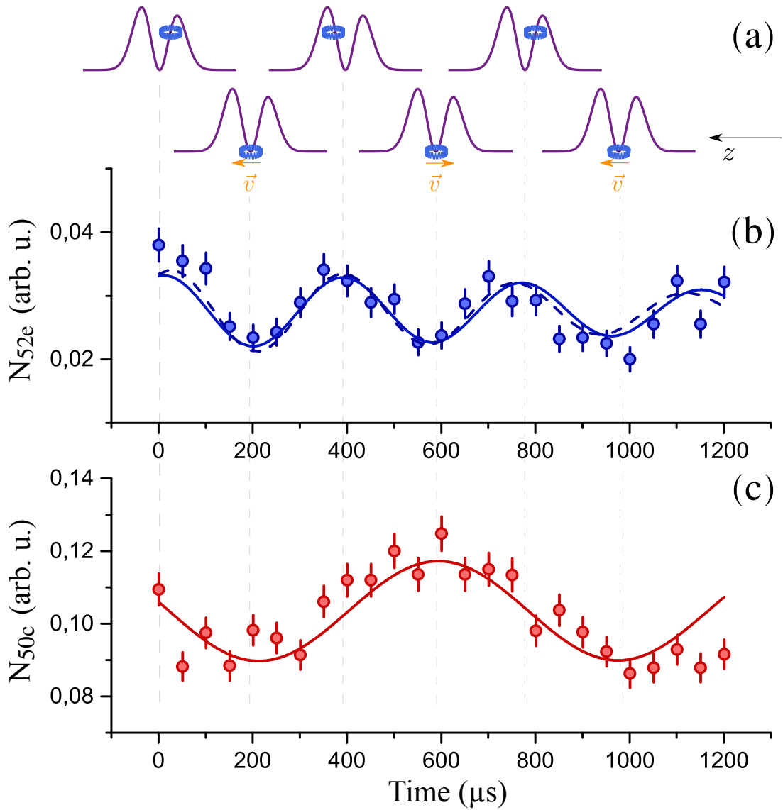
FIGURE V.19 Trap frequency measurement. (a) The top sketch shows a cRy atom oscillating in the LG trap. (b) Number of atoms, number of |52e^- atoms detected. (c) Number of atoms, number of |50c\rangle atoms detected. The lines are damped sinusoidal fits to the data.
