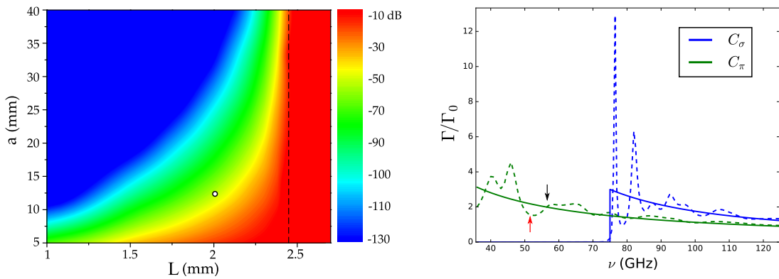
FIGURE II.11 On the left we plot the CST calculation for the inhibition of the real capacitor. On the right we plot the power ratio as a function of frequency for both dipole orientations for the chosen capacitor geometry. The full lines correspond to the ideal capacitor and the dashed lines correspond to the CST calculation. The dominant transition frequencies are marked with arrows. The black arrow corresponds to the frequency of the n = 48, \pi \uparrow (57.69 GHz) transition and the red arrow corresponds to the frequency of the n = 50, \pi \uparrow (51.099 GHz) transition.
