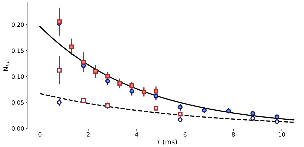
FIGURE V.15 Total population of |50c\rangle before the \text{MW}_P probe pulse for trapped (blue circles) and untrapped (red rectangles) atoms. The line is an exponential fit. Full symbols correspond to an average atom number \bar{N} . Open symbols correspond to measurements with about \bar{N}/2 atoms.
