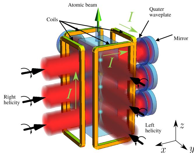
FIGURE III.2 Drawing of the 2D-MOT. The (bi-dimensional) cold atoms are shown in cyan.
