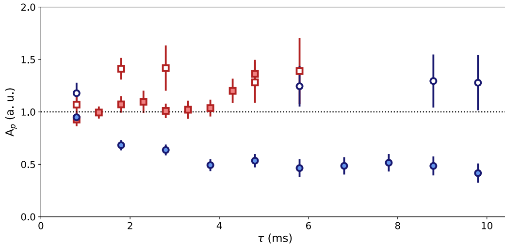
FIGURE V.16 Integrated area A_p of the MW_P probe spectrum for trapped (blue) and untrapped (red) atoms. Full symbols correspond to the measurements in Figures V.14 and V.15, for an average atom number \bar{N} . Open symbols correspond to measurements with about \bar{N}/2 atoms.
