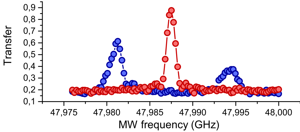
FIGURE III.18 Autler-Townes splitting and recombination. The \sigma^- RF field splits energies of the |\pm\rangle states (blue dots). Tuning the electrodes phases to turn the polarization of the field into \sigma^+ recombines the peaks into one single line (red dots).
