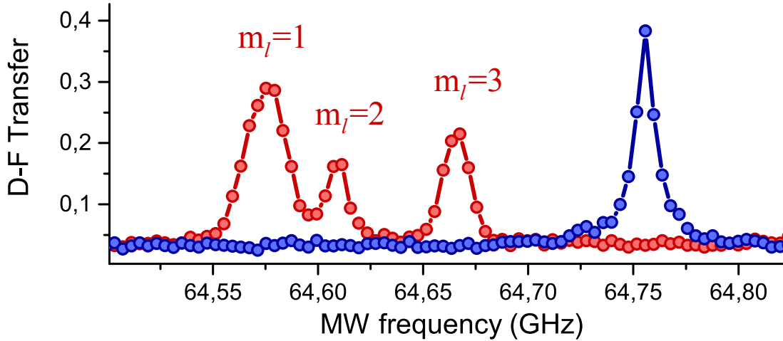
FIGURE III.12 MW spectroscopy from |52D_{5/2}\rangle . In blue, the three 52F lines collapsed into one at zero electric field. Excitation is done from the laser accessible level |52D_{5/2}, m_j = 5/2\rangle . At an electric field of \sim 0.67 V/cm we see that the three lines are resolved (red).
