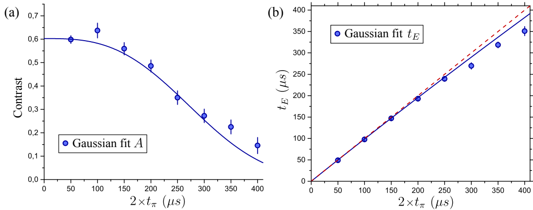
FIGURE IV.16 In (a), we plot the Gaussian amplitude A (dots) as a function of 2 \times t_\pi . Physically, A represents the contrast of the oscillation at time t_E . Note that the measured t_E is smaller than 2 \times t_\pi (b).
