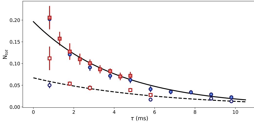
FIGURE V.15 Total population of |50c\rangle before the MW_P probe pulse for trapped (blue circles) and untrapped (red rectangles) atoms. The line is an exponential fit. Full symbols correspond to an average atom number \bar{N} . Open symbols correspond to measurements with about \bar{N}/2 atoms.
