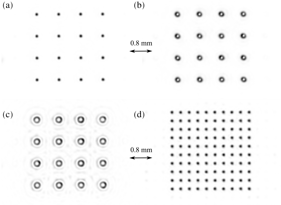
FIGURE CONC.2 Two-dimensional 4 \times 4 arrays of Gaussians (a), LG_{01} (b), and Bob traps (c). In (d), we show an array of 10 \times 10 Gaussian beams which are optimized to an intensity spread of 0.6% intensity.
