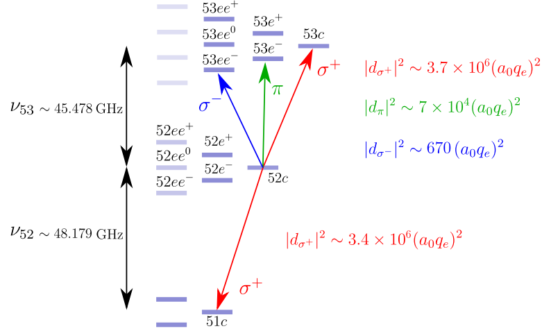
FIGURE II.6 Main transitions responsible for the decay of level 52c . Note that |d_{\sigma+}| \gg |d_{\pi}| \gg |d_{\sigma-}| . The ordering is in general true for all cRy levels n and it is a consequence of the scaling laws.
