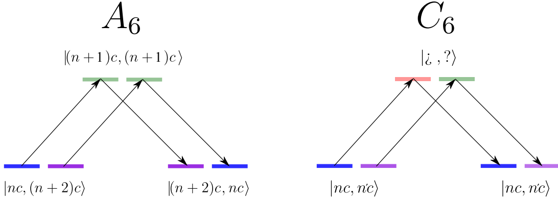
FIGURE II.4 We show a graphical interpretation of the physical processes giving rise to the van der Waals interaction eq.(II.3) between cRy atoms. The state labeled with question marks represent anyone of the many states contributing to the process.
