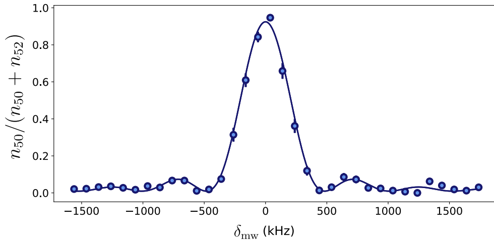
FIGURE III.24 Microwave spectroscopy of the two-photon |52c\rangle to |50c\rangle ( \text{MW}_S ) transition. The frequency offset is 99.2786 GHz.
