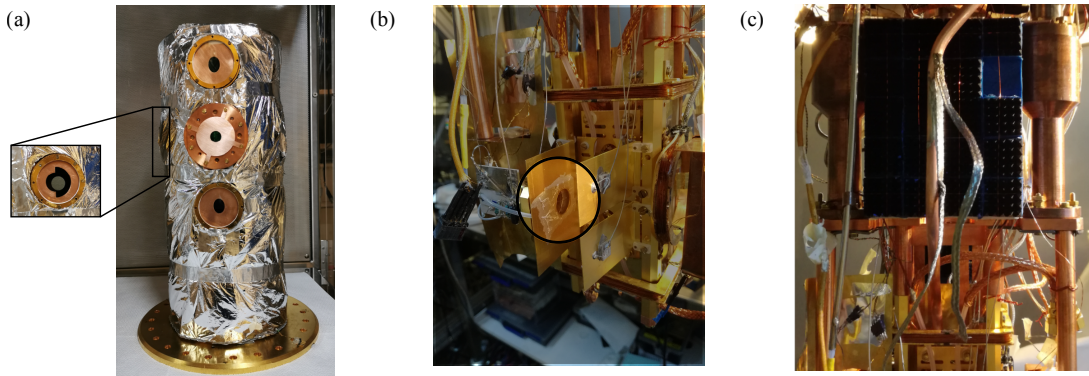
FIGURE IV.1 In (a), the Helium screen is shown where the copper irises are installed. In (b), the hole in the shield electrode covered with the thin mesh is show. In (c), we show a photograph of the MW absorber installation.
