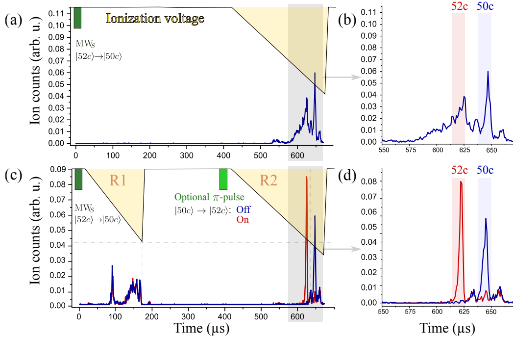
FIGURE V.11 The partial ionization technique. The ionization voltage is shown by the yellow shaded area. In the upper panel, we show the ionization-signal corresponding to the preparation of |50c\rangle state (a) and a zoom to the interesting area (b) for a high number of Rydberg atoms. The lower panel (c) shows the action of the partial ionization with (red) and without the action of a \pi pulse from |50c\rangle \rightarrow |52c\rangle . A zoom to the interesting area is shown in (d).
