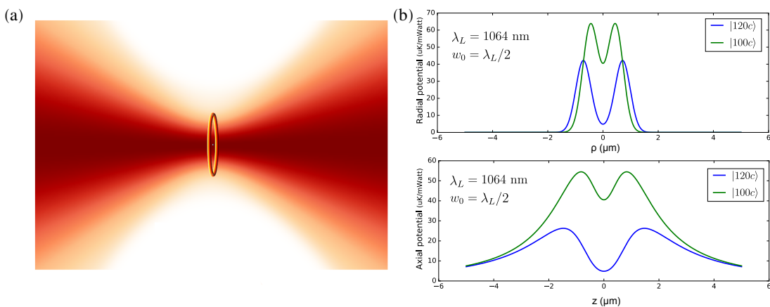
FIGURE CONC.3 A Rydberg belt for a light waist. (a) The trapping scheme. For large enough circular orbits, the trap is confining the atom in 3D. Otherwise the beam is a 2D radial trap and an anti-trap in the axial direction. In (b), we show the ponderomotive energy landscape for two large n circular atoms.
