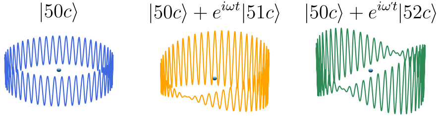
FIGURE I.1 Here we represent the cRy electron as a matter-wave. A cRy has a symmetric distribution of charge around the nucleus and presents no permanent dipole. A superposition of |nc\rangle and |(n + 1)c\rangle creates an asymmetric electron density, which gives rise to a rotating dipole. A superposition of |nc\rangle and |(n + 2)c\rangle regains reflection symmetry. There is no permanent dipole.
