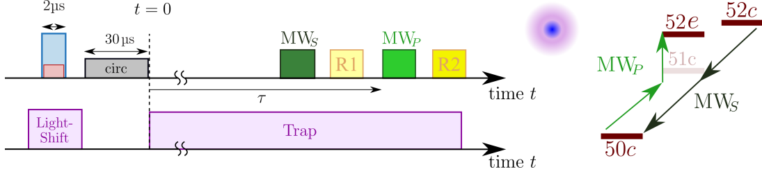
FIGURE V.12 Left: Timing of the experiment (not to scale). In the top timeline, from left to right, we have the laser excitation (blue/red), circular state preparation (grey), selection pulse MW_S (dark green), partial ionization (light yellow), probe pulse MW_P (light green), and field ionization (dark yellow). In the lower timeline, the trapping laser timing is shown. Right: Partial diagram of the Stark levels in the n = 50 and n = 52 manifolds. The arrows represent the microwave transitions MW_S (level selection) and MW_P (probe). The two-photon transition is done with two MW photons of equal frequency despite the length difference of the arrows in the drawing.
