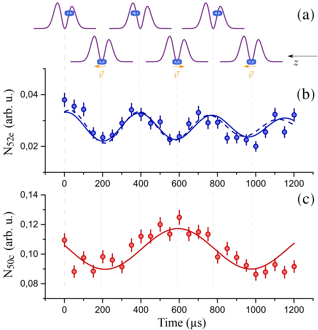
FIGURE V.19 Trap frequency measurement. (a) The top sketch shows a cRy atom oscillating in the LG trap. (b) Number of atoms, number of |52e^- atoms detected. (c) Number of atoms, number of |50c atoms detected. The lines are damped sinusoidal fits to the data.
