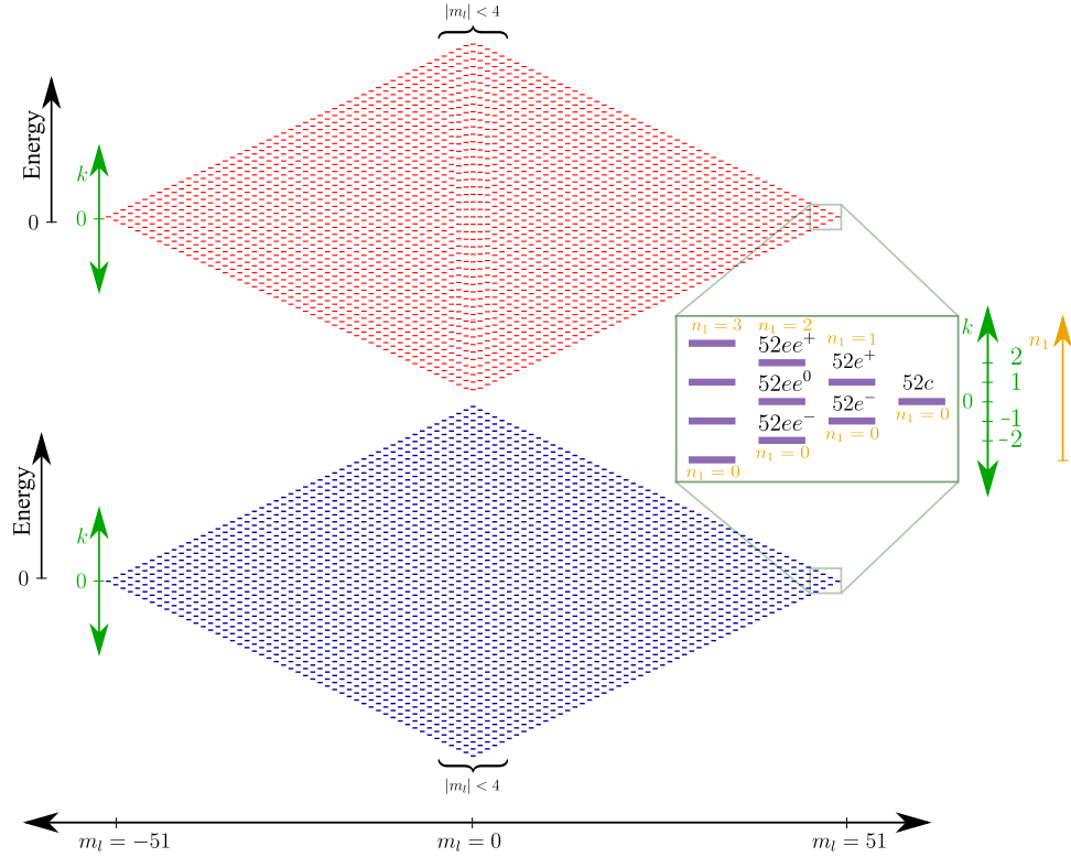
FIGURE I.2 The Stark diamond for Rubidium-87 (red) showing the quantum defects under the influence of an electric field (for B_z = 0 G and F_z > 2 V/cm) and that for the Coulomb potential (blue).
